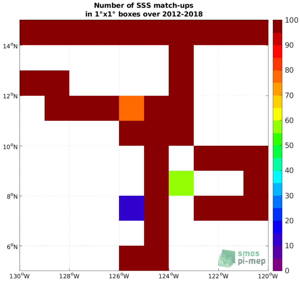
Figure 4: Number of SSS match-ups between TSG (SAMOS) SSS and the SMAP SSS L4 OI v1 - 7 Days (IPRC) SSS product for the SPURS 2 Pi-MEP region over 1°×1° boxes and for the full satellite product period.
