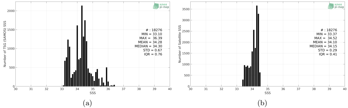
Figure 2: Histograms of SSS from TSG (SAMOS) (a) and SMAP SSS L4 OI v1 - 7 Days (IPRC) (b) considering all match-up pairs per bins of 0.1 over the SPURS 2 Pi-MEP region and for the full satellite product period.
