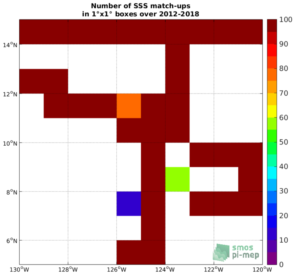
Figure 4: Number of SSS match-ups between TSG (SAMOS) SSS and the SMAP SSS L4 OI v1 - 7 Days (IPRC) SSS product for the SPURS 2 Pi-MEP region over 1^\circ \times 1^\circ boxes and for the full satellite product period.
