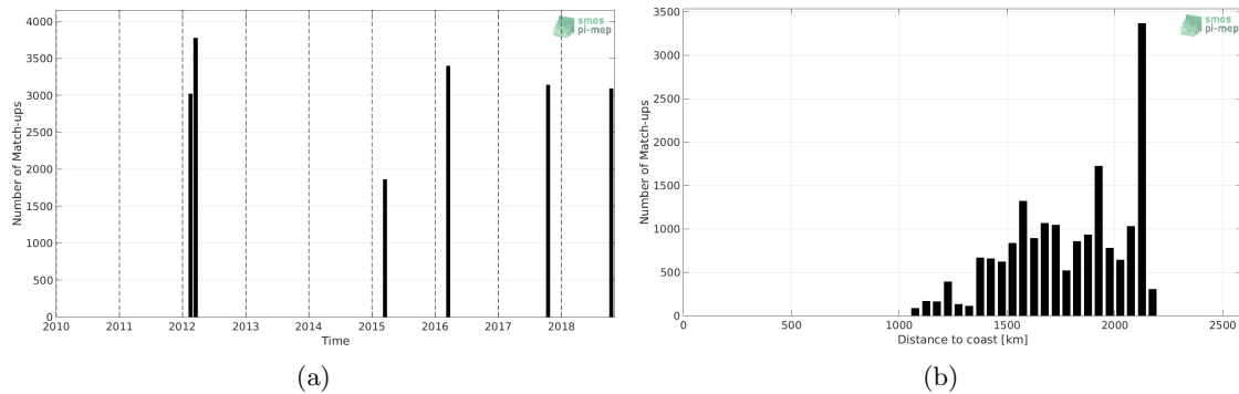
Figure 1: Number of match-ups between TSG (SAMOS) and SMAP SSS L4 OI v1 - 7 Days (IPRC) SSS as a function of time (a) and as function of the distance to coast (b) over the SPURS 2 Pi-MEP region and for the full satellite product period.
