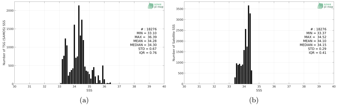
Figure 2: Histograms of SSS from TSG (SAMOS) (a) and SMAP SSS L4 OI v1 - 7day (IPRC) (b) considering all match-up pairs per bins of 0.1 over the SPURS 2 Pi-MEP region and for the full satellite product period.
