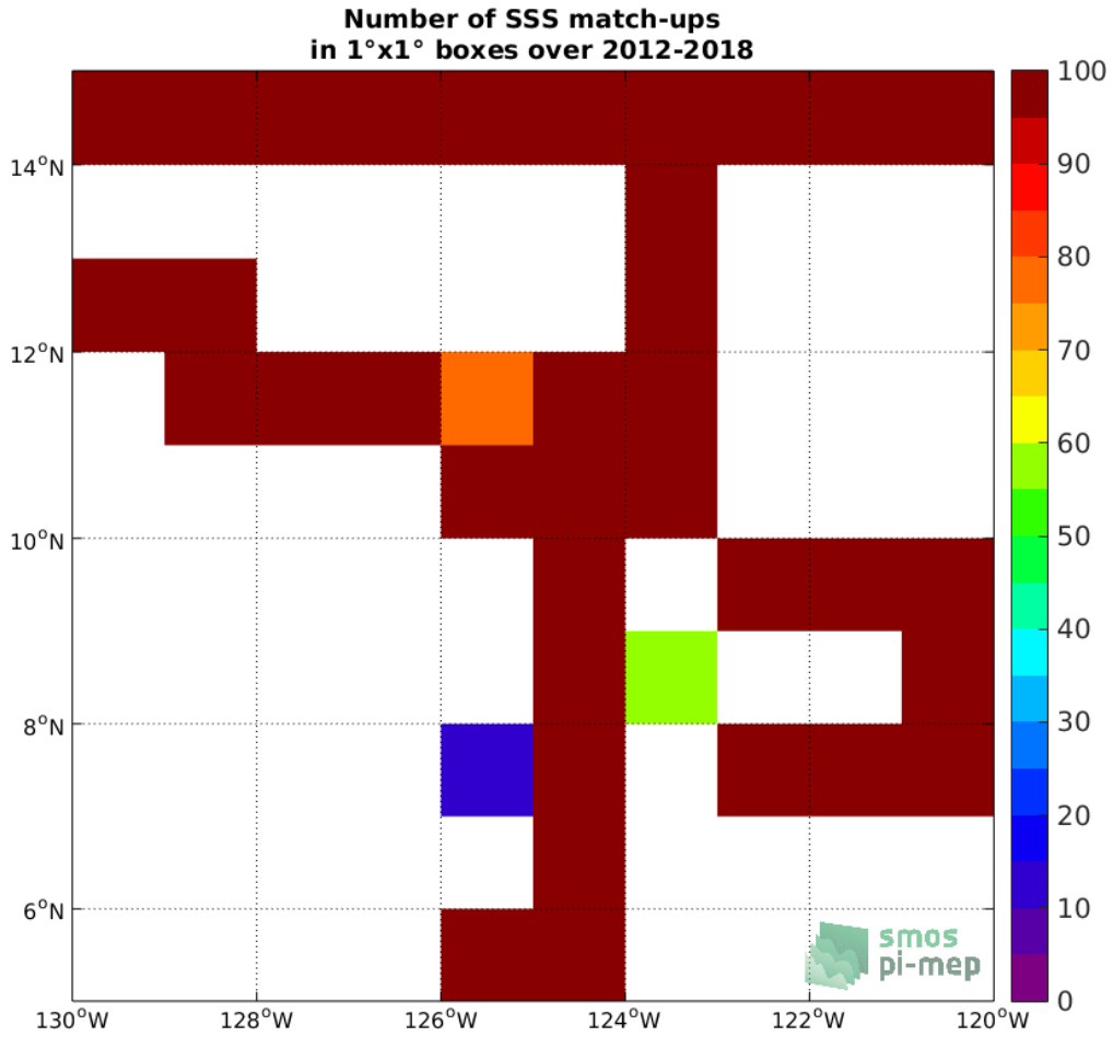
Figure 4: Number of SSS match-ups between TSG (SAMOS) SSS and the SMAP SSS L4 OI v1 - 7day (IPRC) SSS product for the SPURS 2 Pi-MEP region over 1°x1° boxes and for the full satellite product period.
