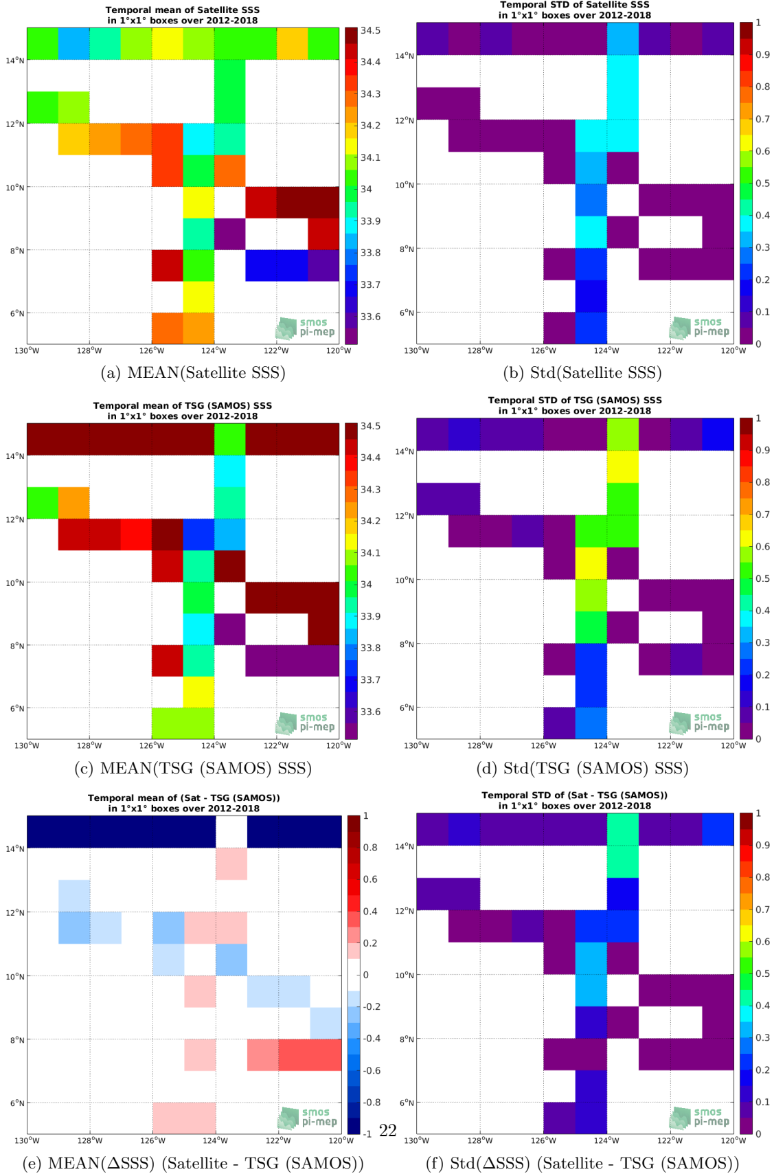
Figure 6: Temporal mean (left) and Std (right) of SSS from SMAP SSS L4 OI v1 - 7day (IPRC) (top), TSG (SAMOS) (middle), and of \Delta SSS (Satellite - TSG (SAMOS)). Only match-up pairs are used to generate these maps.
