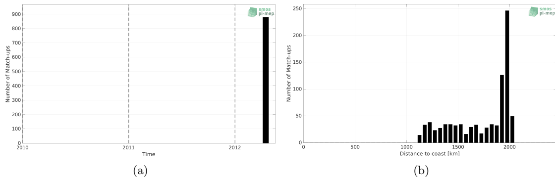
Figure 1: Number of match-ups between TSG (GOSUD-Research-vessel) and SMAP SSS L4 OI v1 - 7 Days (IPRC) SSS as a function of time (a) and as function of the distance to coast (b) over the SPURS 2 Pi-MEP region and for the full satellite product period.
