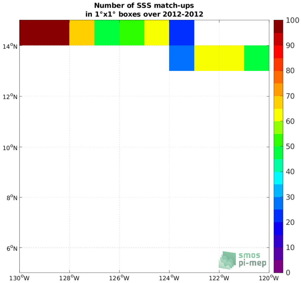
Figure 4: Number of SSS match-ups between TSG (GOSUD-Research-vessel) SSS and the SMAP SSS L4 OI v1 - 7 Days (IPRC) SSS product for the SPURS 2 Pi-MEP region over 1^\circ \times 1^\circ boxes and for the full satellite product period.
