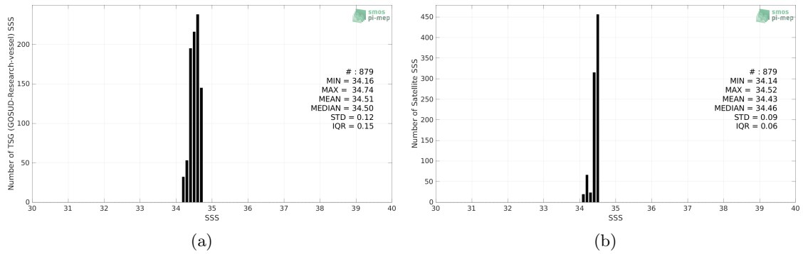
Figure 2: Histograms of SSS from TSG (GOSUD-Research-vessel) (a) and SMAP SSS L4 OI v1 - 7 Days (IPRC) (b) considering all match-up pairs per bins of 0.1 over the SPURS 2 Pi-MEP region and for the full satellite product period.
