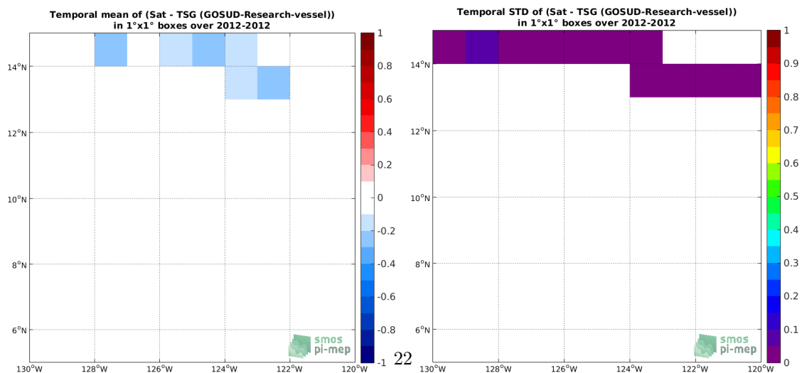
Figure 6: Temporal mean (left) and Std (right) of SSS from SMAP SSS L4 OI v1 - 7day (IPRC) (top), TSG (GOSUD-Research-vessel) (middle), and of \Delta SSS (Satellite - TSG (GOSUD-Research-vessel)). Only match-up pairs are used to generate these maps.
