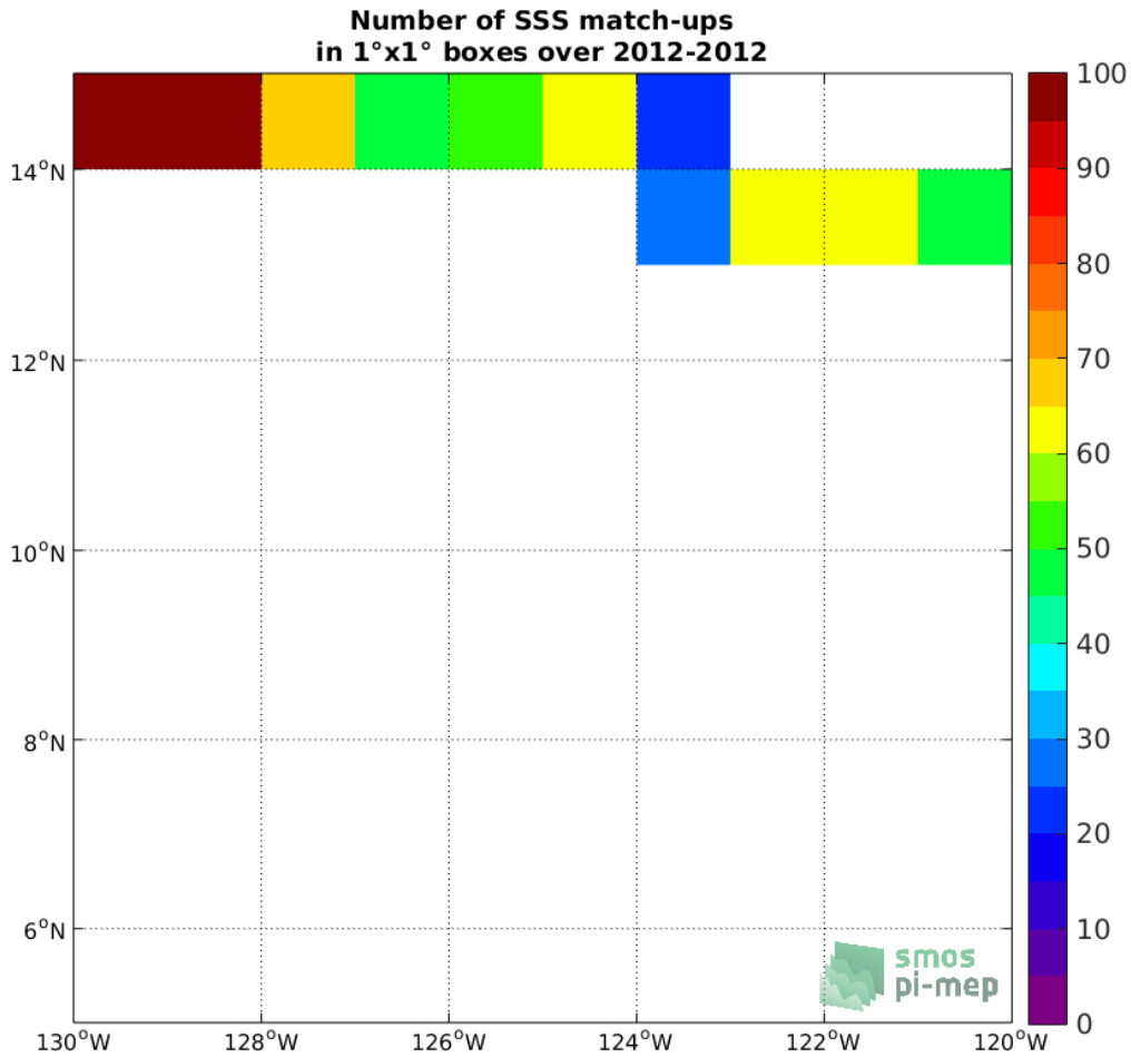
Figure 4: Number of SSS match-ups between TSG (GOSUD-Research-vessel) SSS and the SMAP SSS L4 OI v1 - 7day (IPRC) SSS product for the SPURS 2 Pi-MEP region over 1°x1° boxes and for the full satellite product period.
