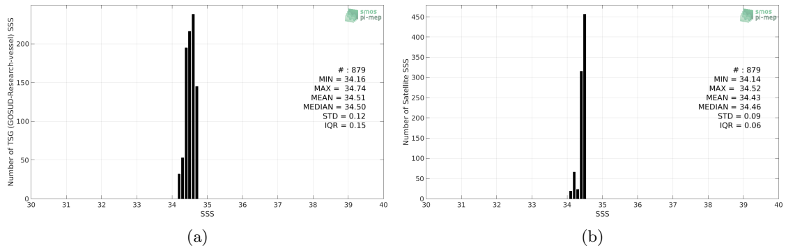
Figure 2: Histograms of SSS from TSG (GOSUD-Research-vessel) (a) and SMAP SSS L4 OI v1 - 7day (IPRC) (b) considering all match-up pairs per bins of 0.1 over the SPURS 2 Pi-MEP region and for the full satellite product period.
