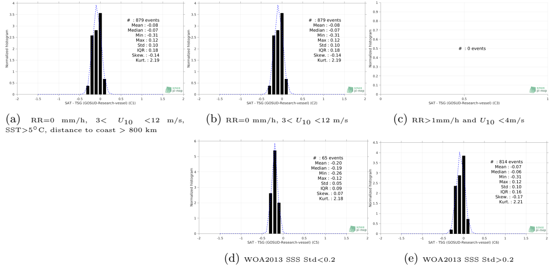
Figure 13: Normalized histogram of \Delta SSS (SMAP SSS L4 OI v1 - 7day (IPRC) - TSG (GOSUD-Research-vessel)) for 5 different subdatasets corresponding to: RR=0 mm/h, 3 < U_{10} < 12 m/s, SST > 5°C, distance to coast > 800 km (a), RR=0 mm/h, 3 < U_{10} < 12 m/s (b), RR > 1mm/h and U_{10} < 4 m/s (c), WOA2013 SSS Std < 0.2 (d), WOA2013 SSS Std > 0.2 (e).
