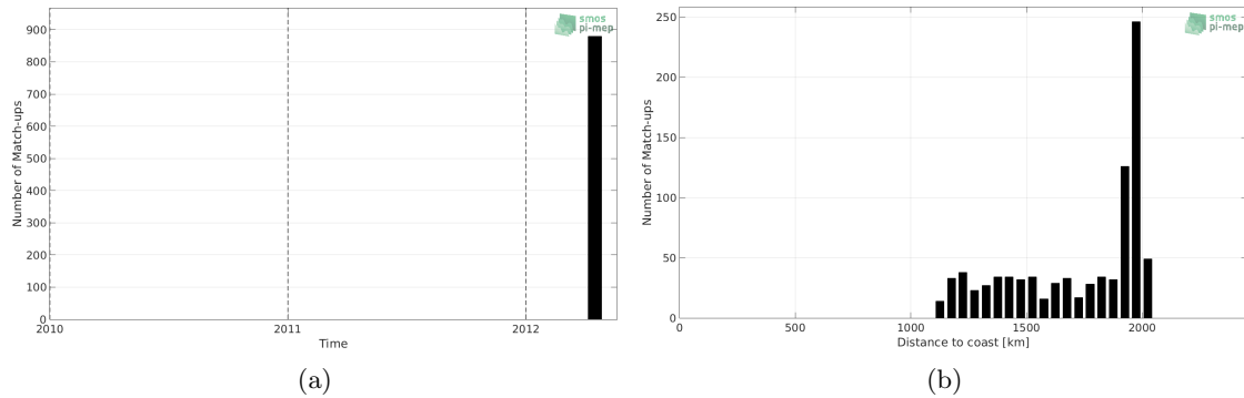
Figure 1: Number of match-ups between TSG (GOSUD-Research-vessel) and SMAP SSS L4 OI v1 - 7day (IPRC) SSS as a function of time (a) and as function of the distance to coast (b) over the SPURS 2 Pi-MEP region and for the full satellite product period.
