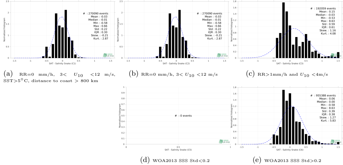
Figure 12: Normalized histogram of \Delta SSS (SMAP SSS L4 OI v1 - 7 Days (IPRC) - Salinity Snake) for 5 different subdatasets corresponding to: RR=0 mm/h, 3 < U_{10} < 12 m/s, SST > 5°C, distance to coast > 800 km (a), RR=0 mm/h, 3 < U_{10} < 12 m/s (b), RR > 1mm/h and U_{10} < 4 m/s (c), WOA2013 SSS Std < 0.2 (d), WOA2013 SSS Std > 0.2 (e).
