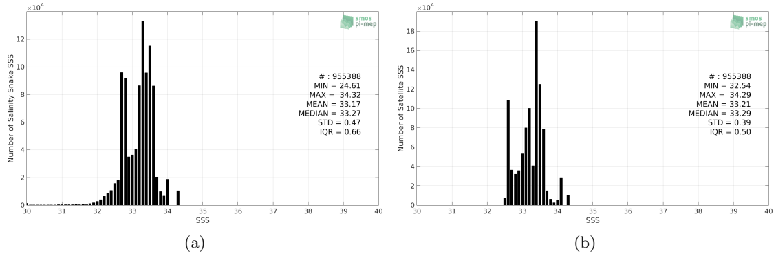
Figure 2: Histograms of SSS from Salinity Snake (a) and SMAP SSS L4 OI v1 - 7 Days (IPRC) (b) considering all match-up pairs per bins of 0.1 over the SPURS 2 Pi-MEP region and for the full satellite product period.
