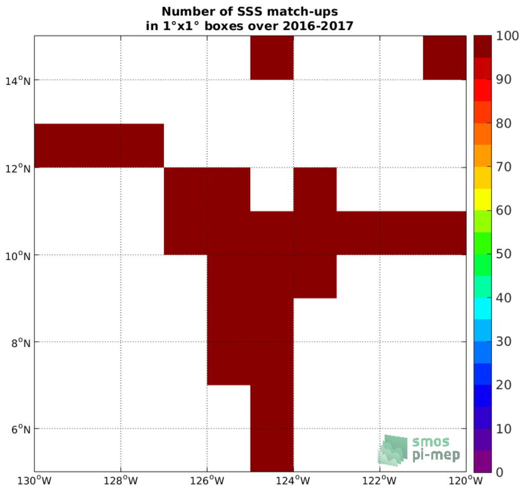
Figure 3: Number of SSS match-ups between Salinity Snake SSS and the SMAP SSS L4 OI v1 - 7 Days (IPRC) SSS product for the SPURS 2 Pi-MEP region over 1^\circ \times 1^\circ boxes and for the full satellite product period.
