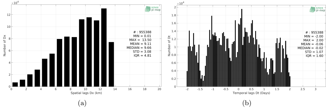
Figure 4: Histograms of the spatial (a) and temporal (b) lags between the location/time of the Salinity Snake measurement and the date of the corresponding SMAP SSS L4 OI v1 - 7 Days (IPRC) SSS pixel.
