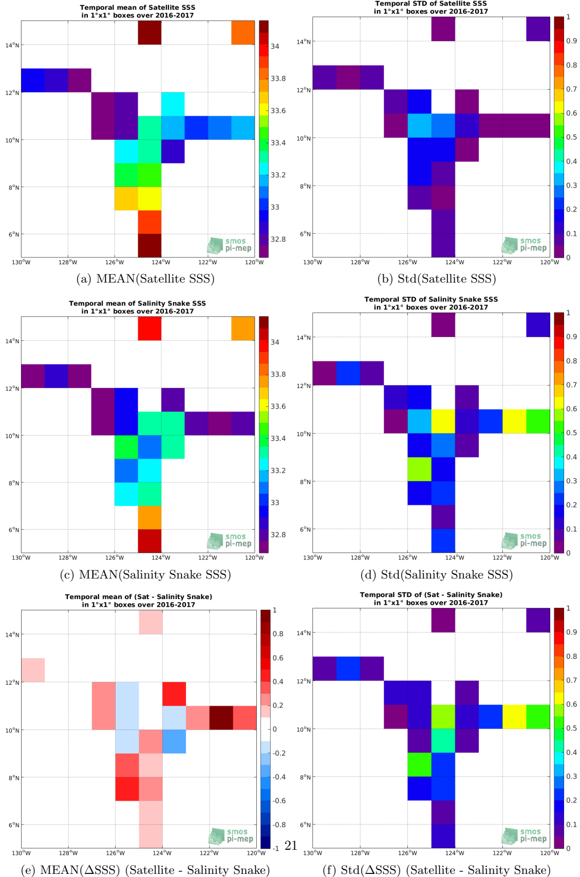
Figure 5: Temporal mean (left) and Std (right) of SSS from SMAP SSS L4 OI v1 - 7 Days (IPRC) (top), Salinity Snake (middle), and of \Delta SSS (Satellite - Salinity Snake). Only match-up pairs are used to generate these maps.
