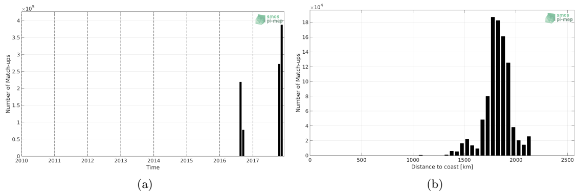
Figure 1: Number of match-ups between Salinity Snake and SMAP SSS L4 OI v1 - 7 Days (IPRC) SSS as a function of time (a) and as function of the distance to coast (b) over the SPURS 2 Pi-MEP region and for the full satellite product period.
