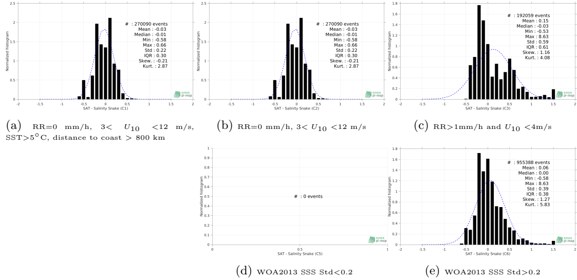
Figure 12: Normalized histogram of \Delta SSS (SMAP SSS L4 OI v1 - 7 Days (IPRC) - Salinity Snake) for 5 different subdatasets corresponding to: RR=0 mm/h, 3 < U_{10} < 12 m/s, SST>5°C, distance to coast > 800 km (a), RR=0 mm/h, 3 < U_{10} < 12 m/s (b), RR>1mm/h and U_{10} < 4 m/s (c), WOA2013 SSS Std<0.2 (d), WOA2013 SSS Std>0.2 (e).
