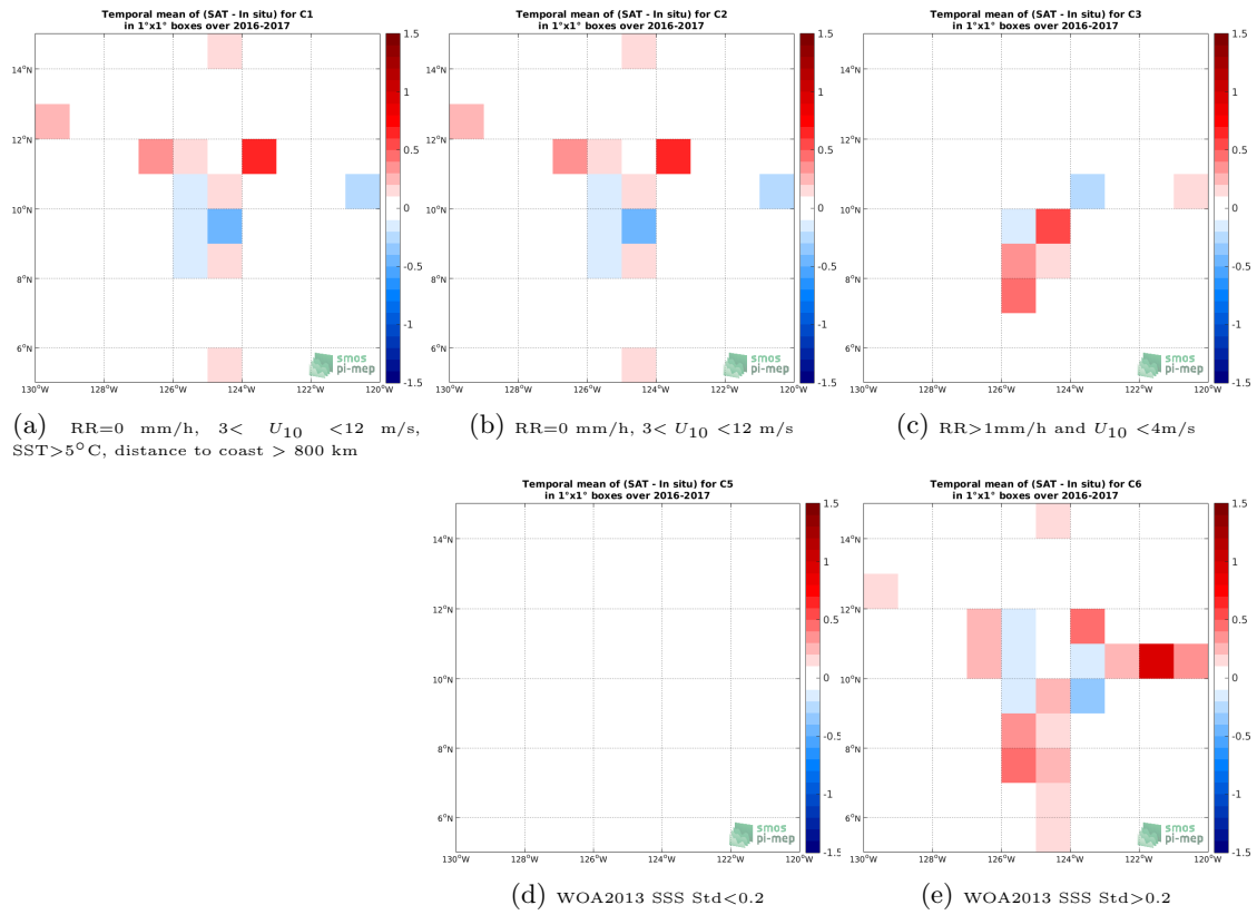
Figure 11: Temporal mean gridded over spatial boxes of size 1^\circ \times 1^\circ of \Delta\text{SSS} (SMAP SSS L4 OI v1 - 7 Days (IPRC) - Salinity Snake) for 5 different subdatasets corresponding to: RR=0 mm/h, 3 < U_{10} < 12 m/s, SST > 5^\circ\text{C} , distance to coast > 800 km (a), RR=0 mm/h, 3 < U_{10} < 12 m/s (b), RR > 1 mm/h and U_{10} < 4 m/s (c), WOA2013 SSS Std < 0.2 (d), WOA2013 SSS Std > 0.2 (e).
