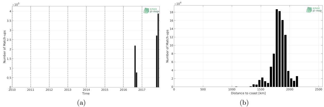
Figure 1: Number of match-ups between Salinity Snake and SMAP SSS L4 OI v1 - 7day (IPRC) SSS as a function of time (a) and as function of the distance to coast (b) over the SPURS 2 Pi-MEP region and for the full satellite product period.
