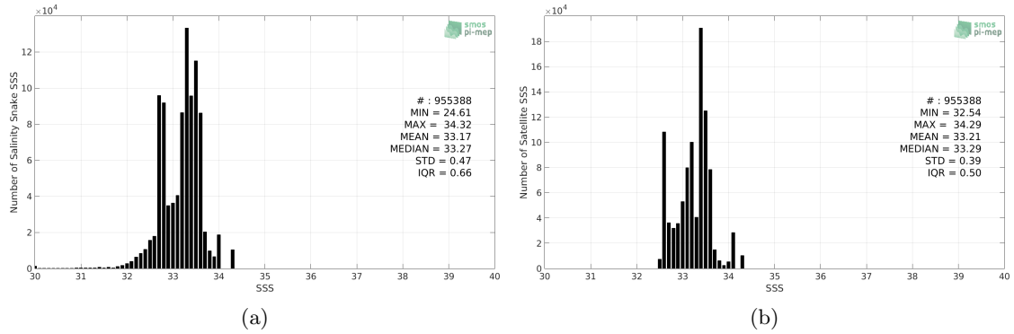
Figure 2: Histograms of SSS from Salinity Snake (a) and SMAP SSS L4 OI v1 - 7day (IPRC) (b) considering all match-up pairs per bins of 0.1 over the SPURS 2 Pi-MEP region and for the full satellite product period.
