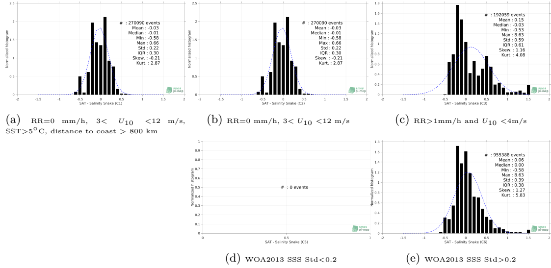
Figure 12: Normalized histogram of \Delta SSS (SMAP SSS L4 OI v1 - 7day (IPRC) - Salinity Snake) for 5 different subdatasets corresponding to: RR=0 mm/h, 3 < U_{10} < 12 m/s, SST > 5°C, distance to coast > 800 km (a), RR=0 mm/h, 3 < U_{10} < 12 m/s (b), RR > 1mm/h and U_{10} < 4 m/s (c), WOA2013 SSS Std < 0.2 (d), WOA2013 SSS Std > 0.2 (e).
