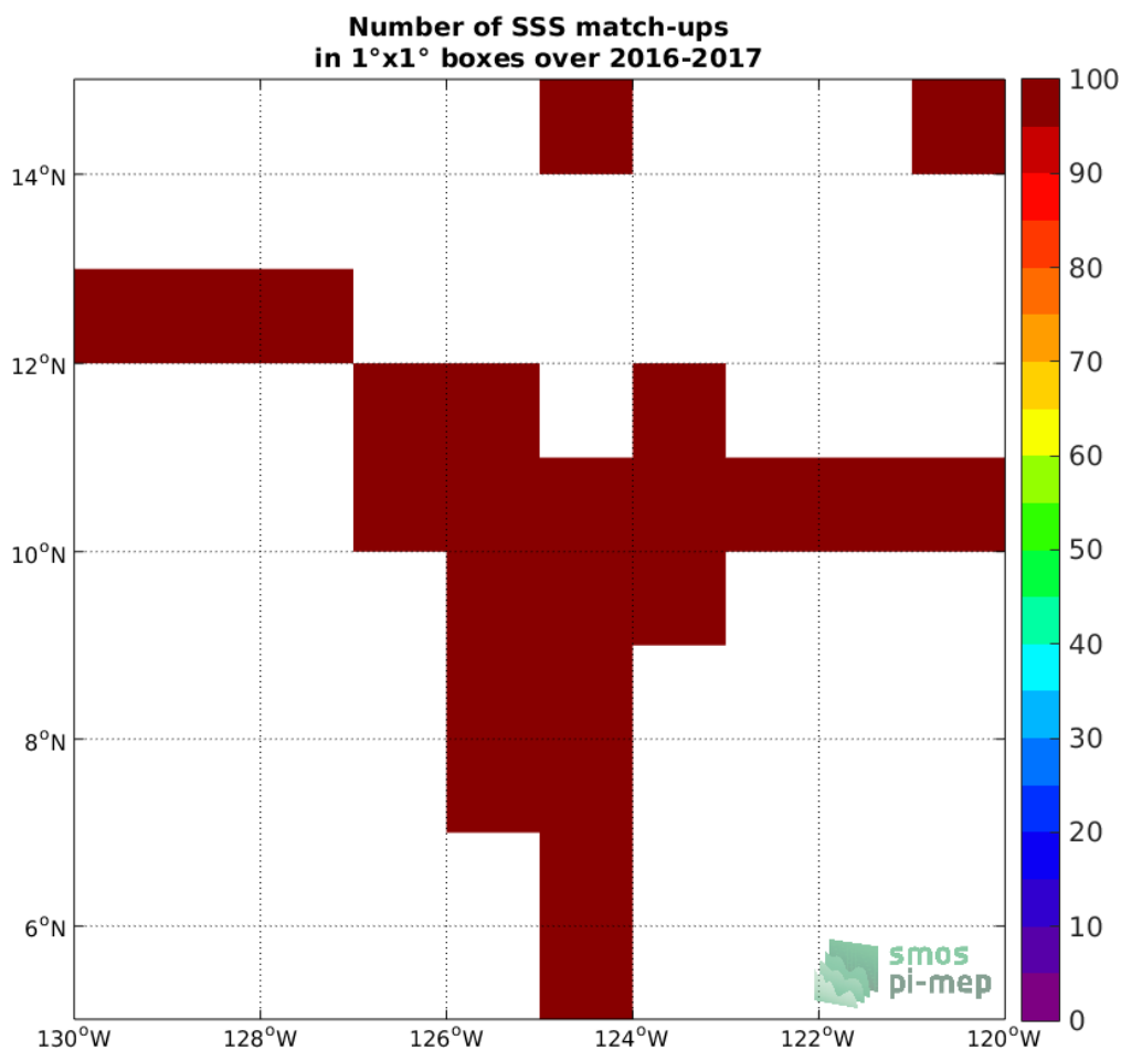
Figure 3: Number of SSS match-ups between Salinity Snake SSS and the SMAP SSS L4 OI v1 - 7day (IPRC) SSS product for the SPURS 2 Pi-MEP region over 1°x1° boxes and for the full satellite product period.
