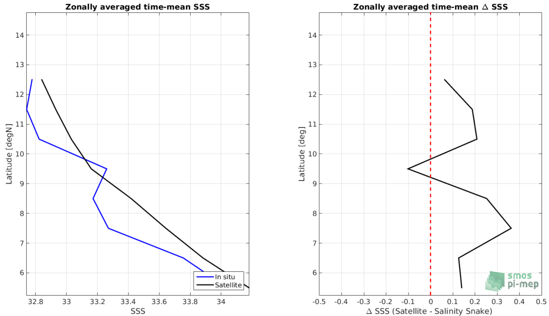
Figure 7: Left panel: Zonal mean SSS from SMAP SSS L4 OI v1 - 7day (IPRC) satellite product (black) and from Salinity Snake (blue). Right panel: Zonal mean of \Delta SSS (Satellite - Salinity Snake) for all the collected Pi-MEP match-up pairs estimated over the full satellite product period.
