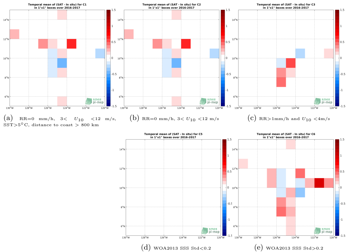
Figure 11: Temporal mean gridded over spatial boxes of size 1^\circ \times 1^\circ of \Delta SSS (SMAP SSS L4 OI v1 - 7day (IPRC) - Salinity Snake) for 5 different subdatasets corresponding to:RR=0 mm/h, 3 < U_{10} < 12 m/s, SST >5^\circ\text{C} , distance to coast > 800 km (a), RR=0 mm/h, 3 < U_{10} < 12 m/s (b), RR >1 mm/h and U_{10} < 4 m/s (c), WOA2013 SSS Std <0.2 (d), WOA2013 SSS Std >0.2 (e).
