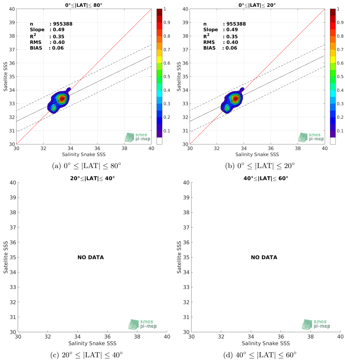
Figure 8: Contour maps of the concentration of SMAP SSS L4 OI v1 - 7day (IPRC) SSS (y-axis) versus Salinity Snake SSS (x-axis) at match-up pairs for different latitude bands. For each plot, the red line shows x=y . The black thin and dashed lines indicate a linear fit through the data cloud and the \pm 95\% confidence levels, respectively. The number match-up pairs n , the slope and R^2 coefficient of the linear fit, the root mean square (RMS) and the mean bias between satellite and in situ data are indicated for each latitude band in each plots.
