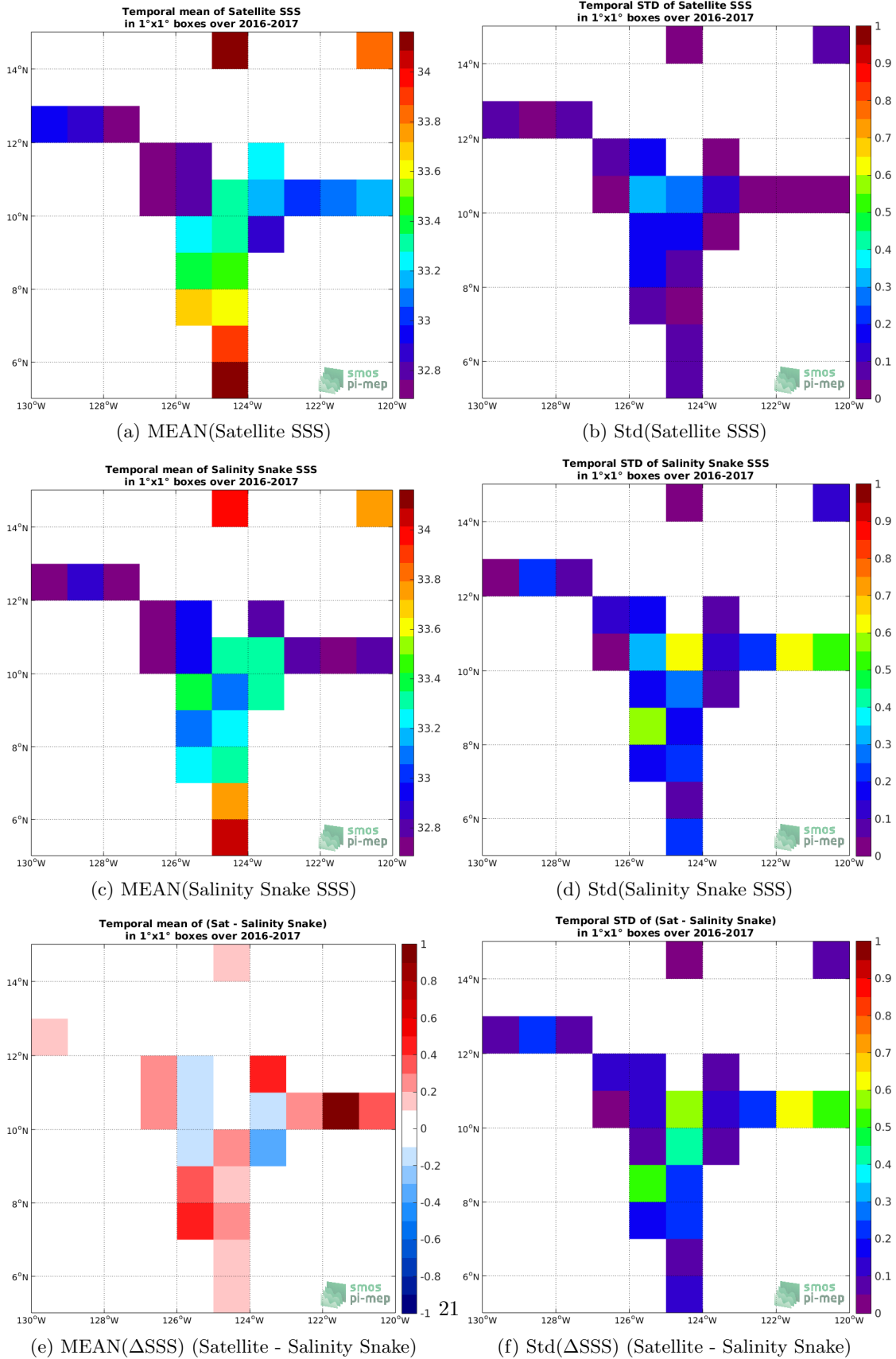
Figure 5: Temporal mean (left) and Std (right) of SSS from SMAP SSS L4 OI v1 - 7day (IPRC) (top), Salinity Snake (middle), and of \Delta SSS (Satellite - Salinity Snake). Only match-up pairs are used to generate these maps.
