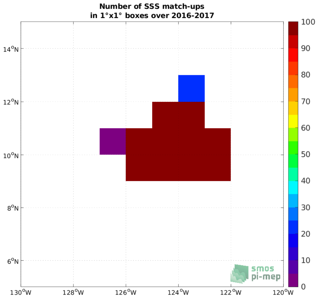
Figure 3: Number of SSS match-ups between Seaglider SSS and the SMAP SSS L4 OI v1 - 7 Days (IPRC) SSS product for the SPURS 2 Pi-MEP region over 1°x1° boxes and for the full satellite product period.
