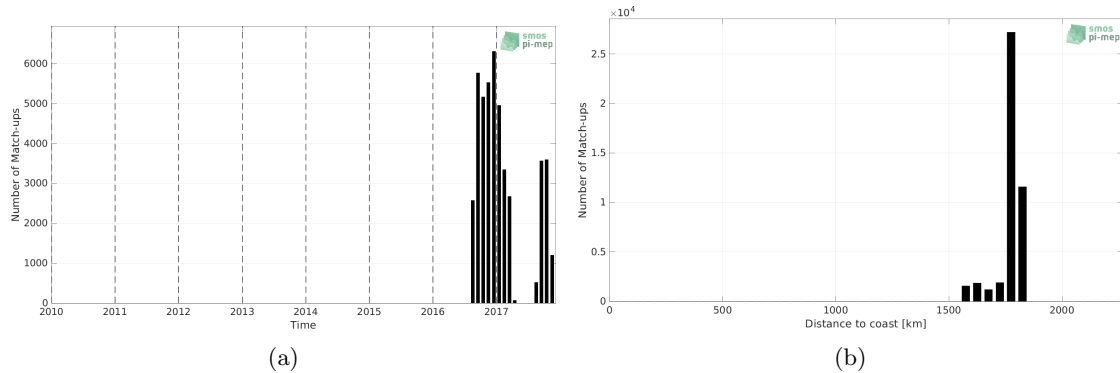
Figure 1: Number of match-ups between Seaglider and SMAP SSS L4 OI v1 - 7 Days (IPRC) SSS as a function of time (a) and as function of the distance to coast (b) over the SPURS 2 Pi-MEP region and for the full satellite product period.
