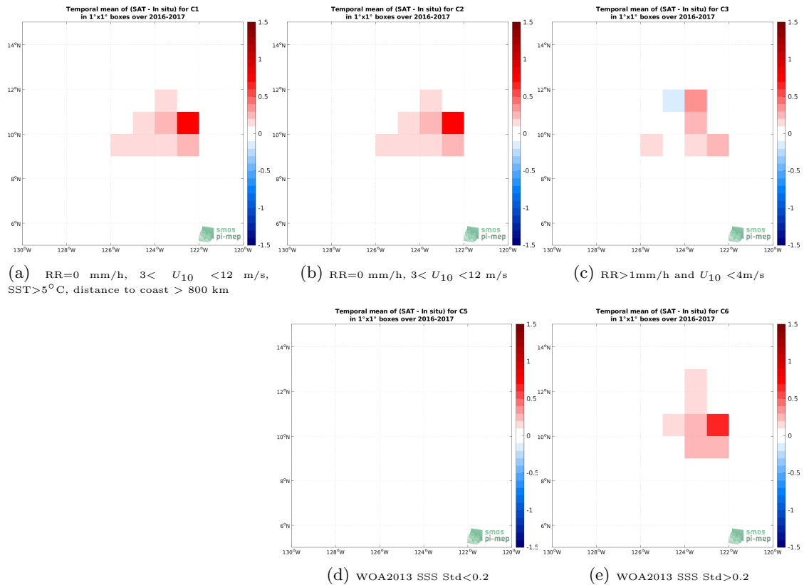
Figure 11: Temporal mean gridded over spatial boxes of size 1^\circ \times 1^\circ of \Delta SSS (SMAP SSS L4 OI v1 - 7 Days (IPRC) - Seaglider) for 5 different subdatasets corresponding to:RR=0 mm/h, 3 < U_{10} < 12 m/s, SST > 5°C, distance to coast > 800 km (a), RR=0 mm/h, 3 < U_{10} < 12 m/s (b), RR > 1mm/h and U_{10} < 4 m/s (c), WOA2013 SSS Std < 0.2 (d), WOA2013 SSS Std > 0.2 (e).
