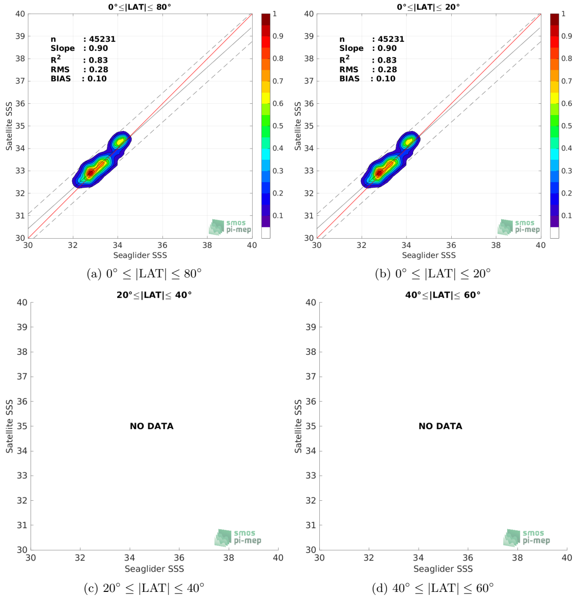
Figure 8: Contour maps of the concentration of SMAP SSS L4 OI v1 - 7 Days (IPRC) SSS (y-axis) versus Seaglider SSS (x-axis) at match-up pairs for different latitude bands. For each plot, the red line shows x=y . The black thin and dashed lines indicate a linear fit through the data cloud and the \pm 95\% confidence levels, respectively. The number match-up pairs n , the slope and R^2 coefficient of the linear fit, the root mean square (RMS) and the mean bias between satellite and in situ data are indicated for each latitude band in each plots.
