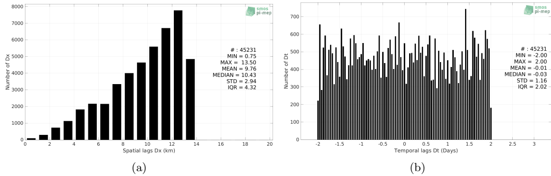
Figure 4: Histograms of the spatial (a) and temporal (b) lags between the location/time of the Seaglider measurement and the date of the corresponding SMAP SSS L4 OI v1 - 7 Days (IPRC) SSS pixel.
