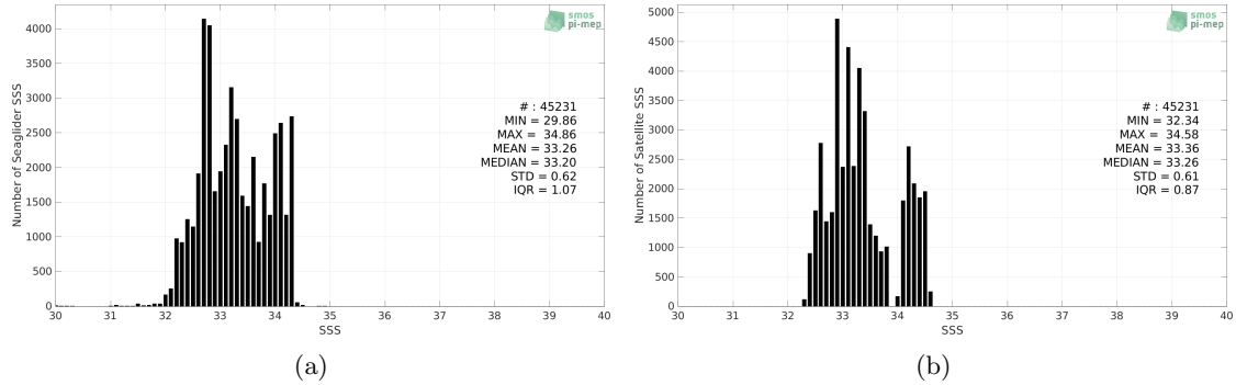
Figure 2: Histograms of SSS from Seagliders (a) and SMAP SSS L4 OI v1 - 7 Days (IPRC) (b) considering all match-up pairs per bins of 0.1 over the SPURS 2 Pi-MEP region and for the full satellite product period.
