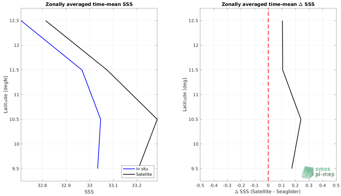
Figure 7: Left panel: Zonal mean SSS from SMAP SSS L4 OI v1 - 7 Days (IPRC) satellite product (black) and from Seaglider (blue). Right panel: Zonal mean of \Delta SSS (Satellite - Seaglider) for all the collected Pi-MEP match-up pairs estimated over the full satellite product period.
