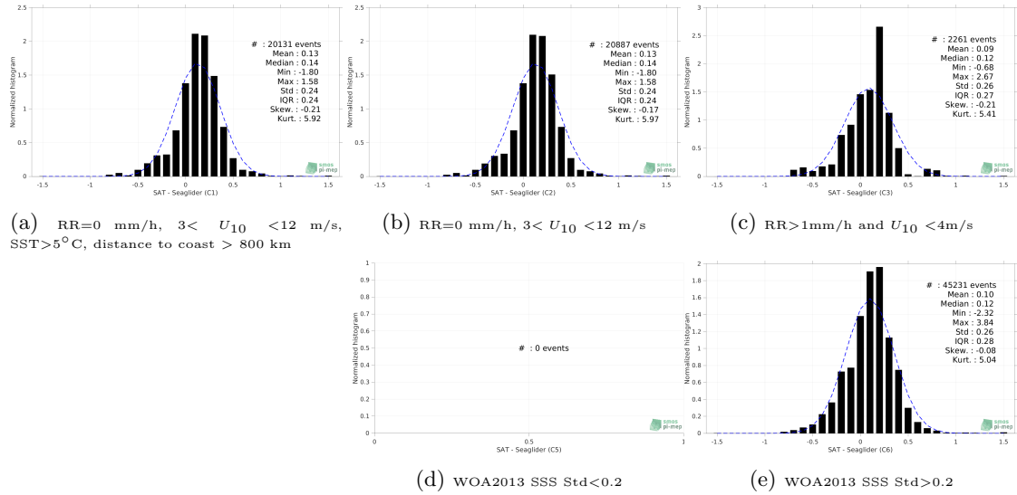
Figure 12: Normalized histogram of \Delta\text{SSS} (SMAP SSS L4 OI v1 - 7 Days (IPRC) - Seaglider) for 5 different subdatasets corresponding to: RR=0 mm/h, 3 < U_{10} < 12 m/s, SST>5°C, distance to coast > 800 km (a), RR=0 mm/h, 3 < U_{10} < 12 m/s (b), RR>1mm/h and U_{10} < 4 m/s (c), WOA2013 SSS Std<0.2 (d), WOA2013 SSS Std>0.2 (e).
