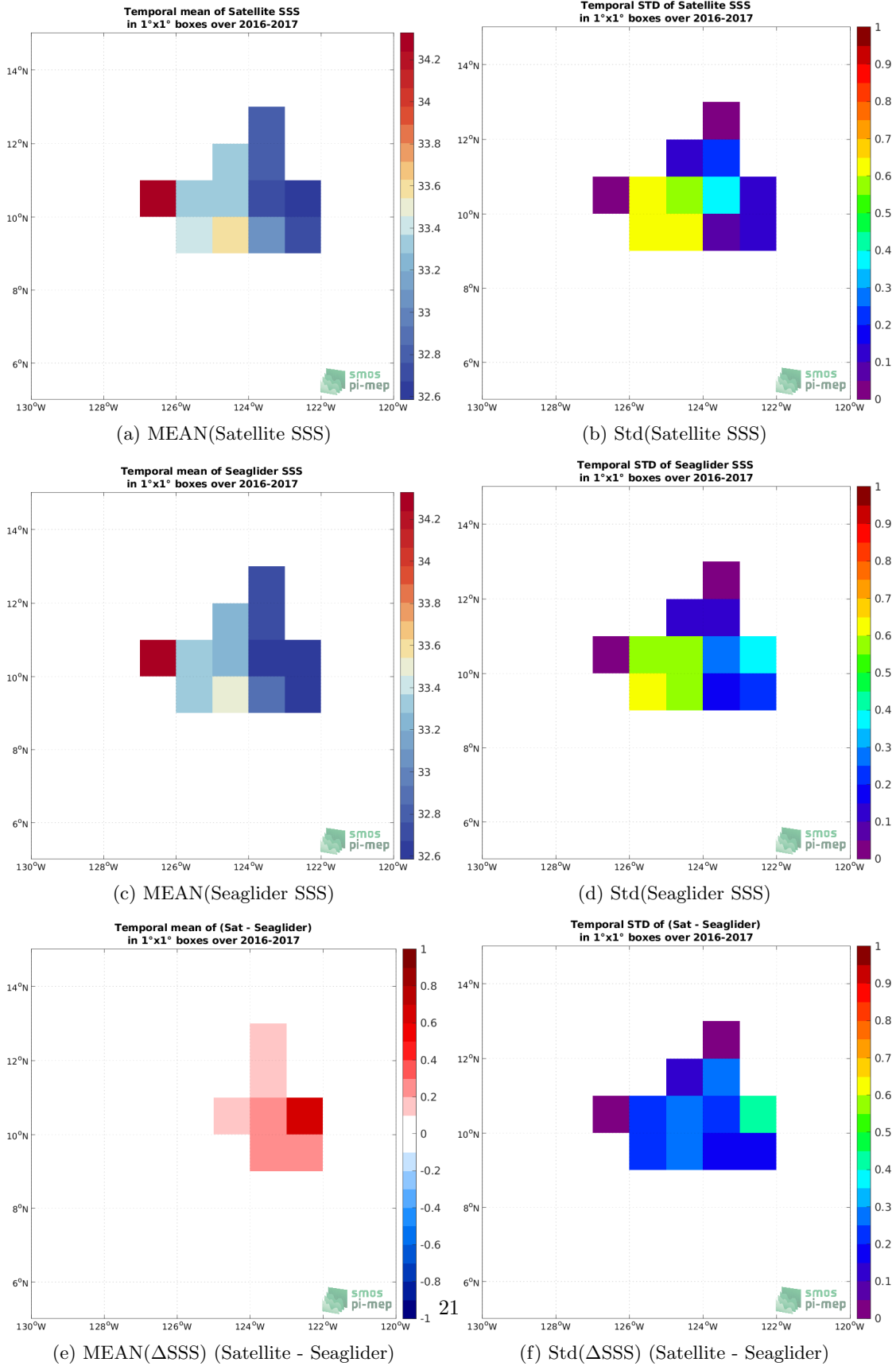
Figure 5: Temporal mean (left) and Std (right) of SSS from SMAP SSS L4 OI v1 - 7 Days (IPRC) (top), Seaglider (middle), and of \Delta SSS (Satellite - Seaglider). Only match-up pairs are used to generate these maps.
