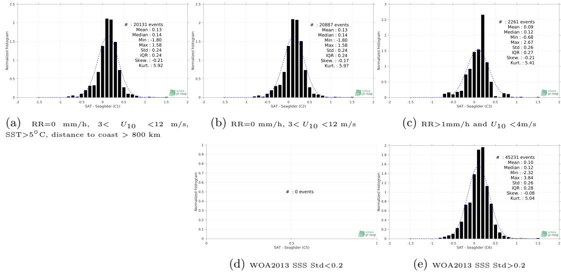
Figure 12: Normalized histogram of \Delta SSS (SMAP SSS L4 OI v1 - 7 Days (IPRC) - Seaglider) for 5 different subdatasets corresponding to: RR=0 mm/h, 3 < U_{10} < 12 m/s, SST>5°C, distance to coast > 800 km (a), RR=0 mm/h, 3 < U_{10} < 12 m/s (b), RR>1mm/h and U_{10} < 4 m/s (c), WOA2013 SSS Std<0.2 (d), WOA2013 SSS Std>0.2 (e).
