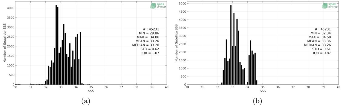
Figure 2: Histograms of SSS from Seaglader (a) and SMAP SSS L4 OI v1 - 7 Days (IPRC) (b) considering all match-up pairs per bins of 0.1 over the SPURS 2 Pi-MEP region and for the full satellite product period.
