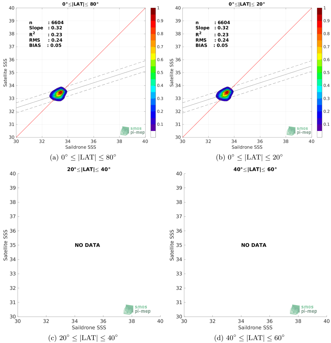
Figure 8: Contour maps of the concentration of SMAP SSS L4 OI v1 - 7 Days (IPRC) SSS (y-axis) versus Saildrone SSS (x-axis) at match-up pairs for different latitude bands. For each plot, the red line shows x=y . The black thin and dashed lines indicate a linear fit through the data cloud and the \pm 95\% confidence levels, respectively. The number match-up pairs n , the slope and R^2 coefficient of the linear fit, the root mean square (RMS) and the mean bias between satellite and in situ data are indicated for each latitude band in each plots.
