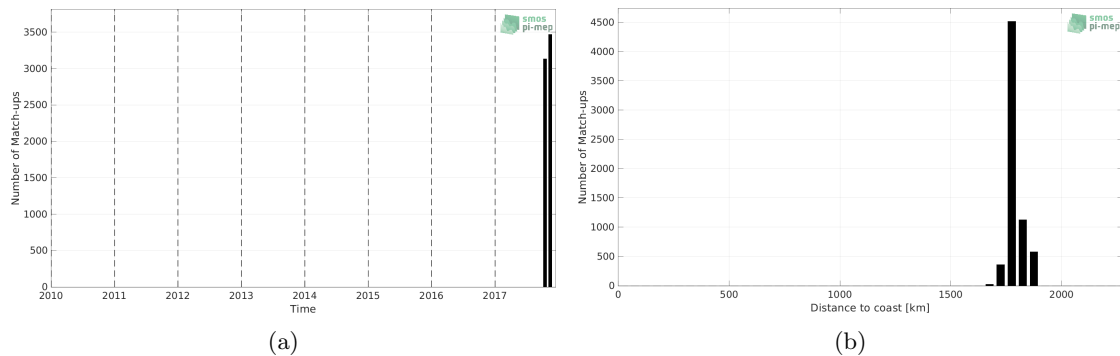
Figure 1: Number of match-ups between Saildrone and SMAP SSS L4 OI v1 - 7 Days (IPRC) SSS as a function of time (a) and as function of the distance to coast (b) over the SPURS 2 Pi-MEP region and for the full satellite product period.
