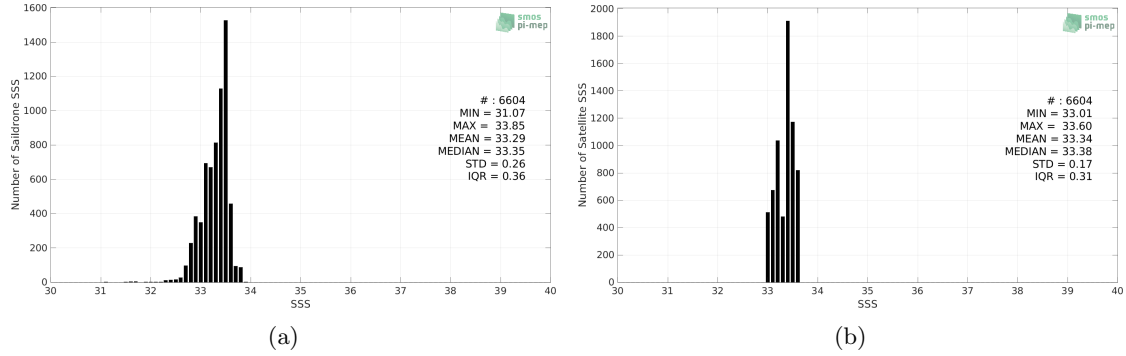
Figure 2: Histograms of SSS from Sairdrone (a) and SMAP SSS L4 OI v1 - 7 Days (IPRC) (b) considering all match-up pairs per bins of 0.1 over the SPURS 2 Pi-MEP region and for the full satellite product period.
