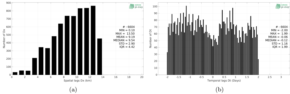
Figure 4: Histograms of the spatial (a) and temporal (b) lags between the location/time of the Saildrone measurement and the date of the corresponding SMAP SSS L4 OI v1 - 7 Days (IPRC) SSS pixel.
