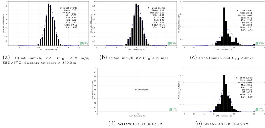
Figure 12: Normalized histogram of \Delta SSS (SMAP SSS L4 OI v1 - 7 Days (IPRC) - Saildrone) for 5 different subdatasets corresponding to: RR=0 mm/h, 3 < U_{10} < 12 m/s, SST>5°C, distance to coast > 800 km (a), RR=0 mm/h, 3 < U_{10} < 12 m/s (b), RR>1mm/h and U_{10} < 4 m/s (c), WOA2013 SSS Std<0.2 (d), WOA2013 SSS Std>0.2 (e).
