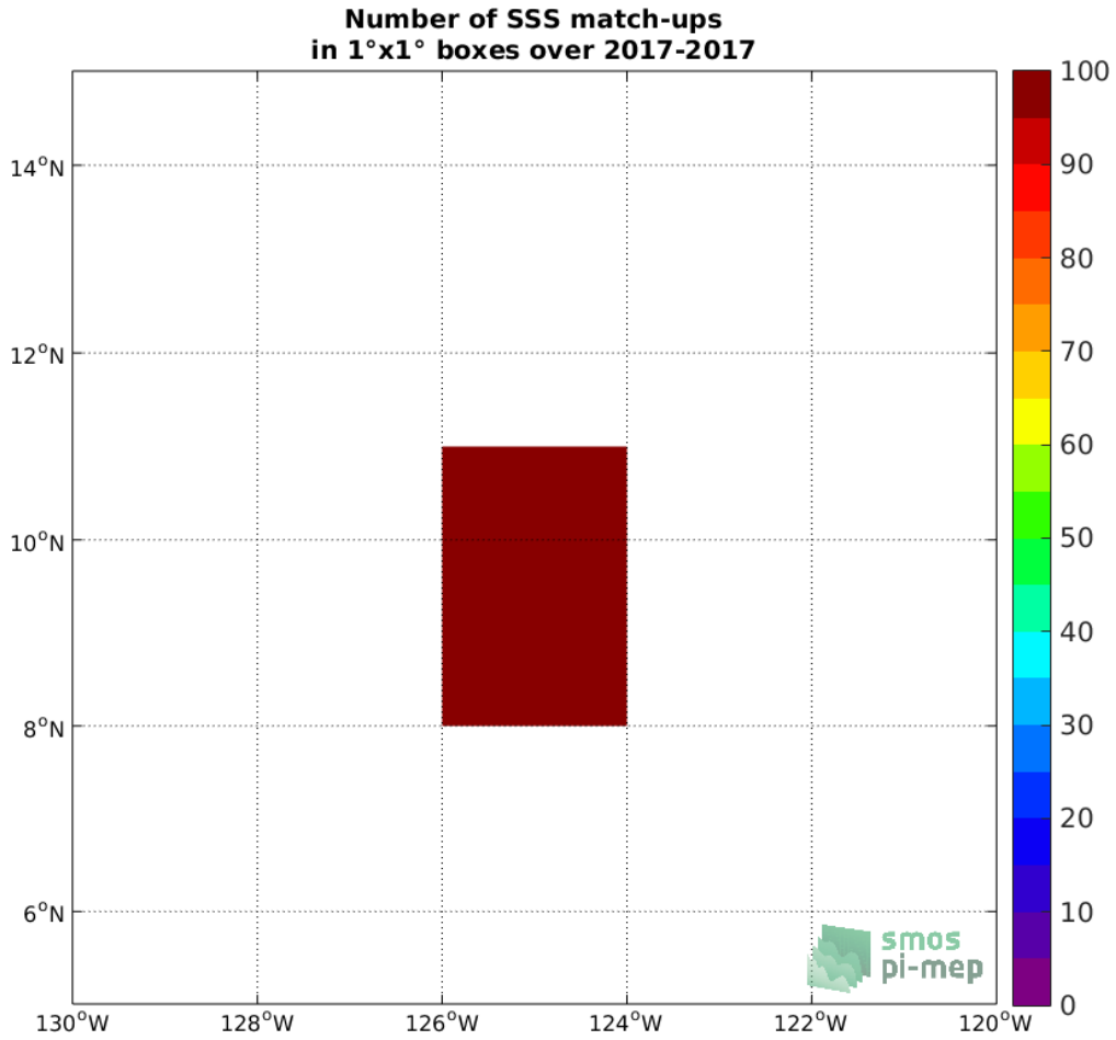
Figure 3: Number of SSS match-ups between Sairdrone SSS and the SMAP SSS L4 OI v1 - 7day (IPRC) SSS product for the SPURS 2 Pi-MEP region over 1°x1° boxes and for the full satellite product period.
