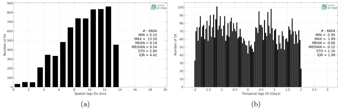
Figure 4: Histograms of the spatial (a) and temporal (b) lags between the location/time of the Saildrone measurement and the date of the corresponding SMAP SSS L4 OI v1 - 7day (IPRC) SSS pixel.
