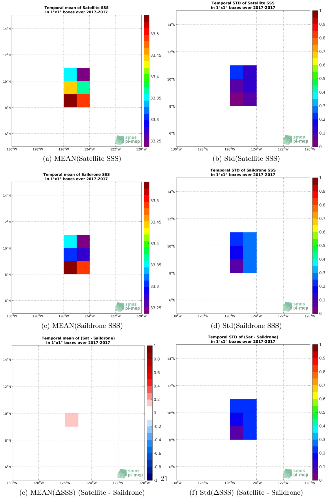
Figure 5: Temporal mean (left) and Std (right) of SSS from SMAP SSS L4 OI v1 - 7day (IPRC) (top), Saildrone (middle), and of \Delta SSS (Satellite - Saildrone). Only match-up pairs are used to generate these maps.
