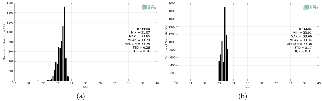
Figure 2: Histograms of SSS from Saildrone (a) and SMAP SSS L4 OI v1 - 7day (IPRC) (b) considering all match-up pairs per bins of 0.1 over the SPURS 2 Pi-MEP region and for the full satellite product period.
