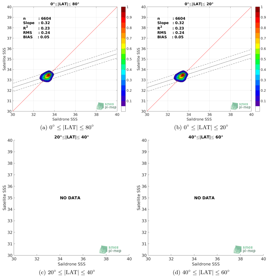
Figure 8: Contour maps of the concentration of SMAP SSS L4 OI v1 - 7day (IPRC) SSS (y-axis) versus Sailability SSS (x-axis) at match-up pairs for different latitude bands. For each plot, the red line shows x=y . The black thin and dashed lines indicate a linear fit through the data cloud and the \pm 95\% confidence levels, respectively. The number match-up pairs n , the slope and R^2 coefficient of the linear fit, the root mean square (RMS) and the mean bias between satellite and in situ data are indicated for each latitude band in each plots.
