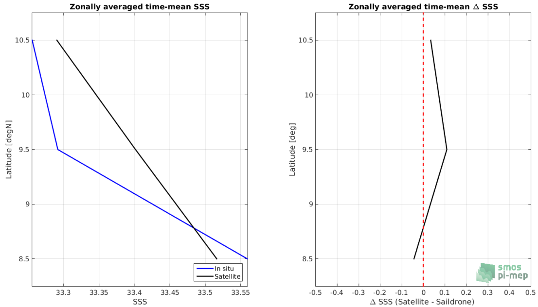
Figure 7: Left panel: Zonal mean SSS from SMAP SSS L4 OI v1 - 7day (IPRC) satellite product (black) and from Sairdrone (blue). Right panel: Zonal mean of \Delta SSS (Satellite - Sairdrone) for all the collected Pi-MEP match-up pairs estimated over the full satellite product period.
