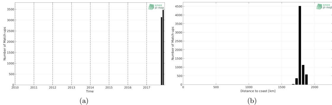
Figure 1: Number of match-ups between Saildrone and SMAP SSS L4 OI v1 - 7day (IPRC) SSS as a function of time (a) and as function of the distance to coast (b) over the SPURS 2 Pi-MEP region and for the full satellite product period.
