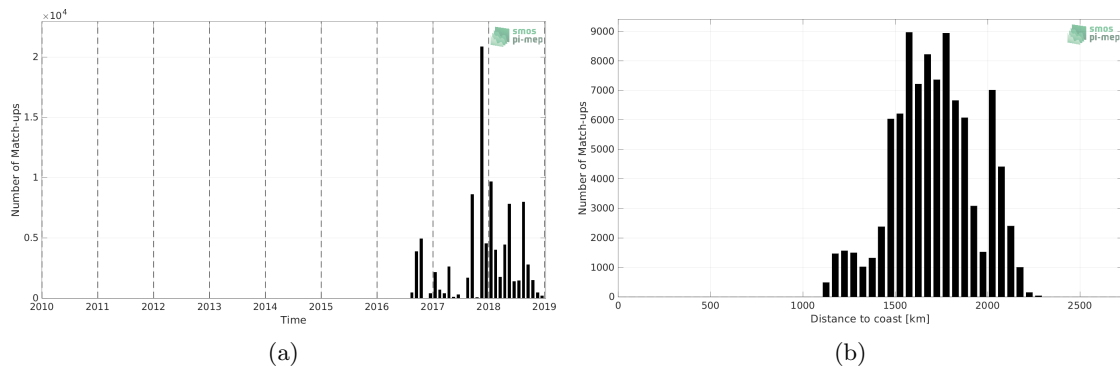
Figure 1: Number of match-ups between Surface drifters and SMAP SSS L4 OI v1 - 7 Days (IPRC) SSS as a function of time (a) and as function of the distance to coast (b) over the SPURS 2 Pi-MEP region and for the full satellite product period.
