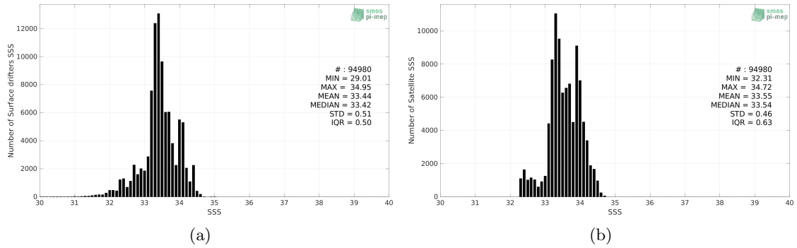
Figure 2: Histograms of SSS from Surface drifters (a) and SMAP SSS L4 OI v1 - 7 Days (IPRC) (b) considering all match-up pairs per bins of 0.1 over the SPURS 2 Pi-MEP region and for the full satellite product period.
