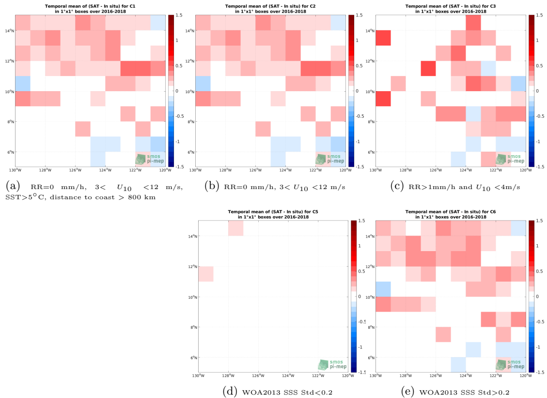
Figure 11: Temporal mean gridded over spatial boxes of size 1^\circ \times 1^\circ of \Delta SSS (SMAP SSS L4 OI v1 - 7 Days (IPRC) - Surface drifters) for 5 different subdatasets corresponding to:RR=0 mm/h, 3 < U_{10} < 12 m/s, SST > 5^\circ\text{C} , distance to coast > 800 km (a), RR=0 mm/h, 3 < U_{10} < 12 m/s (b), RR > 1 mm/h and U_{10} < 4 m/s (c), WOA2013 SSS Std < 0.2 (d), WOA2013 SSS Std > 0.2 (e).
