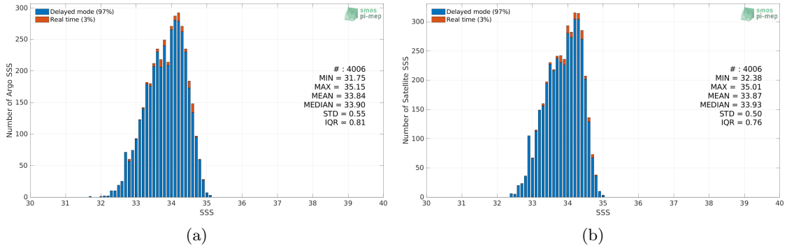
Figure 2: Histograms of SSS from Argo (a) and SMAP SSS L4 OI v1 - 7 Days (IPRC) (b) considering all match-up pairs per bins of 0.1 over the SPURS 2 Pi-MEP region and for the full satellite product period.
