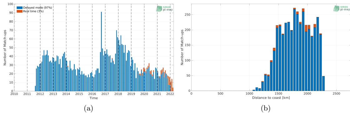
Figure 1: Number of match-ups between Argo and SMAP SSS L4 OI v1 - 7 Days (IPRC) SSS as a function of time (a) and as function of the distance to coast (b) over the SPURS 2 Pi-MEP region and for the full satellite product period.
