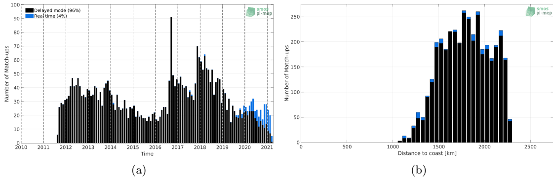
Figure 1: Number of match-ups between Argo and SMAP SSS L4 OI v1 - 7day (IPRC) SSS as a function of time (a) and as function of the distance to coast (b) over the SPURS 2 Pi-MEP region and for the full satellite product period.
