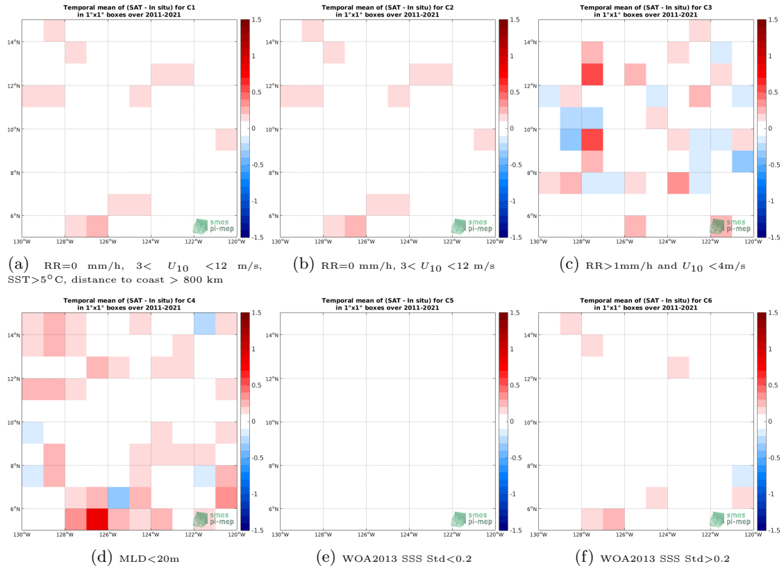
Figure 12: Temporal mean gridded over spatial boxes of size 1^\circ \times 1^\circ of \Delta SSS (SMAP SSS L4 OI v1 - 7day (IPRC) - Argo) for 6 different subdatasets corresponding to:RR=0 mm/h, 3 < U_{10} < 12 m/s, SST >5^\circ C, distance to coast > 800 km (a), RR=0 mm/h, 3 < U_{10} < 12 m/s (b), RR >1 mm/h and U_{10} < 4 m/s (c),MLD <20 m (d),WOA2013 SSS Std <0.2 (e),WOA2013 SSS Std >0.2 (f).
