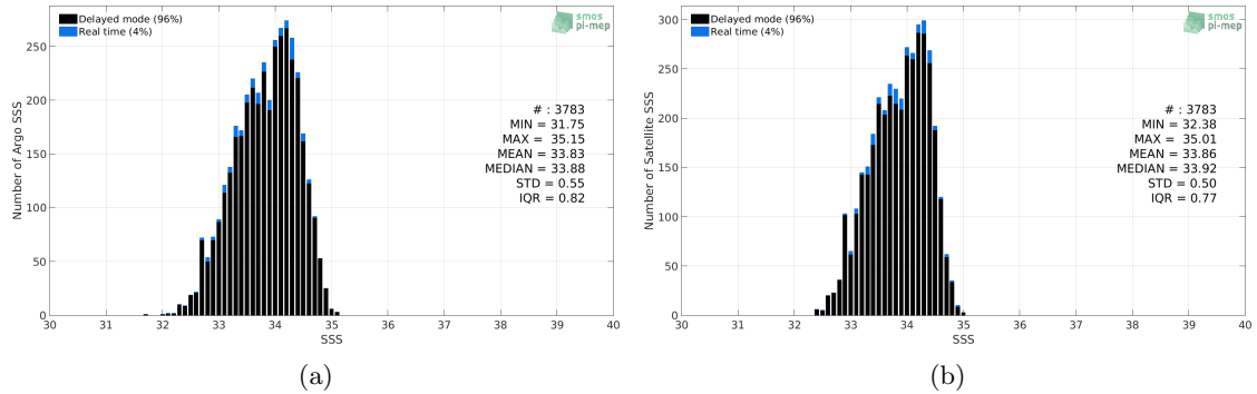
Figure 2: Histograms of SSS from Argo (a) and SMAP SSS L4 OI v1 - 7day (IPRC) (b) considering all match-up pairs per bins of 0.1 over the SPURS 2 Pi-MEP region and for the full satellite product period.
