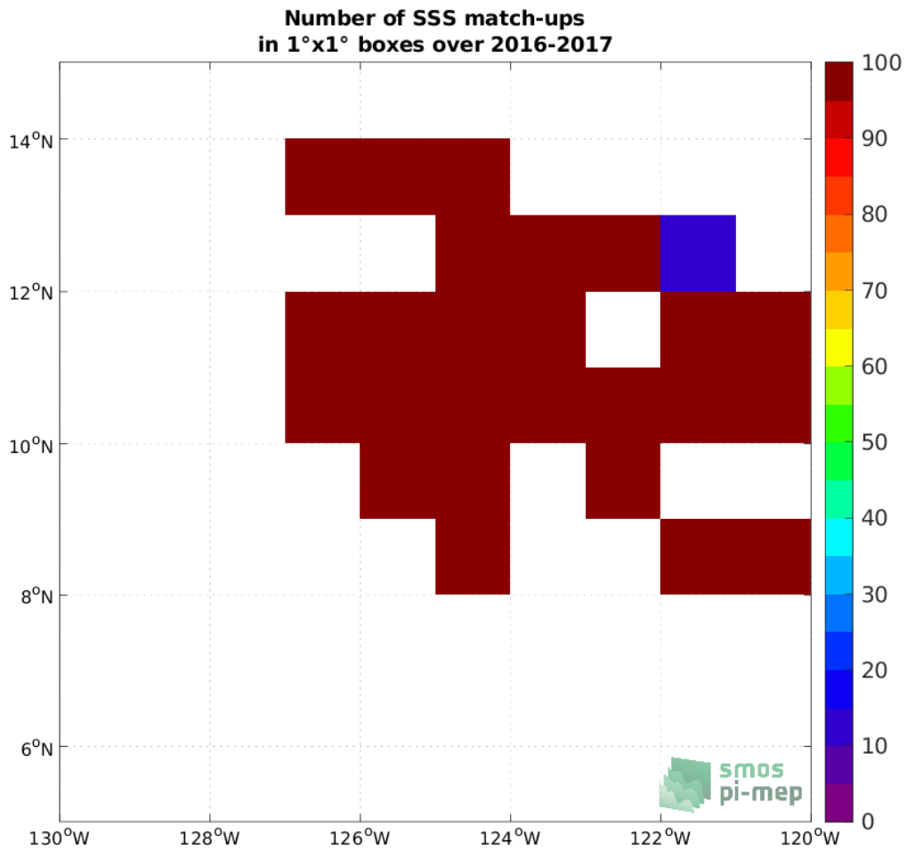
Figure 3: Number of SSS match-ups between Waveglider SSS and the SMAP SSS L4 OI v1 - Monthly (IPRC) SSS product for the SPURS 2 Pi-MEP region over 1°×1° boxes and for the full satellite product period.
