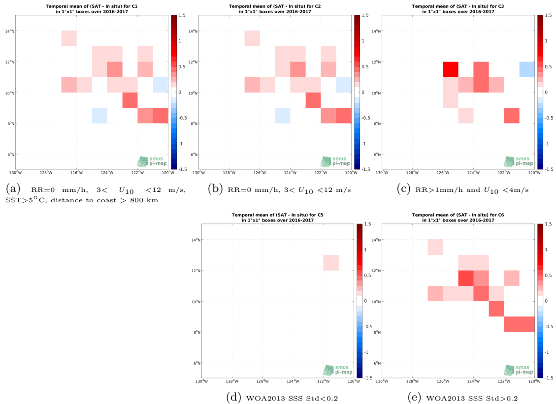
Figure 11: Temporal mean gridded over spatial boxes of size 1^\circ \times 1^\circ of \Delta SSS (SMAP SSS L4 OI v1 - Monthly (IPRC) - Waveglider) for 5 different subdatasets corresponding to:RR=0 mm/h, 3 < U_{10} < 12 m/s, SST >5^\circ\text{C} , distance to coast > 800 km (a), RR=0 mm/h, 3 < U_{10} < 12 m/s (b), RR >1 mm/h and U_{10} < 4 m/s (c), WOA2013 SSS Std <0.2 (d), WOA2013 SSS Std >0.2 (e).
