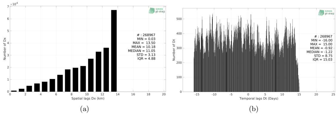
Figure 4: Histograms of the spatial (a) and temporal (b) lags between the location/time of the Waveglider measurement and the date of the corresponding SMAP SSS L4 OI v1 - Monthly (IPRC) SSS pixel.
