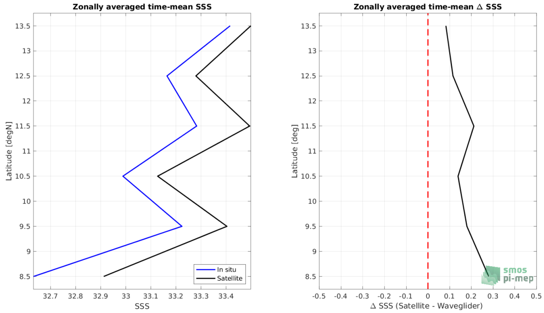
Figure 7: Left panel: Zonal mean SSS from SMAP SSS L4 OI v1 - Monthly (IPRC) satellite product (black) and from Waveglider (blue). Right panel: Zonal mean of \Delta SSS (Satellite - Waveglider) for all the collected Pi-MEP match-up pairs estimated over the full satellite product period.
