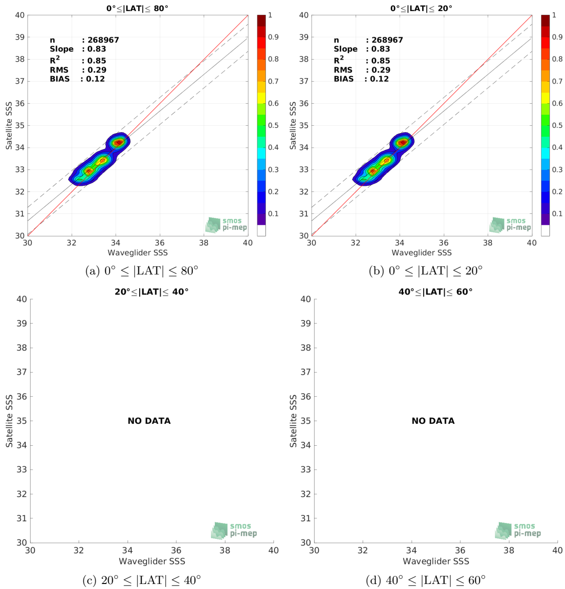
Figure 8: Contour maps of the concentration of SMAP SSS L4 OI v1 - Monthly (IPRC) SSS (y-axis) versus Waveglider SSS (x-axis) at match-up pairs for different latitude bands. For each plot, the red line shows x=y . The black thin and dashed lines indicate a linear fit through the data cloud and the \pm 95\% confidence levels, respectively. The number match-up pairs n , the slope and R^2 coefficient of the linear fit, the root mean square (RMS) and the mean bias between satellite and in situ data are indicated for each latitude band in each plots.
