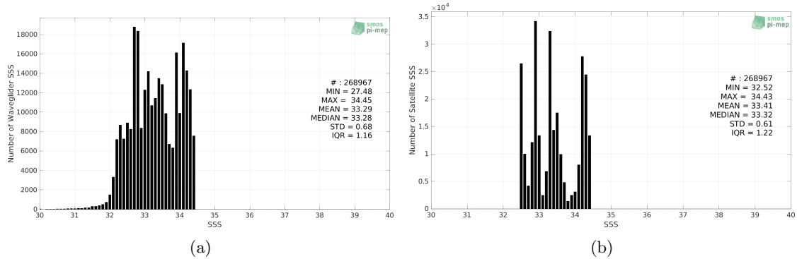
Figure 2: Histograms of SSS from Waveglider (a) and SMAP SSS L4 OI v1 - Monthly (IPRC) (b) considering all match-up pairs per bins of 0.1 over the SPURS 2 Pi-MEP region and for the full satellite product period.
