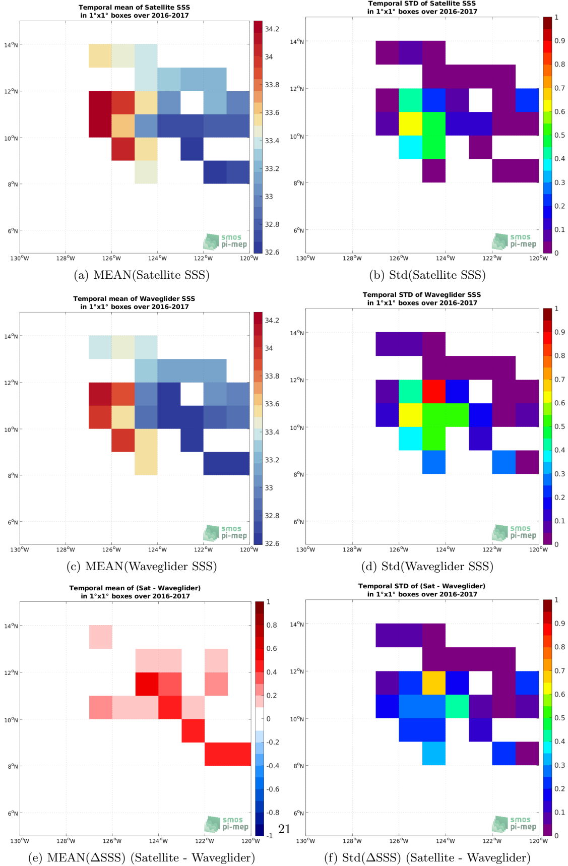
Figure 5: Temporal mean (left) and Std (right) of SSS from SMAP SSS L4 OI v1 - Monthly (IPRC) (top), Waveglider (middle), and of \Delta SSS (Satellite - Waveglider). Only match-up pairs are used to generate these maps.
