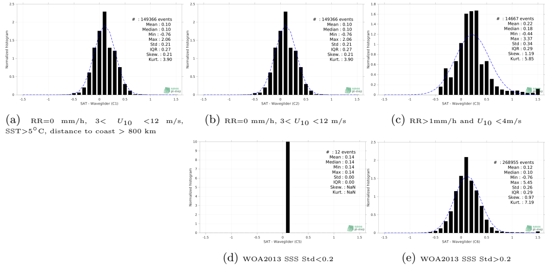
Figure 12: Normalized histogram of \Delta SSS (SMAP SSS L4 OI v1 - Monthly (IPRC) - Waveglider) for 5 different subdatasets corresponding to: RR=0 mm/h, 3 < U_{10} < 12 m/s, SST > 5°C, distance to coast > 800 km (a), RR=0 mm/h, 3 < U_{10} < 12 m/s (b), RR > 1mm/h and U_{10} < 4 m/s (c), WOA2013 SSS Std < 0.2 (d), WOA2013 SSS Std > 0.2 (e).
