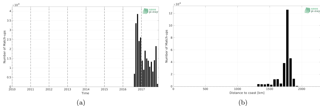
Figure 1: Number of match-ups between Waveglider and SMAP SSS L4 OI v1 - Monthly (IPRC) SSS as a function of time (a) and as function of the distance to coast (b) over the SPURS 2 Pi-MEP region and for the full satellite product period.
