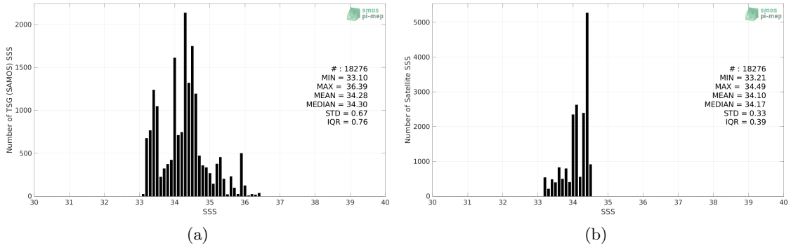
Figure 2: Histograms of SSS from TSG (SAMOS) (a) and SMAP SSS L4 OI v1 - Monthly (IPRC) (b) considering all match-up pairs per bins of 0.1 over the SPURS 2 Pi-MEP region and for the full satellite product period.
