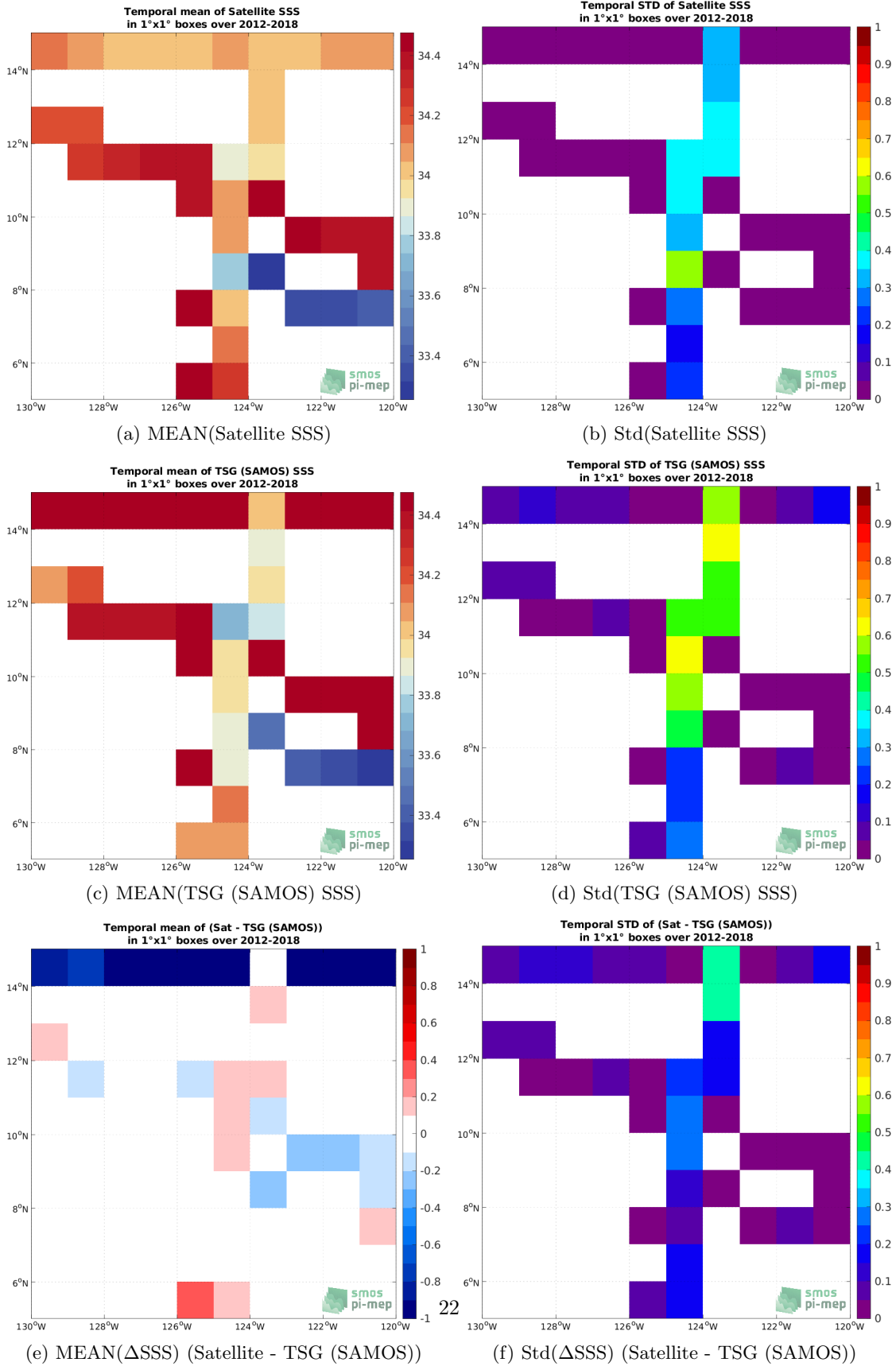
Figure 6: Temporal mean (left) and Std (right) of SSS from SMAP SSS L4 OI v1 - Monthly (IPRC) (top), TSG (SAMOS) (middle), and of \Delta SSS (Satellite - TSG (SAMOS)). Only match-up pairs are used to generate these maps.
