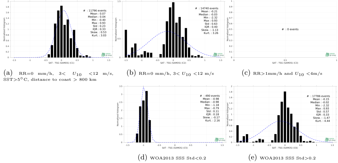
Figure 13: Normalized histogram of \Delta SSS (SMAP SSS L4 OI v1 - Monthly (IPRC) - TSG (SAMOS)) for 5 different subdatasets corresponding to: RR=0 mm/h, 3 < U_{10} < 12 m/s, SST > 5°C, distance to coast > 800 km (a), RR=0 mm/h, 3 < U_{10} < 12 m/s (b), RR > 1mm/h and U_{10} < 4 m/s (c), WOA2013 SSS Std < 0.2 (d), WOA2013 SSS Std > 0.2 (e).
