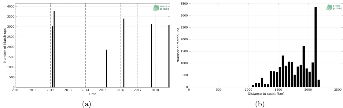
Figure 1: Number of match-ups between TSG (SAMOS) and SMAP SSS L4 OI v1 - Monthly (IPRC) SSS as a function of time (a) and as function of the distance to coast (b) over the SPURS 2 Pi-MEP region and for the full satellite product period.
