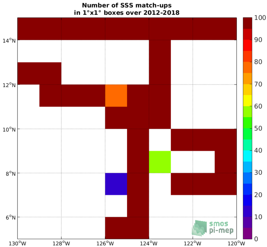
Figure 4: Number of SSS match-ups between TSG (SAMOS) SSS and the SMAP SSS L4 OI v1 - Monthly (IPRC) SSS product for the SPURS 2 Pi-MEP region over 1°x1° boxes and for the full satellite product period.
