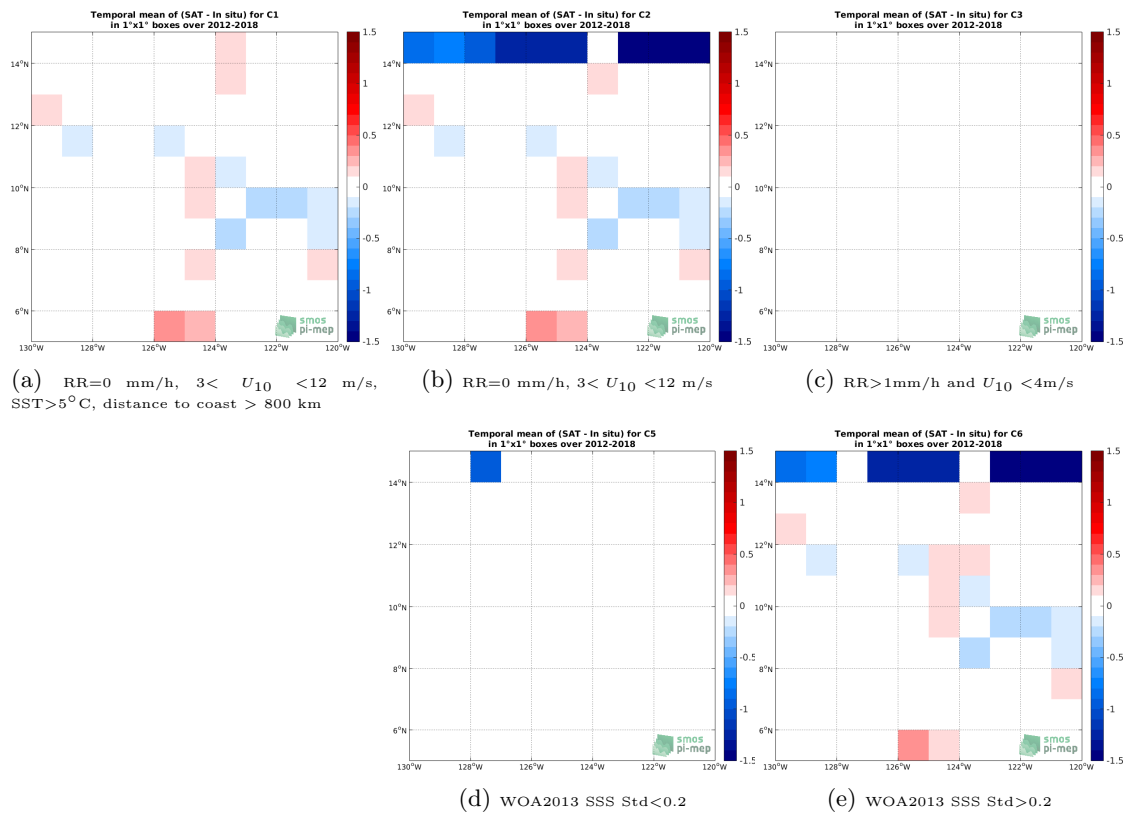
Figure 12: Temporal mean gridded over spatial boxes of size 1^\circ \times 1^\circ of \Delta SSS (SMAP SSS L4 OI v1 - Monthly (IPRC) - TSG (SAMOS)) for 5 different subdatasets corresponding to:RR=0 mm/h, 3 < U_{10} < 12 m/s, SST >5^\circ\text{C} , distance to coast > 800 km (a), RR=0 mm/h, 3 < U_{10} < 12 m/s (b), RR >1 mm/h and U_{10} < 4 m/s (c), WOA2013 SSS Std <0.2 (d), WOA2013 SSS Std >0.2 (e).
