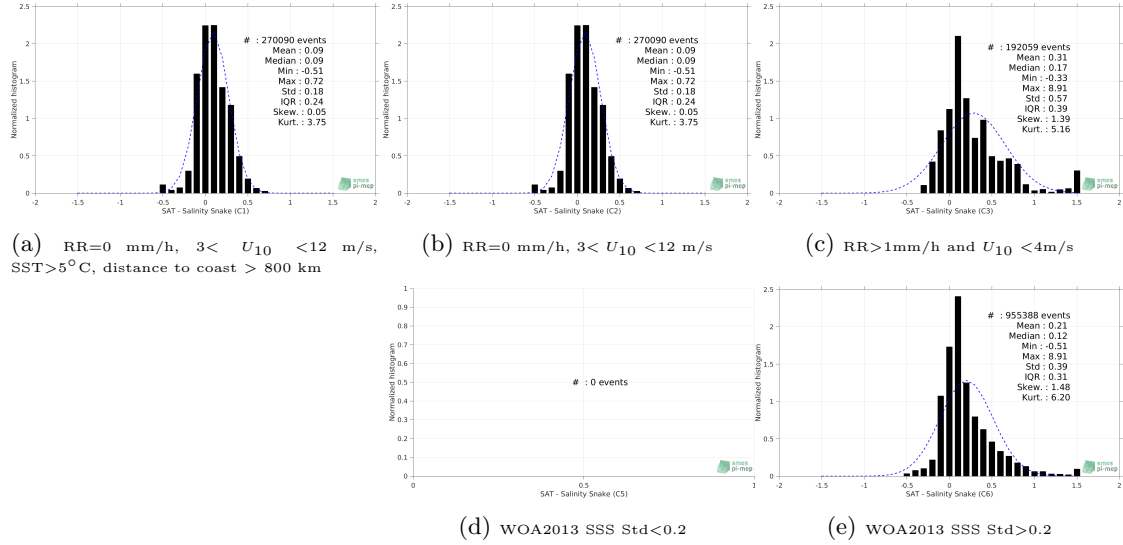
Figure 12: Normalized histogram of \Delta SSS (SMAP SSS L4 OI v1 - Monthly (IPRC) - Salinity Snake) for 5 different subdatasets corresponding to: RR=0 mm/h, 3 < U_{10} < 12 m/s, SST>5°C, distance to coast > 800 km (a), RR=0 mm/h, 3 < U_{10} < 12 m/s (b), RR>1mm/h and U_{10} < 4 m/s (c), WOA2013 SSS Std<0.2 (d), WOA2013 SSS Std>0.2 (e).
