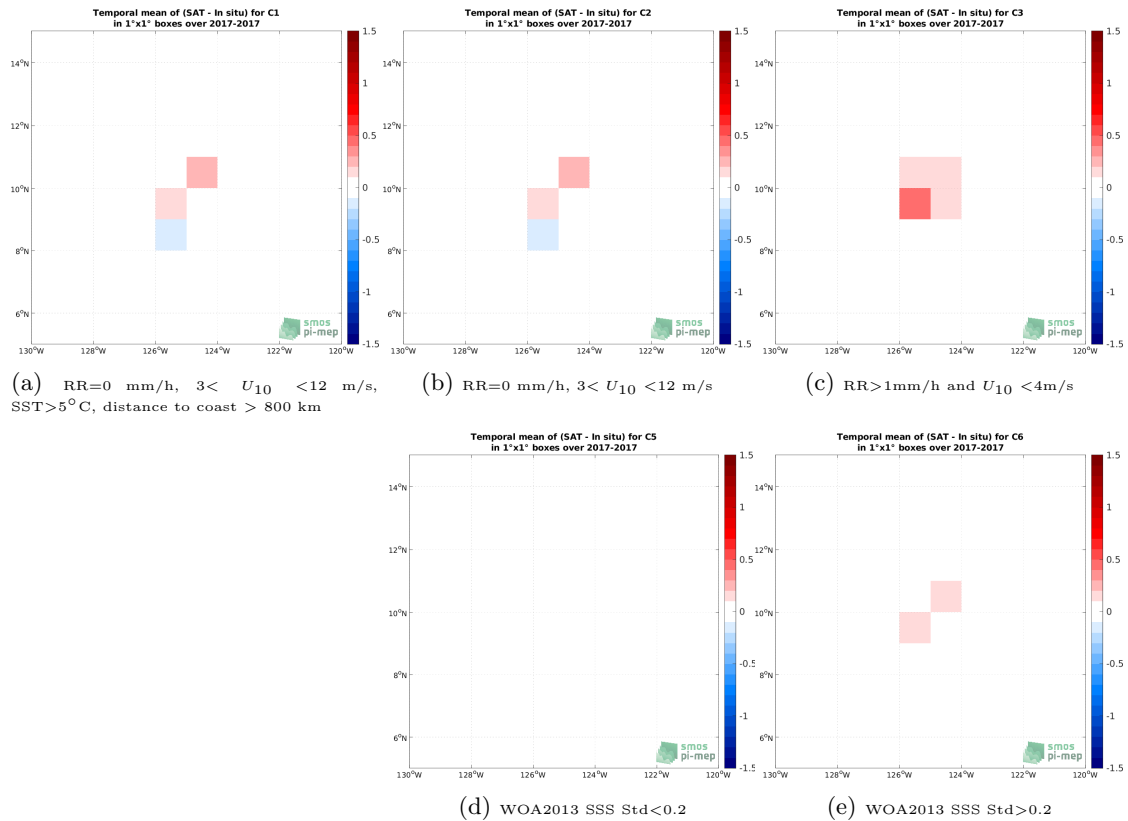
Figure 11: Temporal mean gridded over spatial boxes of size 1^\circ \times 1^\circ of \Delta SSS (SMAP SSS L4 OI v1 - Monthly (IPRC) - Saildrone) for 5 different subdatasets corresponding to:RR=0 mm/h, 3 < U_{10} < 12 m/s, SST >5^\circ C, distance to coast > 800 km (a), RR=0 mm/h, 3 < U_{10} < 12 m/s (b), RR >1 mm/h and U_{10} < 4 m/s (c), WOA2013 SSS Std <0.2 (d), WOA2013 SSS Std >0.2 (e).
