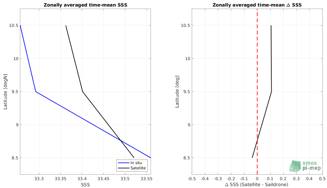
Figure 7: Left panel: Zonal mean SSS from SMAP SSS L4 OI v1 - Monthly (IPRC) satellite product (black) and from Sairdrone (blue). Right panel: Zonal mean of \Delta SSS (Satellite - Sairdrone) for all the collected Pi-MEP match-up pairs estimated over the full satellite product period.
