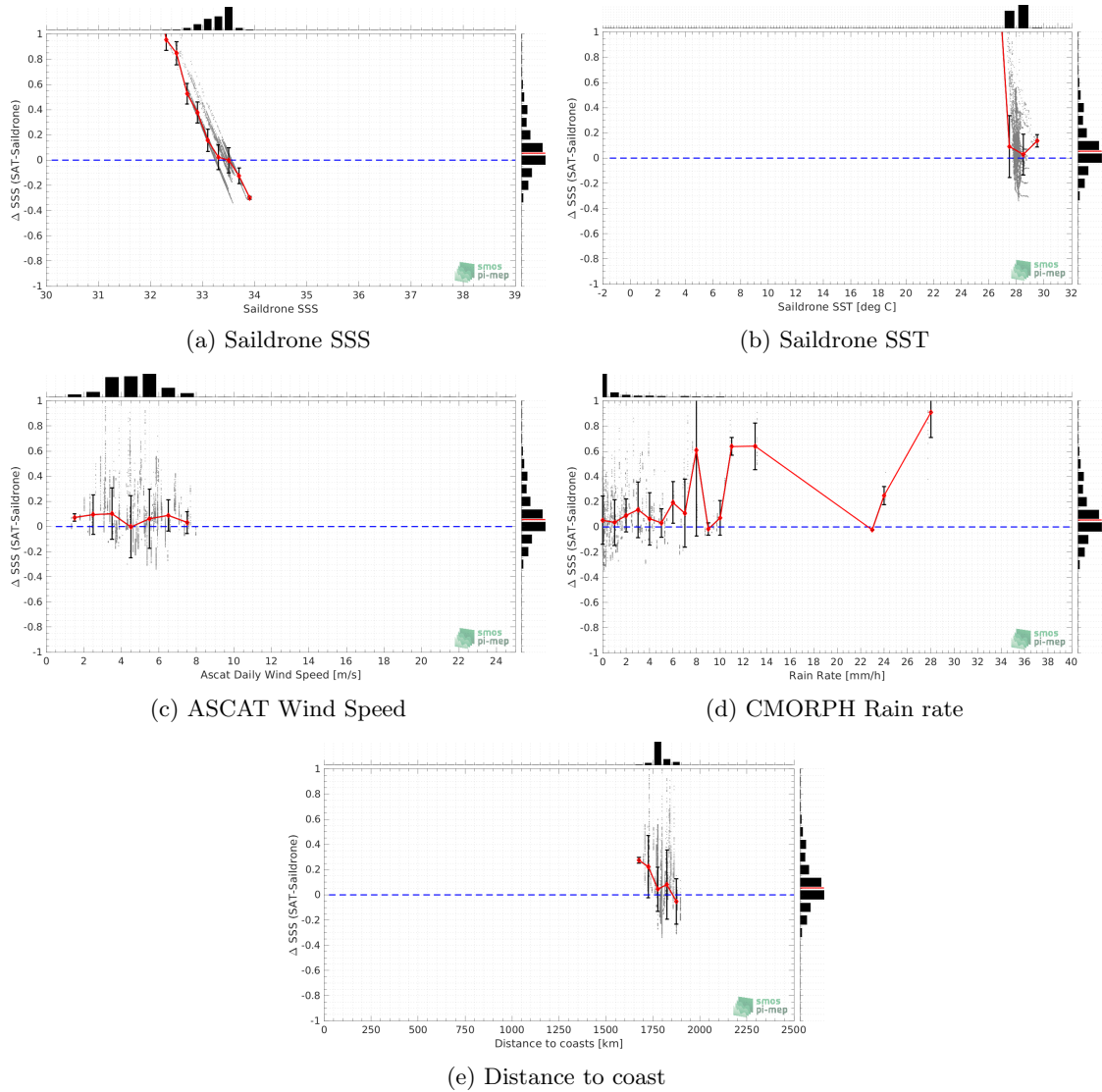
Figure 10: \Delta SSS (Satellite - Saildrone) sorted as function of Saildrone SSS a), Saildrone SST b), ASCAT Wind speed c), CMORPH rain rate d) and distance to coast (e). In all plots the median and Std of \Delta SSS for each bin is indicated by the red curves and black vertical thick bars ( \pm 1 Std)
