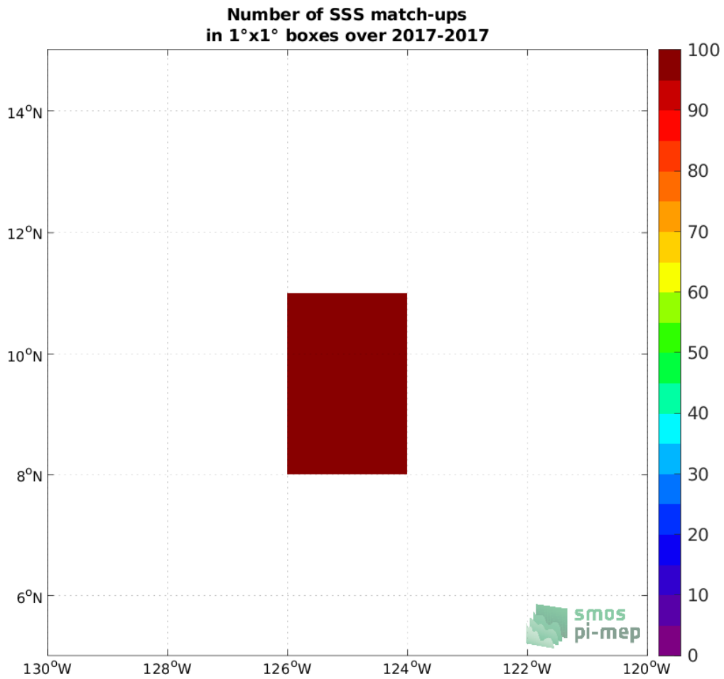
Figure 3: Number of SSS match-ups between Saildrone SSS and the SMAP SSS L4 OI v1 - Monthly (IPRC) SSS product for the SPURS 2 Pi-MEP region over 1°×1° boxes and for the full satellite product period.
