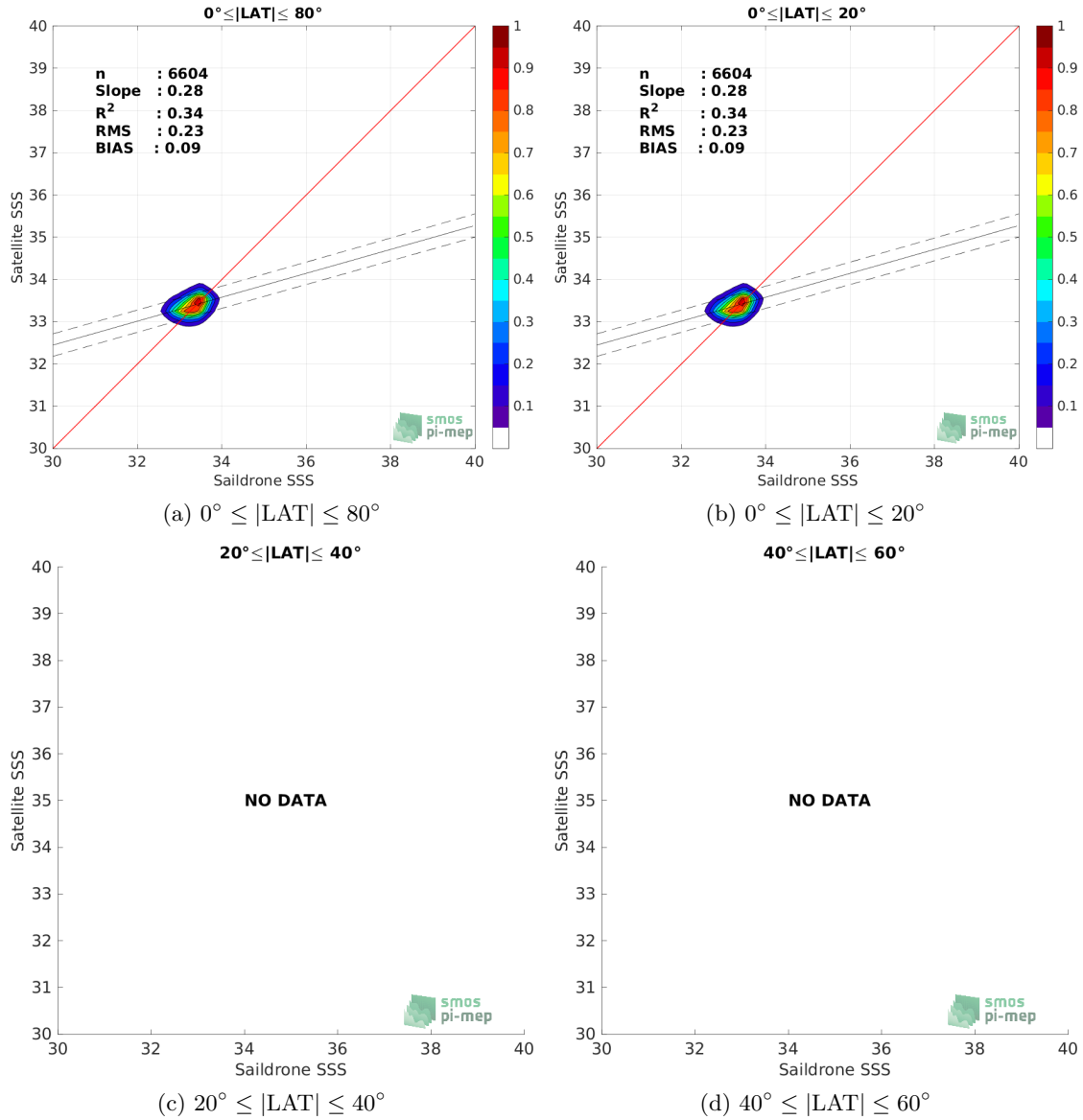
Figure 8: Contour maps of the concentration of SMAP SSS L4 OI v1 - Monthly (IPRC) SSS (y-axis) versus Saildrone SSS (x-axis) at match-up pairs for different latitude bands. For each plot, the red line shows x=y . The black thin and dashed lines indicate a linear fit through the data cloud and the \pm 95\% confidence levels, respectively. The number match-up pairs n , the slope and R^2 coefficient of the linear fit, the root mean square (RMS) and the mean bias between satellite and in situ data are indicated for each latitude band in each plots.
