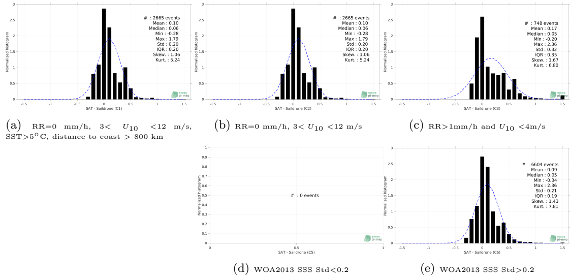
Figure 12: Normalized histogram of \Delta SSS (SMAP SSS L4 OI v1 - Monthly (IPRC) - Sairdrone) for 5 different subdatasets corresponding to: RR=0 mm/h, 3 < U_{10} < 12 m/s, SST > 5°C, distance to coast > 800 km (a), RR=0 mm/h, 3 < U_{10} < 12 m/s (b), RR > 1mm/h and U_{10} < 4 m/s (c), WOA2013 SSS Std < 0.2 (d), WOA2013 SSS Std > 0.2 (e).
