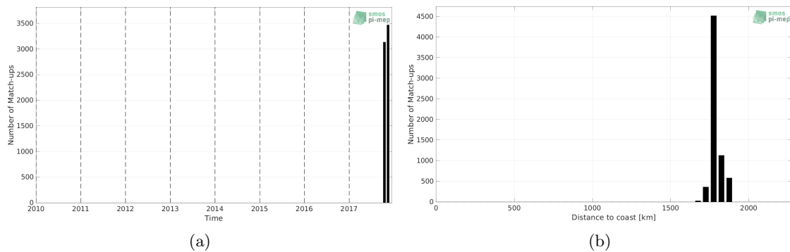
Figure 1: Number of match-ups between Saildrone and SMAP SSS L4 OI v1 - Monthly (IPRC) SSS as a function of time (a) and as function of the distance to coast (b) over the SPURS 2 Pi-MEP region and for the full satellite product period.
