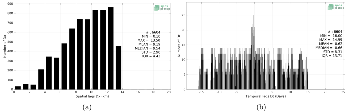
Figure 4: Histograms of the spatial (a) and temporal (b) lags between the location/time of the Saildrone measurement and the date of the corresponding SMAP SSS L4 OI v1 - Monthly (IPRC) SSS pixel.
