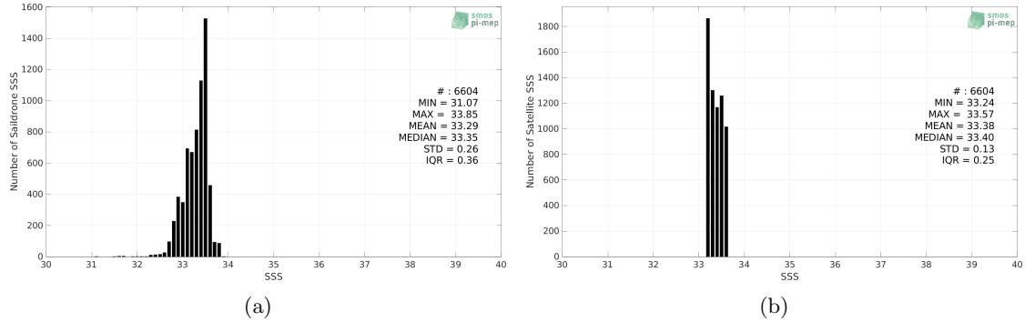
Figure 2: Histograms of SSS from Sairdrone (a) and SMAP SSS L4 OI v1 - Monthly (IPRC) (b) considering all match-up pairs per bins of 0.1 over the SPURS 2 Pi-MEP region and for the full satellite product period.
