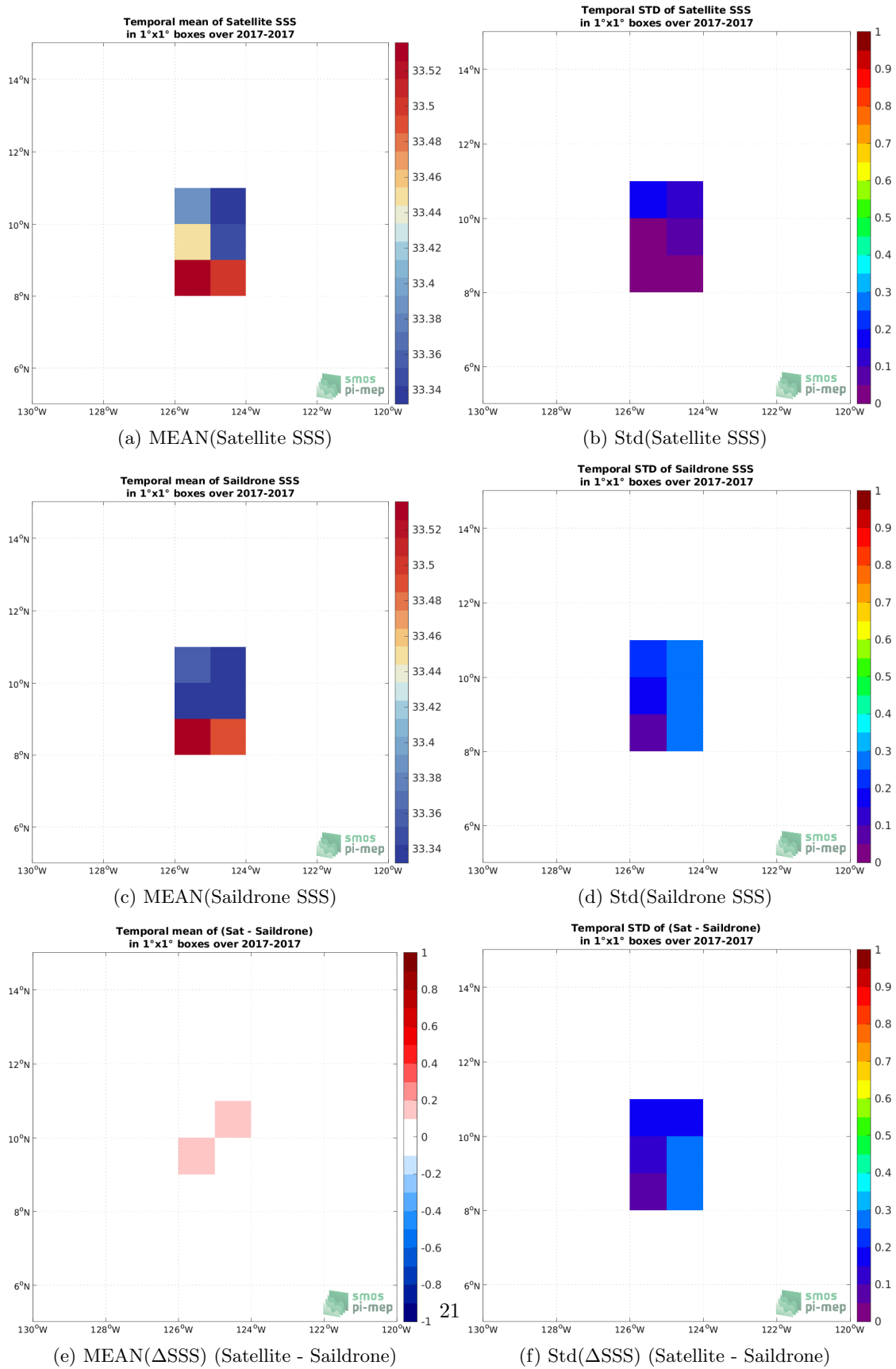
Figure 5: Temporal mean (left) and Std (right) of SSS from SMAP SSS L4 OI v1 - Monthly (IPRC) (top), Saildrone (middle), and of \Delta SSS (Satellite - Saildrone). Only match-up pairs are used to generate these maps.
