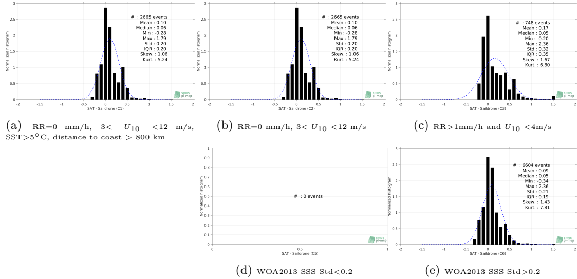
Figure 12: Normalized histogram of \Delta SSS (SMAP SSS L4 OI v1 - Monthly (IPRC) - Saildrone) for 5 different subdatasets corresponding to: RR=0 mm/h, 3 < U_{10} < 12 m/s, SST>5°C, distance to coast > 800 km (a), RR=0 mm/h, 3 < U_{10} < 12 m/s (b), RR>1mm/h and U_{10} < 4 m/s (c), WOA2013 SSS Std<0.2 (d), WOA2013 SSS Std>0.2 (e).
