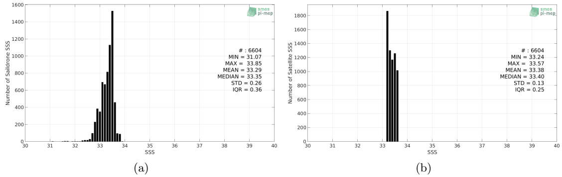
Figure 2: Histograms of SSS from Sairdrono (a) and SMAP SSS L4 OI v1 - Monthly (IPRC) (b) considering all match-up pairs per bins of 0.1 over the SPURS 2 Pi-MEP region and for the full satellite product period.
