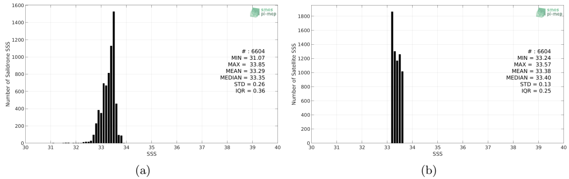
Figure 2: Histograms of SSS from Sairdronne (a) and SMAP SSS L4 OI v1 - Monthly (IPRC) (b) considering all match-up pairs per bins of 0.1 over the SPURS 2 Pi-MEP region and for the full satellite product period.
