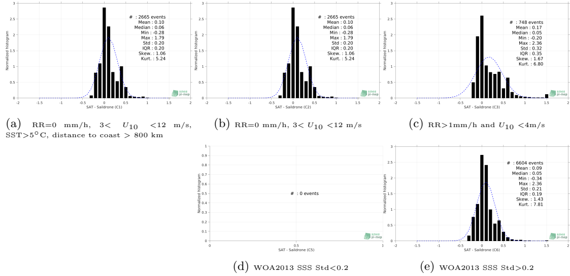
Figure 12: Normalized histogram of \Delta SSS (SMAP SSS L4 OI v1 - Monthly (IPRC) - Saildrone) for 5 different subdatasets corresponding to: RR=0 mm/h, 3 < U_{10} < 12 m/s, SST>5°C, distance to coast > 800 km (a), RR=0 mm/h, 3 < U_{10} < 12 m/s (b), RR>1mm/h and U_{10} < 4 m/s (c), WOA2013 SSS Std<0.2 (d), WOA2013 SSS Std>0.2 (e).
