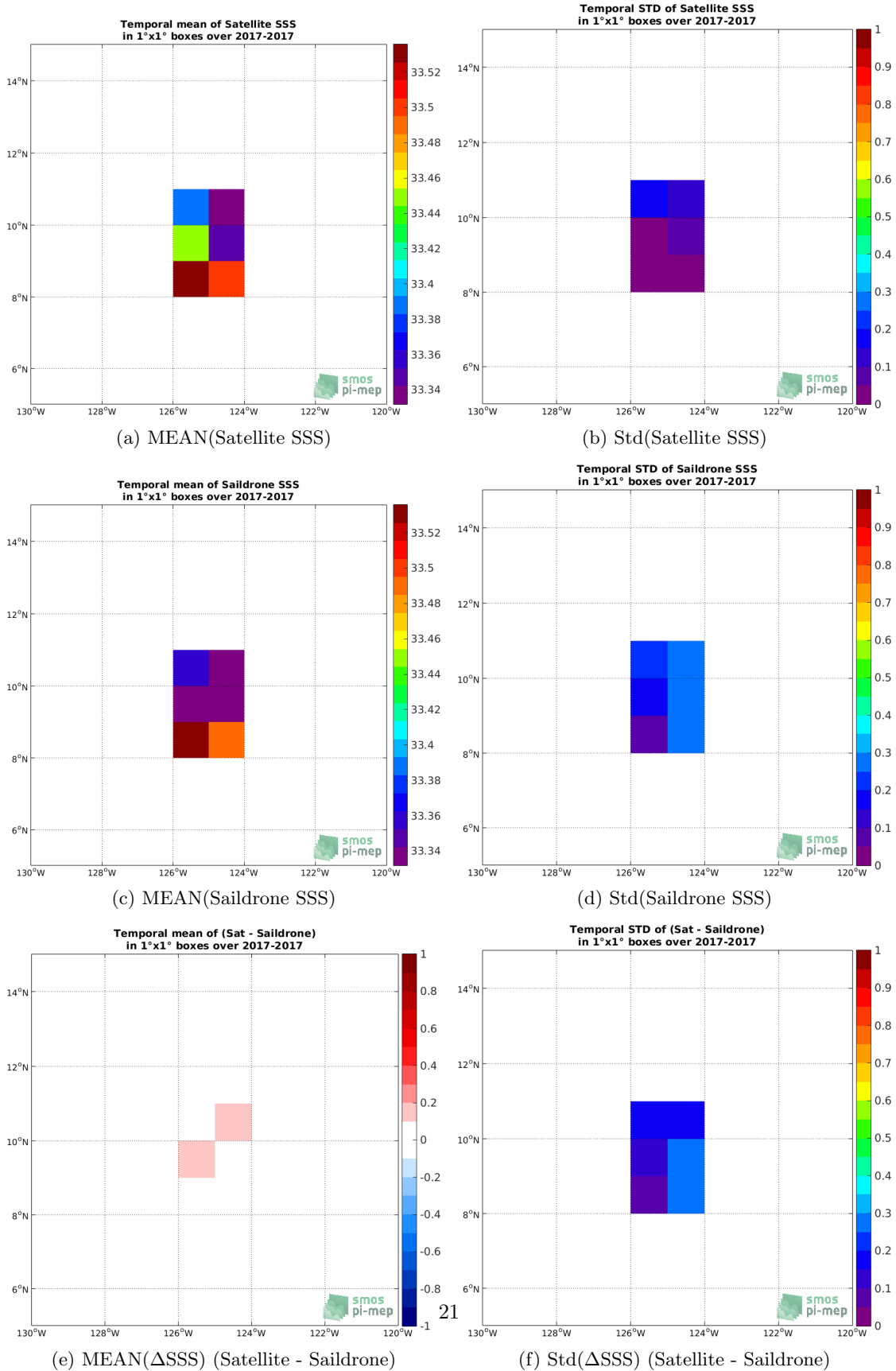
Figure 5: Temporal mean (left) and Std (right) of SSS from SMAP SSS L4 OI v1 - Monthly (IPRC) (top), Saildrone (middle), and of \Delta SSS (Satellite - Saildrone). Only match-up pairs are used to generate these maps.
