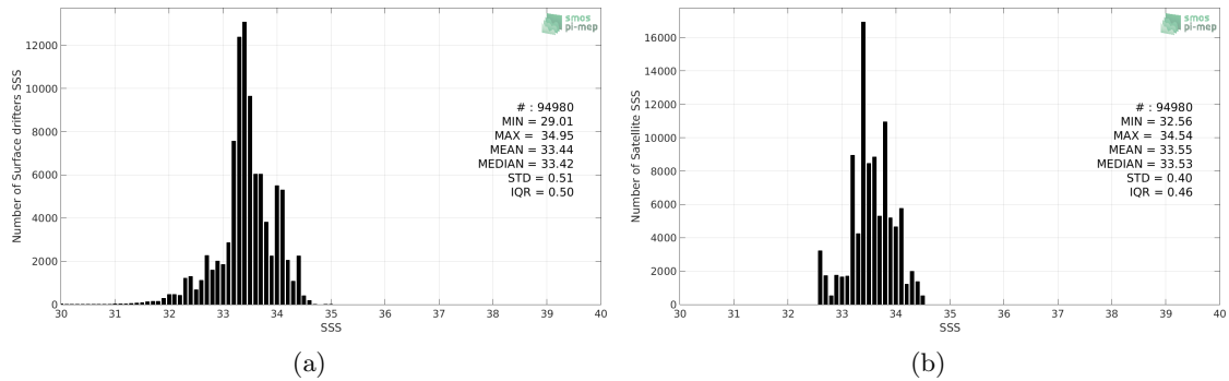
Figure 2: Histograms of SSS from Surface drifters (a) and SMAP SSS L4 OI v1 - Monthly (IPRC) (b) considering all match-up pairs per bins of 0.1 over the SPURS 2 Pi-MEP region and for the full satellite product period.
