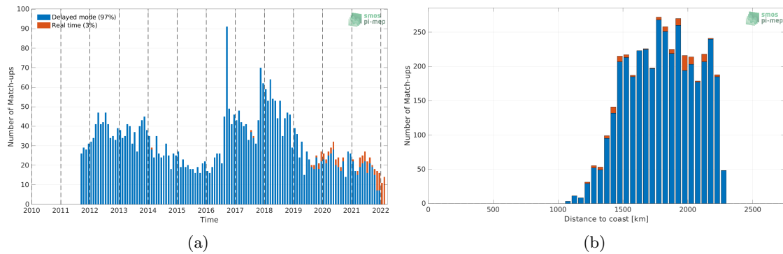
Figure 1: Number of match-ups between Argo and SMAP SSS L4 OI v1 - Monthly (IPRC) SSS as a function of time (a) and as function of the distance to coast (b) over the SPURS 2 Pi-MEP region and for the full satellite product period.
