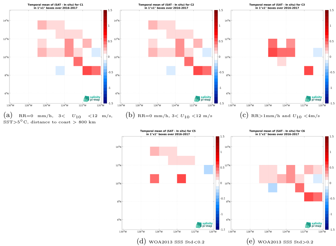
Figure 14: Temporal mean gridded over spatial boxes of size 1^\circ \times 1^\circ of \Delta SSS (SMAP SSS L4 OI v3 - Monthly (ESR) - Waveglider (SPURS 2)) for 5 different subdatasets corresponding to:RR=0 mm/h, 3 < U_{10} < 12 m/s, SST >5^\circ C, distance to coast > 800 km (a), RR=0 mm/h, 3 < U_{10} < 12 m/s (b), RR >1 mm/h and U_{10} < 4 m/s (c), WOA2013 SSS Std <0.2 (d), WOA2013 SSS Std >0.2 (e).
