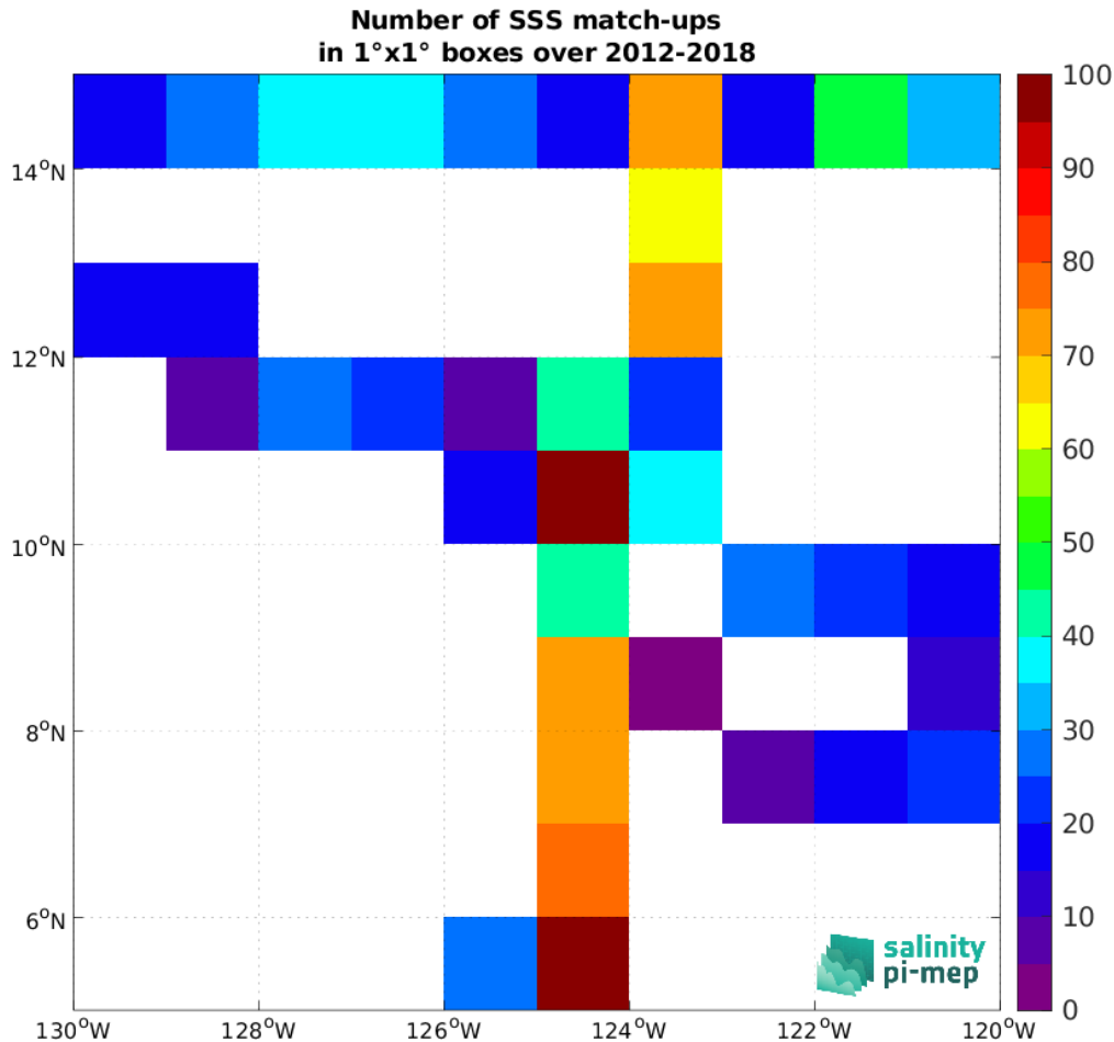
Figure 5: Number of SSS match-ups between TSG (SAMOS) SSS and the SMAP SSS L4 OI v3 - Monthly (ESR) SSS product for the SPURS 2 Pi-MEP region over 1^\circ \times 1^\circ boxes and for the full satellite product period.
