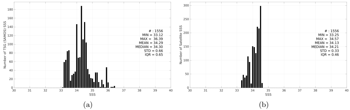
Figure 3: Histograms of SSS from TSG (SAMOS) (a) and SMAP SSS L4 OI v3 - Monthly (ESR) (b) considering all match-up pairs per bins of 0.1 over the SPURS 2 Pi-MEP region and for the full satellite product period.
