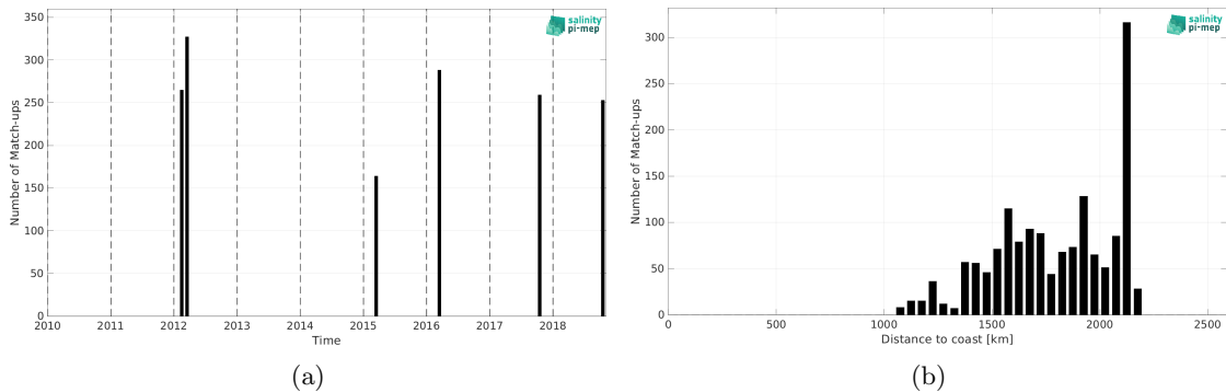
Figure 2: Number of match-ups between TSG (SAMOS) and SMAP SSS L4 OI v3 - Monthly (ESR) SSS as a function of time (a) and as function of the distance to coast (b) over the SPURS 2 Pi-MEP region and for the full satellite product period.
