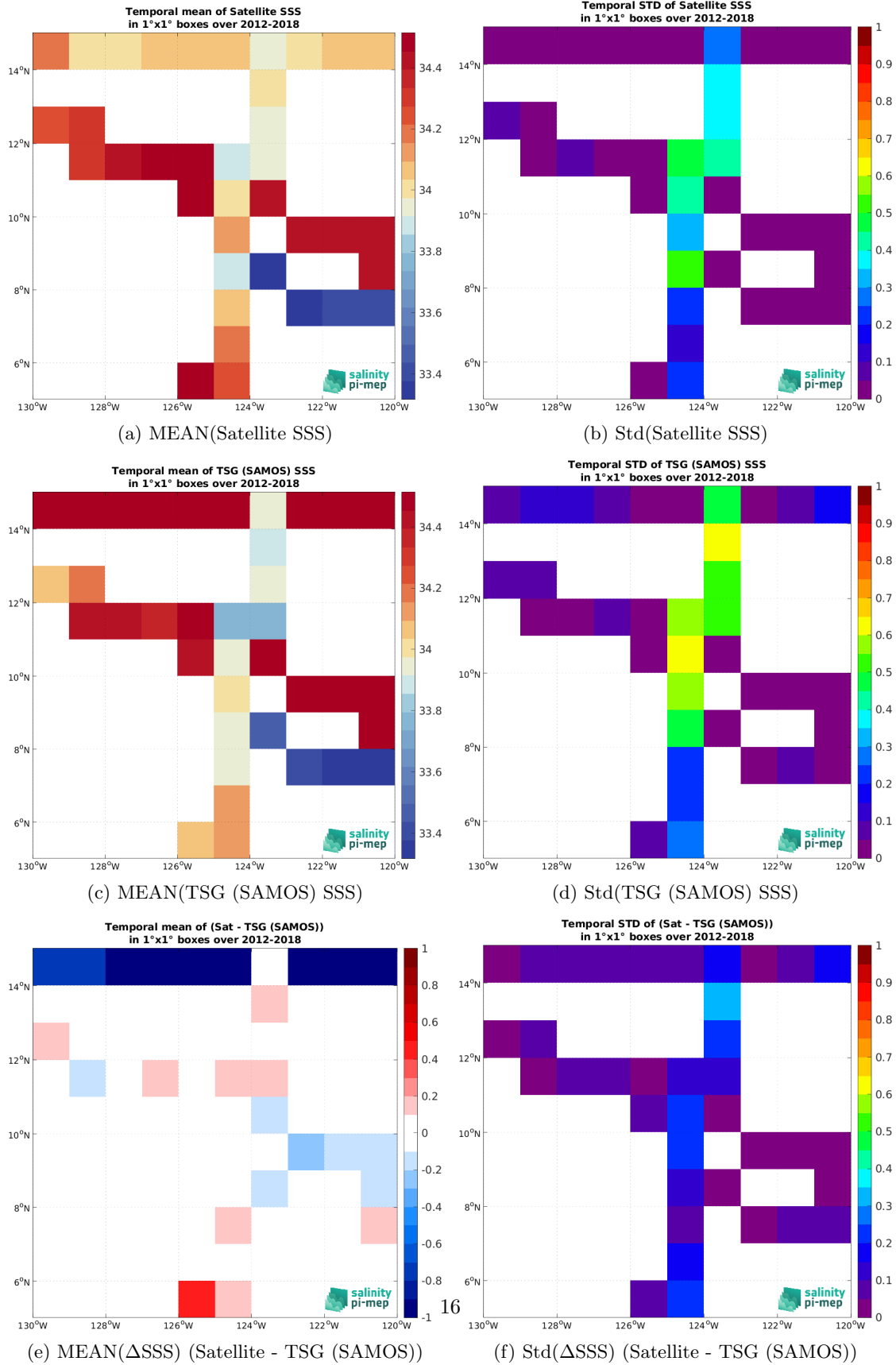
Figure 7: Temporal mean (left) and Std (right) of SSS from SMAP SSS L4 OI v3 - Monthly (ESR) (top), TSG (SAMOS) (middle), and of \Delta SSS (Satellite - TSG (SAMOS)). Only match-up pairs are used to generate these maps.
