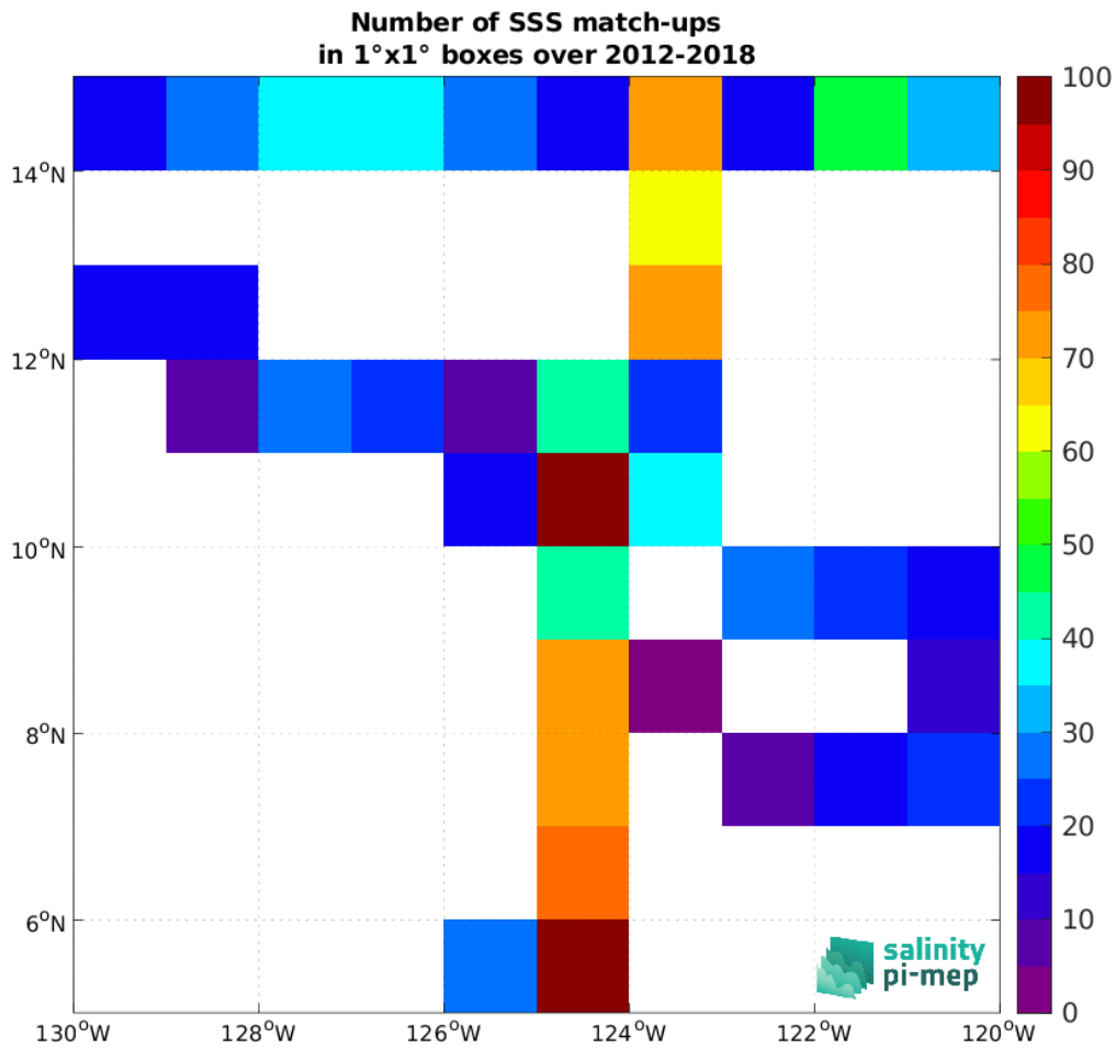
Figure 5: Number of SSS match-ups between TSG (SAMOS) SSS and the SMAP SSS L4 OI v3 - Monthly (ESR) SSS product for the SPURS 2 Pi-MEP region over 1°x1° boxes and for the full satellite product period.
