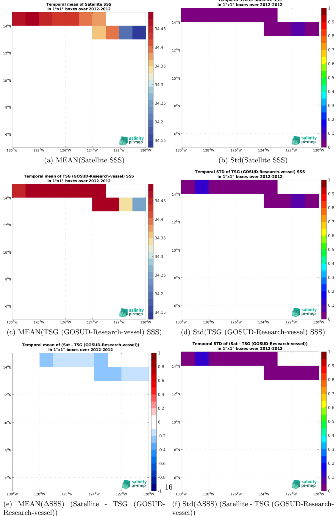
Figure 7: Temporal mean (left) and Std (right) of SSS from SMAP SSS L4 OI v3 - Monthly (ESR) (top), TSG (GOSUD-Research-vessel) (middle), and of \Delta SSS (Satellite - TSG (GOSUD-Research-vessel)). Only match-up pairs are used to generate these maps.
