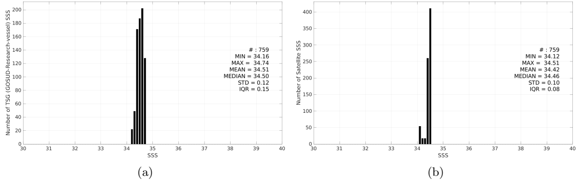
Figure 3: Histograms of SSS from TSG (GOSUD-Research-vessel) (a) and SMAP SSS L4 OI v3 - Monthly (ESR) (b) considering all match-up pairs per bins of 0.1 over the SPURS 2 Pi-MEP region and for the full satellite product period.
