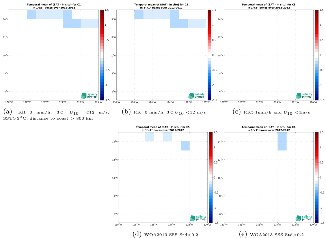
Figure 14: Temporal mean gridded over spatial boxes of size 1^\circ \times 1^\circ of \Delta SSS (SMAP SSS L4 OI v3 - Monthly (ESR) - TSG (GOSUD-Research-vessel)) for 5 different subdatasets corresponding to:RR=0 mm/h, 3 < U_{10} < 12 m/s, SST >5^\circ\text{C} , distance to coast > 800 km (a), RR=0 mm/h, 3 < U_{10} < 12 m/s (b), RR >1 mm/h and U_{10} < 4 m/s (c), WOA2013 SSS Std <0.2 (d), WOA2013 SSS Std >0.2 (e).
