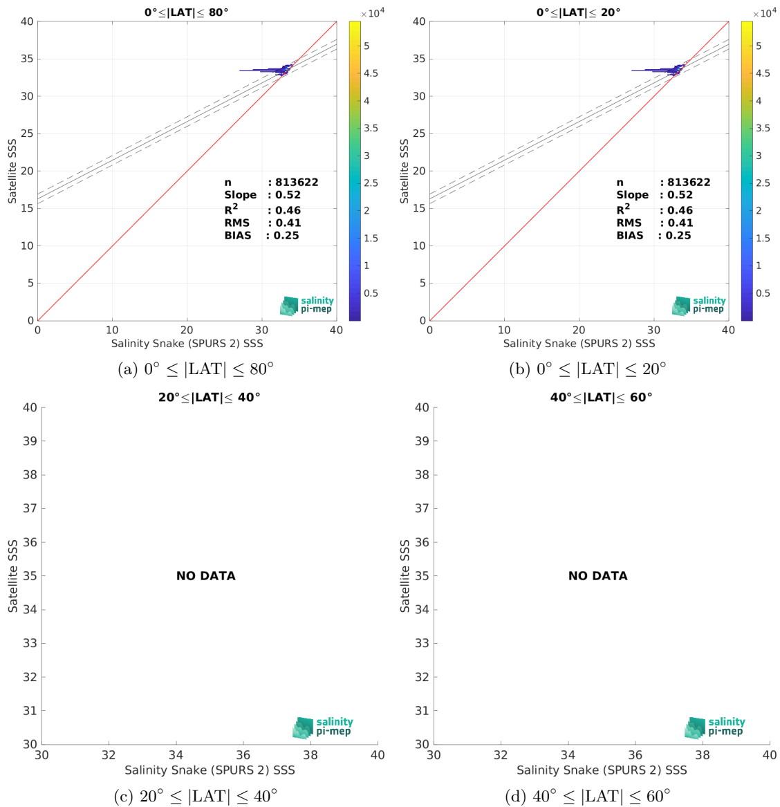
Figure 10: Contour maps of the concentration of SMAP SSS L4 OI v3 - Monthly (ESR) SSS (y-axis) versus Salinity Snake (SPURS 2) SSS (x-axis) at match-up pairs for different latitude bands. For each plot, the red line shows x=y . The black thin and dashed lines indicate a linear fit through the data cloud and the \pm 95\% confidence levels, respectively. The number match-up pairs n , the slope and R^2 coefficient of the linear fit, the root mean square (RMS) and the mean bias between satellite and in situ data are indicated for each latitude band in each plots.
