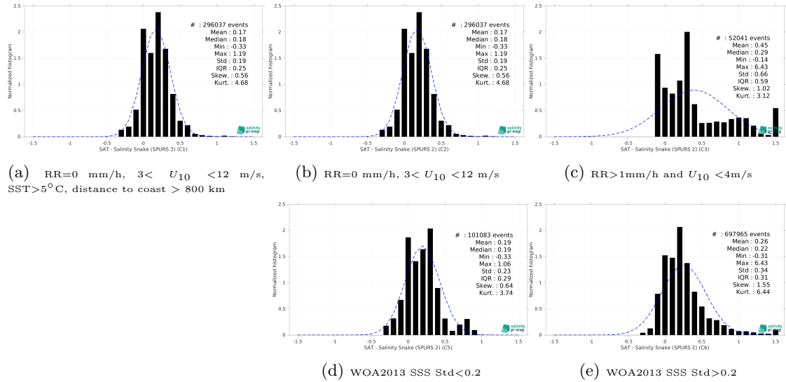
Figure 15: Normalized histogram of \Delta SSS (SMAP SSS L4 OI v3 - Monthly (ESR) - Salinity Snake (SPURS 2)) for 5 different subdatasets corresponding to: RR=0 mm/h, 3 < U_{10} < 12 m/s, SST > 5°C, distance to coast > 800 km (a), RR=0 mm/h, 3 < U_{10} < 12 m/s (b), RR > 1mm/h and U_{10} < 4 m/s (c), WOA2013 SSS Std < 0.2 (d), WOA2013 SSS Std > 0.2 (e).
