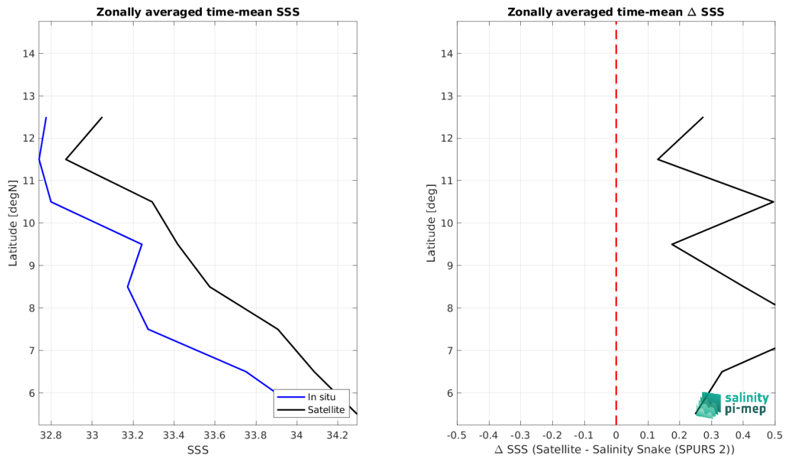
Figure 9: Left panel: Zonal mean SSS from SMAP SSS L4 OI v3 - Monthly (ESR) satellite product (black) and from Salinity Snake (SPURS 2) (blue). Right panel: Zonal mean of \Delta SSS (Satellite - Salinity Snake (SPURS 2)) for all the collected Pi-MEP match-up pairs estimated over the full satellite product period.
