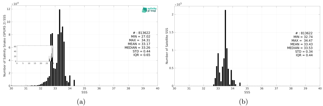
Figure 3: Histograms of SSS from Salinity Snake (SPURS 2) (a) and SMAP SSS L4 OI v3 - Monthly (ESR) (b) considering all match-up pairs per bins of 0.1 over the SPURS 2 Pi-MEP region and for the full satellite product period.
