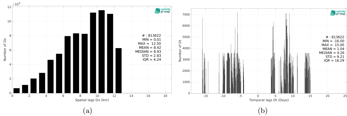
Figure 6: Histograms of the spatial (a) and temporal (b) lags between the location/time of the Salinity Snake (SPURS 2) measurement and the date of the corresponding SMAP SSS L4 OI v3 - Monthly (ESR) SSS pixel.
