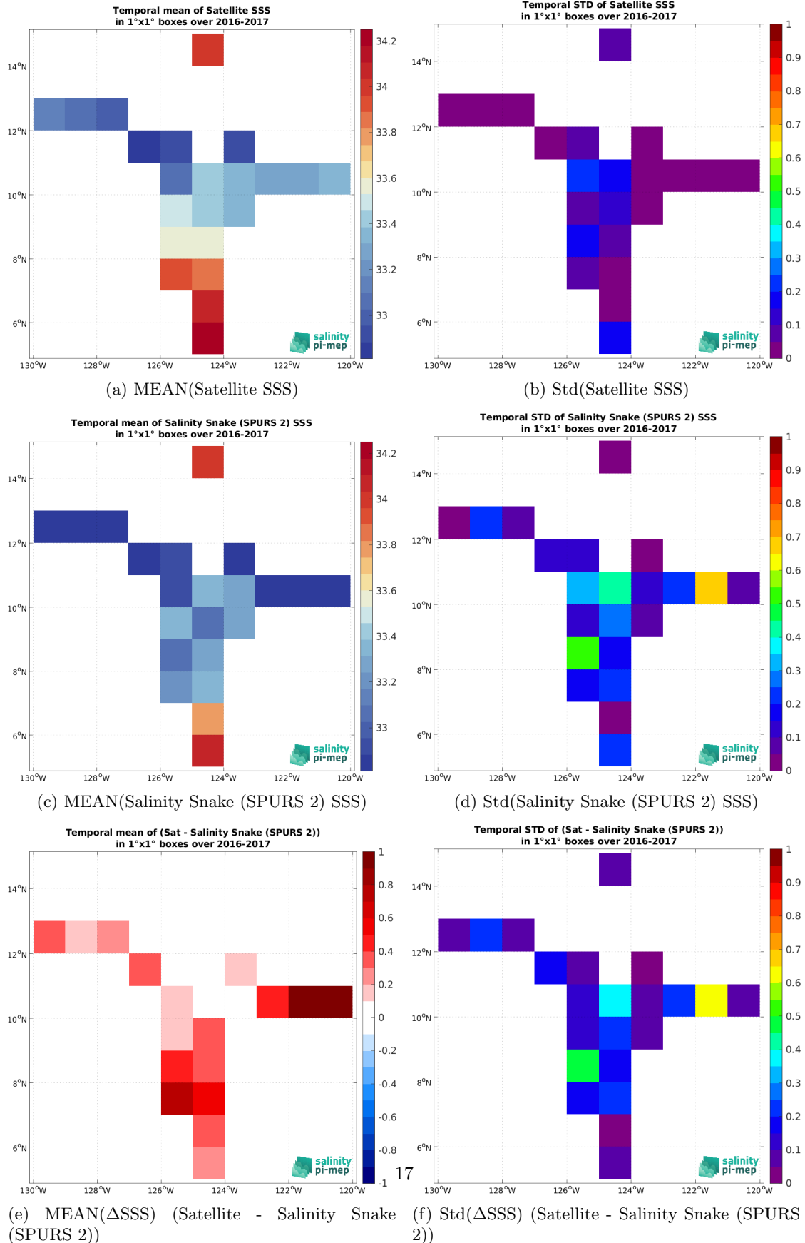
Figure 7: Temporal mean (left) and Std (right) of SSS from SMAP SSS L4 OI v3 - Monthly (ESR) (top), Salinity Snake (SPURS 2) (middle), and of \Delta SSS (Satellite - Salinity Snake (SPURS 2)). Only match-up pairs are used to generate these maps.
