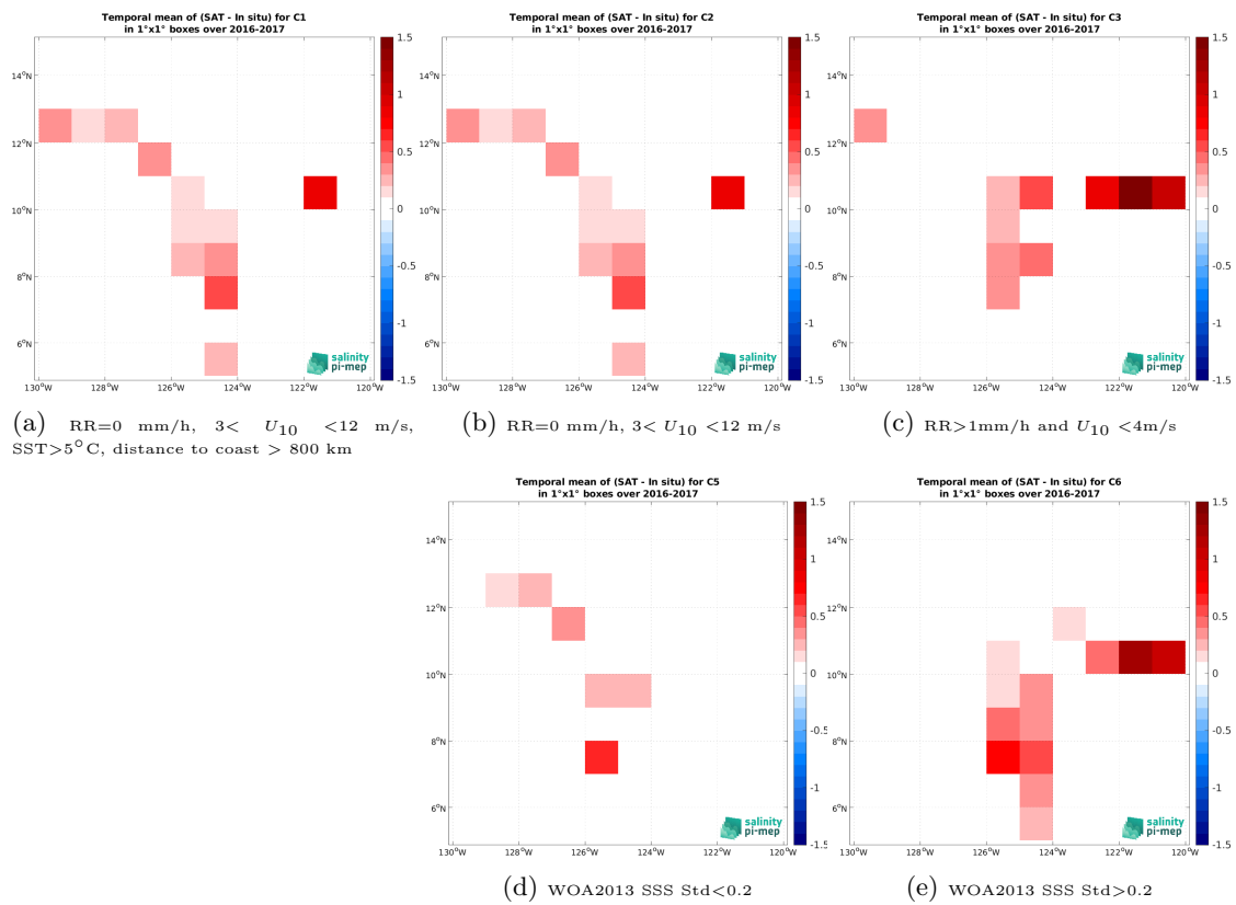
Figure 14: Temporal mean gridded over spatial boxes of size 1^\circ \times 1^\circ of \Delta\text{SSS} (SMAP SSS L4 OI v3 - Monthly (ESR) - Salinity Snake (SPURS 2)) for 5 different subdatasets corresponding to:RR=0 mm/h, 3 < U_{10} < 12 m/s, SST>5°C, distance to coast > 800 km (a), RR=0 mm/h, 3 < U_{10} < 12 m/s (b), RR>1mm/h and U_{10} < 4 m/s (c), WOA2013 SSS Std<0.2 (d), WOA2013 SSS Std>0.2 (e).
