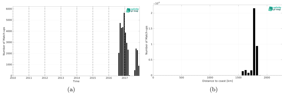
Figure 2: Number of match-ups between Seaglider (SPURS 2) and SMAP SSS L4 OI v3 - Monthly (ESR) SSS as a function of time (a) and as function of the distance to coast (b) over the SPURS 2 Pi-MEP region and for the full satellite product period.
