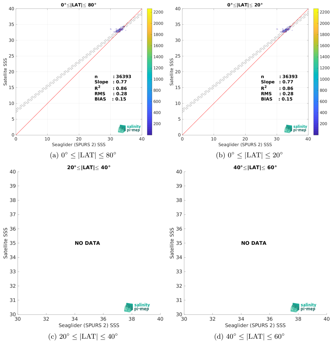
Figure 10: Contour maps of the concentration of SMAP SSS L4 OI v3 - Monthly (ESR) SSS (y-axis) versus Seaglider (SPURS 2) SSS (x-axis) at match-up pairs for different latitude bands. For each plot, the red line shows x=y . The black thin and dashed lines indicate a linear fit through the data cloud and the \pm 95\% confidence levels, respectively. The number match-up pairs n , the slope and R^2 coefficient of the linear fit, the root mean square (RMS) and the mean bias between satellite and in situ data are indicated for each latitude band in each plots.
