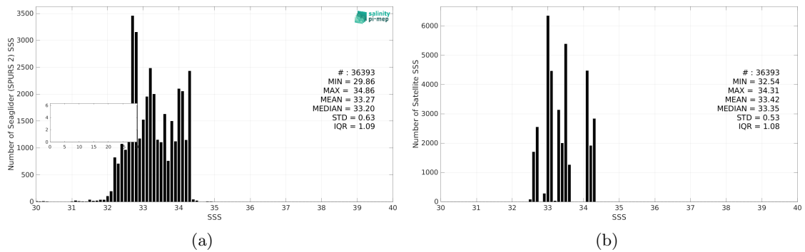
Figure 3: Histograms of SSS from Seaglider (SPURS 2) (a) and SMAP SSS L4 OI v3 - Monthly (ESR) (b) considering all match-up pairs per bins of 0.1 over the SPURS 2 Pi-MEP region and for the full satellite product period.
