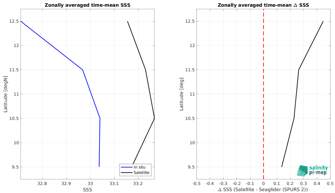
Figure 9: Left panel: Zonal mean SSS from SMAP SSS L4 OI v3 - Monthly (ESR) satellite product (black) and from Seaglider (SPURS 2) (blue). Right panel: Zonal mean of \Delta SSS (Satellite - Seaglider (SPURS 2)) for all the collected Pi-MEP match-up pairs estimated over the full satellite product period.
