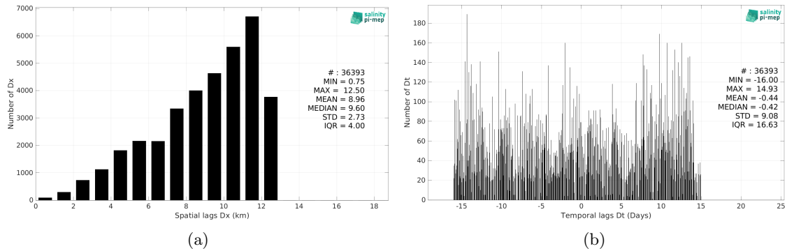
Figure 6: Histograms of the spatial (a) and temporal (b) lags between the location/time of the Seaglider (SPURS 2) measurement and the date of the corresponding SMAP SSS L4 OI v3 - Monthly (ESR) SSS pixel.
