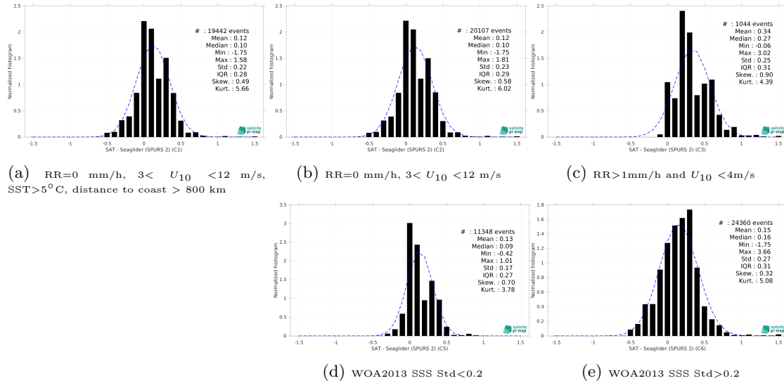
Figure 15: Normalized histogram of \Delta SSS (SMAP SSS L4 OI v3 - Monthly (ESR) - Seaglider (SPURS 2)) for 5 different subdatasets corresponding to: RR=0 mm/h, 3 < U_{10} < 12 m/s, SST>5°C, distance to coast > 800 km (a), RR=0 mm/h, 3 < U_{10} < 12 m/s (b), RR>1mm/h and U_{10} < 4 m/s (c), WOA2013 SSS Std<0.2 (d), WOA2013 SSS Std>0.2 (e).
