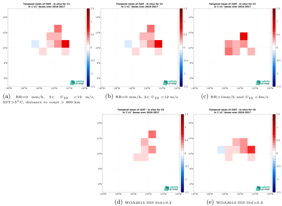
Figure 14: Temporal mean gridded over spatial boxes of size 1^\circ \times 1^\circ of \Delta SSS (SMAP SSS L4 OI v3 - Monthly (ESR) - Seaglider (SPURS 2)) for 5 different subdatasets corresponding to:RR=0 mm/h, 3 < U_{10} < 12 m/s, SST >5^\circ C, distance to coast > 800 km (a), RR=0 mm/h, 3 < U_{10} < 12 m/s (b), RR >1 mm/h and U_{10} < 4 m/s (c), WOA2013 SSS Std <0.2 (d), WOA2013 SSS Std >0.2 (e).
