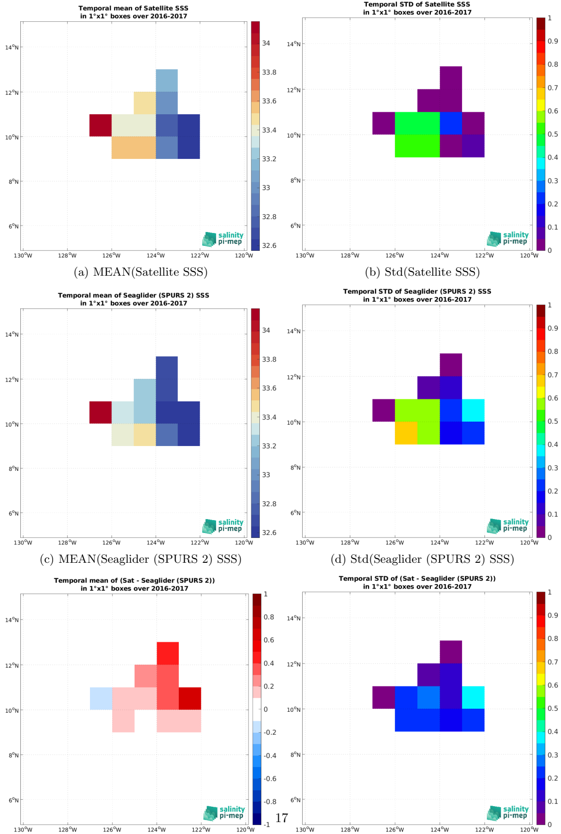
Figure 7: Temporal mean (left) and Std (right) of SSS from SMAP SSS L4 OI v3 - Monthly (ESR) (top), Seaglider (SPURS 2) (middle), and of \Delta SSS (Satellite - Seaglider (SPURS 2)). Only match-up pairs are used to generate these maps.
