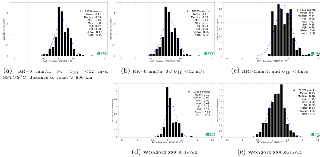
Figure 15: Normalized histogram of \Delta\text{SSS} (SMAP SSS L4 OI v3 - Monthly (ESR) - Seaglider (SPURS 2)) for 5 different subdatasets corresponding to: RR=0 mm/h, 3 < U_{10} < 12 m/s, SST >5^{\circ}\text{C} , distance to coast > 800 km (a), RR=0 mm/h, 3 < U_{10} < 12 m/s (b), RR >1 mm/h and U_{10} < 4 m/s (c), WOA2013 SSS Std <0.2 (d), WOA2013 SSS Std >0.2 (e).
