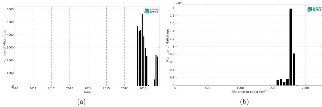
Figure 2: Number of match-ups between Seagliders (SPURS 2) and SMAP SSS L4 OI v3 - Monthly (ESR) SSS as a function of time (a) and as function of the distance to coast (b) over the SPURS 2 Pi-MEP region and for the full satellite product period.
