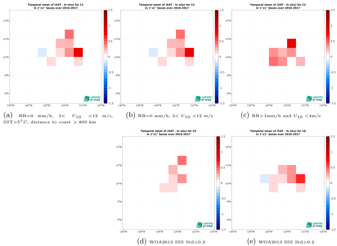
Figure 14: Temporal mean gridded over spatial boxes of size 1^\circ \times 1^\circ of \Delta\text{SSS} (SMAP SSS L4 OI v3 - Monthly (ESR) - Seaglider (SPURS 2)) for 5 different subdatasets corresponding to:RR=0 mm/h, 3 < U_{10} < 12 m/s, SST>5°C, distance to coast > 800 km (a), RR=0 mm/h, 3 < U_{10} < 12 m/s (b), RR>1mm/h and U_{10} < 4 m/s (c), WOA2013 SSS Std<0.2 (d), WOA2013 SSS Std>0.2 (e).
