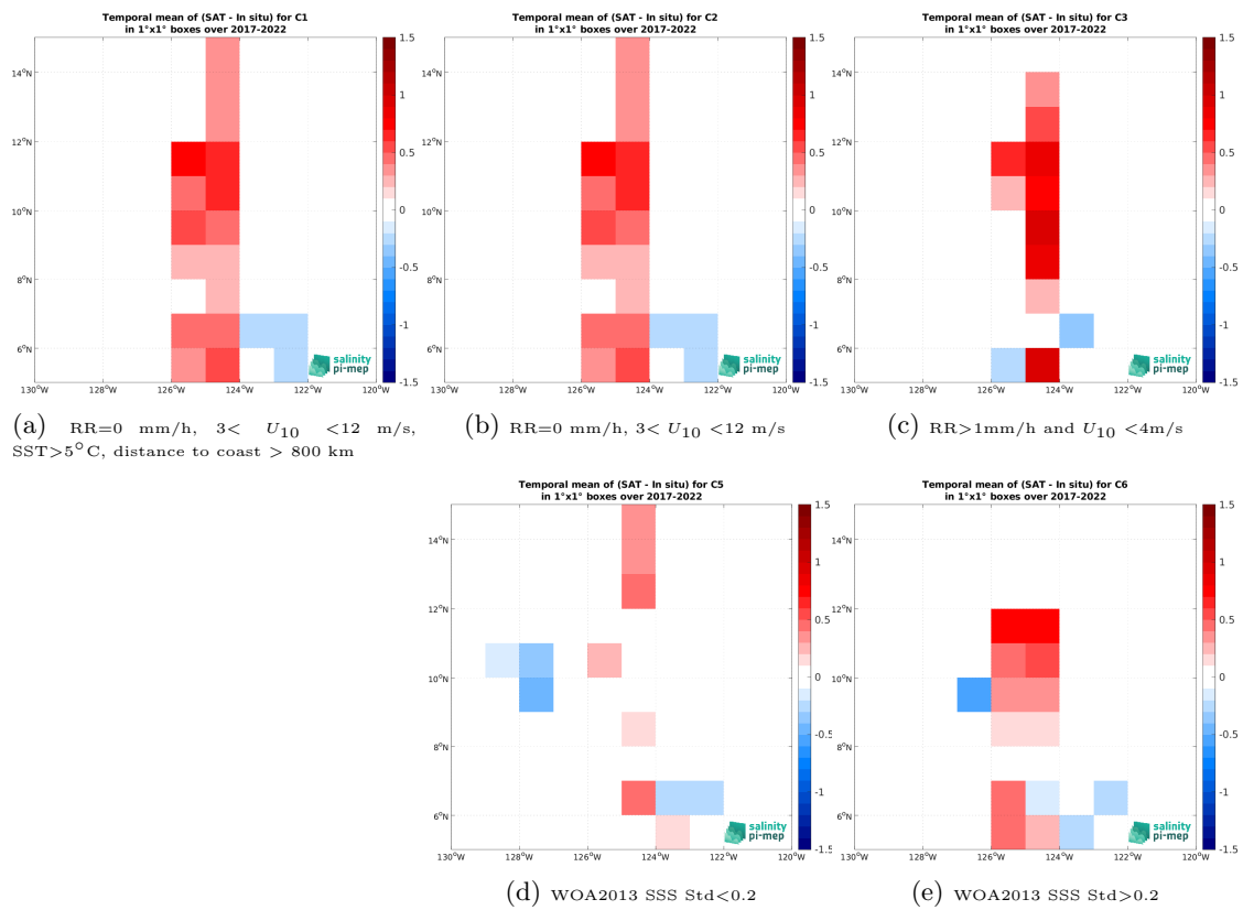
Figure 14: Temporal mean gridded over spatial boxes of size 1^\circ \times 1^\circ of \Delta\text{SSS} (SMAP SSS L4 OI v3 - Monthly (ESR) - Sairdrone) for 5 different subdatasets corresponding to:RR=0 mm/h, 3 < U_{10} < 12 m/s, SST>5°C, distance to coast > 800 km (a), RR=0 mm/h, 3 < U_{10} < 12 m/s (b), RR>1mm/h and U_{10} < 4 m/s (c), WOA2013 SSS Std<0.2 (d), WOA2013 SSS Std>0.2 (e).
