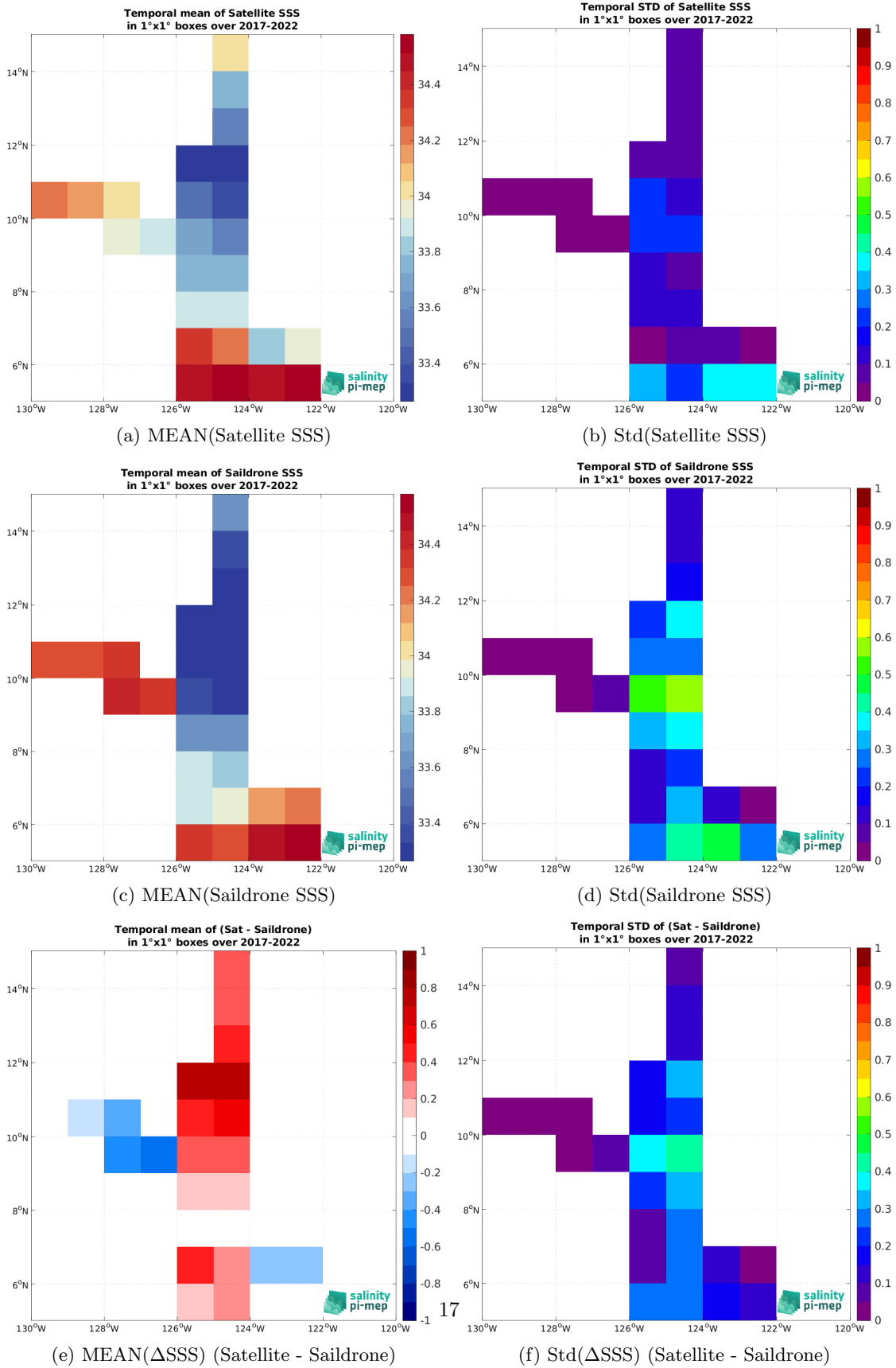
Figure 7: Temporal mean (left) and Std (right) of SSS from SMAP SSS L4 OI v3 - Monthly (ESR) (top), Saildrone (middle), and of \Delta SSS (Satellite - Saildrone). Only match-up pairs are used to generate these maps.
