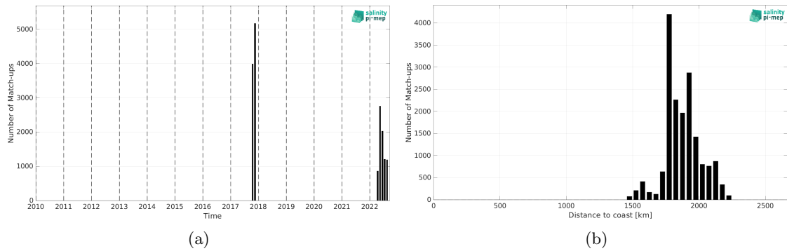
Figure 2: Number of match-ups between Saildrone and SMAP SSS L4 OI v3 - Monthly (ESR) SSS as a function of time (a) and as function of the distance to coast (b) over the SPURS 2 Pi-MEP region and for the full satellite product period.
