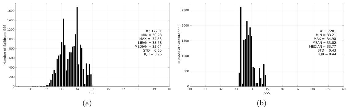
Figure 3: Histograms of SSS from Saildrone (a) and SMAP SSS L4 OI v3 - Monthly (ESR) (b) considering all match-up pairs per bins of 0.1 over the SPURS 2 Pi-MEP region and for the full satellite product period.
