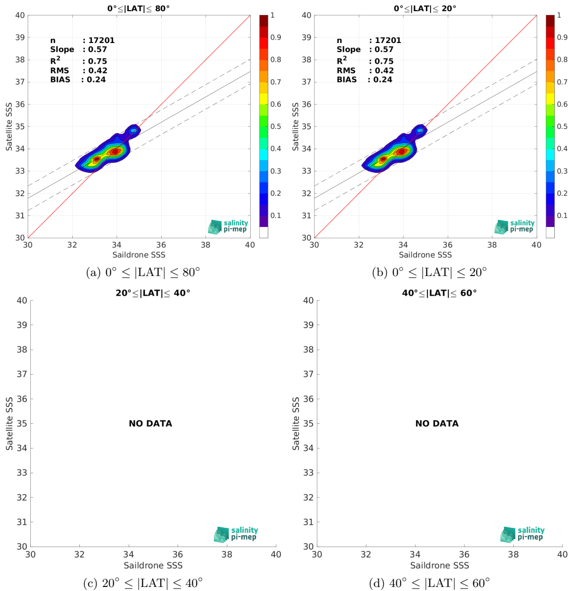
Figure 10: Contour maps of the concentration of SMAP SSS L4 OI v3 - Monthly (ESR) SSS (y-axis) versus Sailldrone SSS (x-axis) at match-up pairs for different latitude bands. For each plot, the red line shows x=y . The black thin and dashed lines indicate a linear fit through the data cloud and the \pm 95\% confidence levels, respectively. The number match-up pairs n , the slope and R^2 coefficient of the linear fit, the root mean square (RMS) and the mean bias between satellite and in situ data are indicated for each latitude band in each plots.
