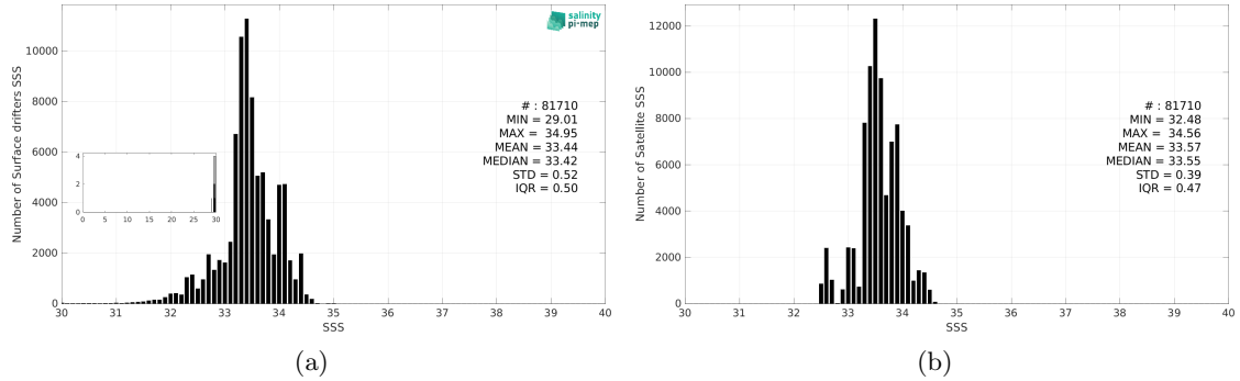
Figure 3: Histograms of SSS from Surface drifters (a) and SMAP SSS L4 OI v3 - Monthly (ESR) (b) considering all match-up pairs per bins of 0.1 over the SPURS 2 Pi-MEP region and for the full satellite product period.
