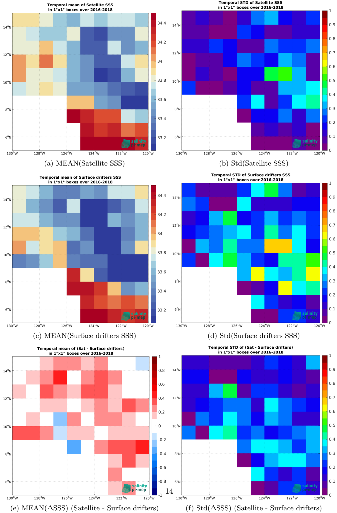
Figure 6: Temporal mean (left) and Std (right) of SSS from SMAP SSS L4 OI v3 - Monthly (ESR) (top), Surface drifters (middle), and of \Delta SSS (Satellite - Surface drifters). Only match-up pairs are used to generate these maps.
