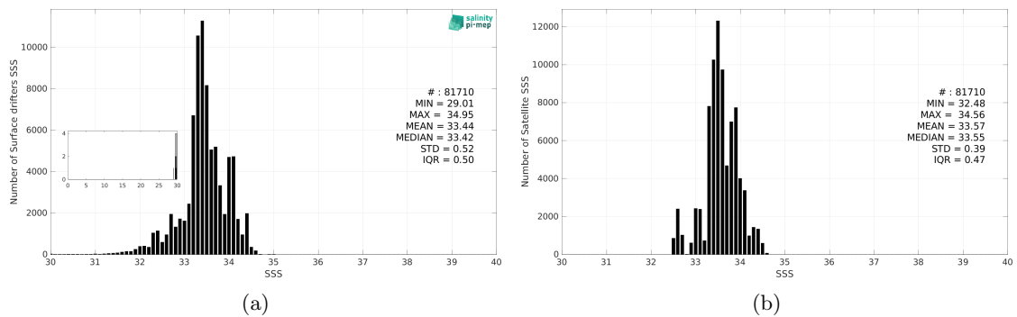
Figure 3: Histograms of SSS from Surface drifters (a) and SMAP SSS L4 OI v3 - Monthly (ESR) (b) considering all match-up pairs per bins of 0.1 over the SPURS 2 Pi-MEP region and for the full satellite product period.
