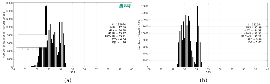
Figure 3: Histograms of SSS from Waveglider (SPURS 2) (a) and SMAP SSS L4 OI v3 - Daily (ESR) (b) considering all match-up pairs per bins of 0.1 over the SPURS 2 Pi-MEP region and for the full satellite product period.
