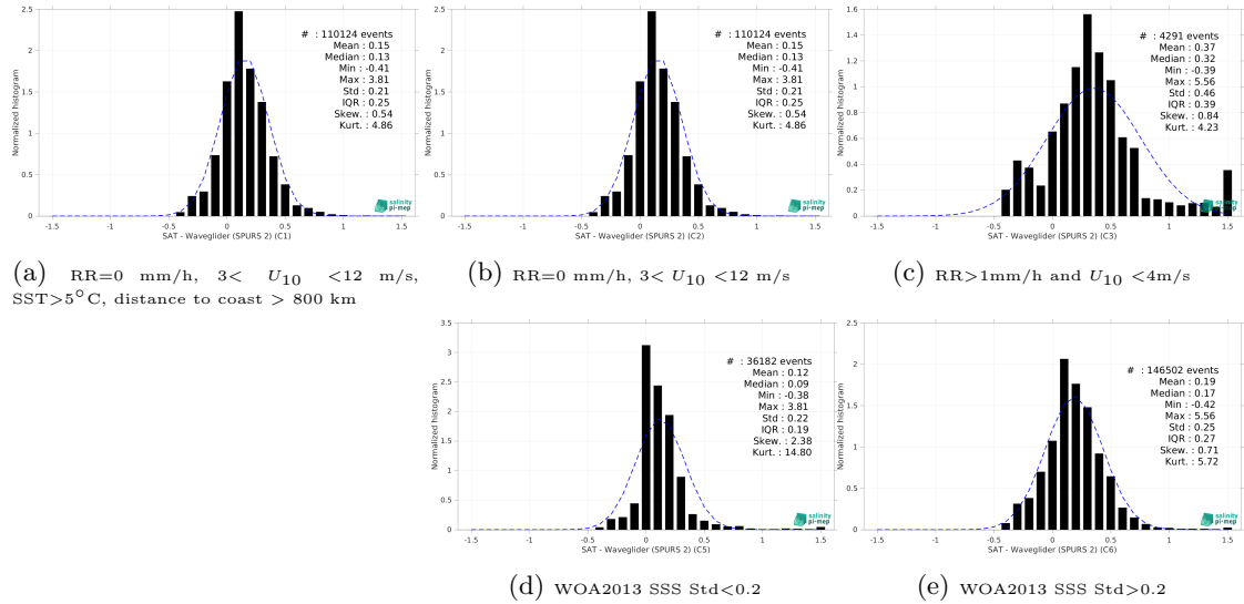
Figure 15: Normalized histogram of \Delta SSS (SMAP SSS L4 OI v3 - Daily (ESR) - Waveglider (SPURS 2)) for 5 different subdatasets corresponding to: RR=0 mm/h, 3 < U_{10} < 12 m/s, SST>5°C, distance to coast > 800 km (a), RR=0 mm/h, 3 < U_{10} < 12 m/s (b), RR>1mm/h and U_{10} < 4 m/s (c), WOA2013 SSS Std<0.2 (d), WOA2013 SSS Std>0.2 (e).
