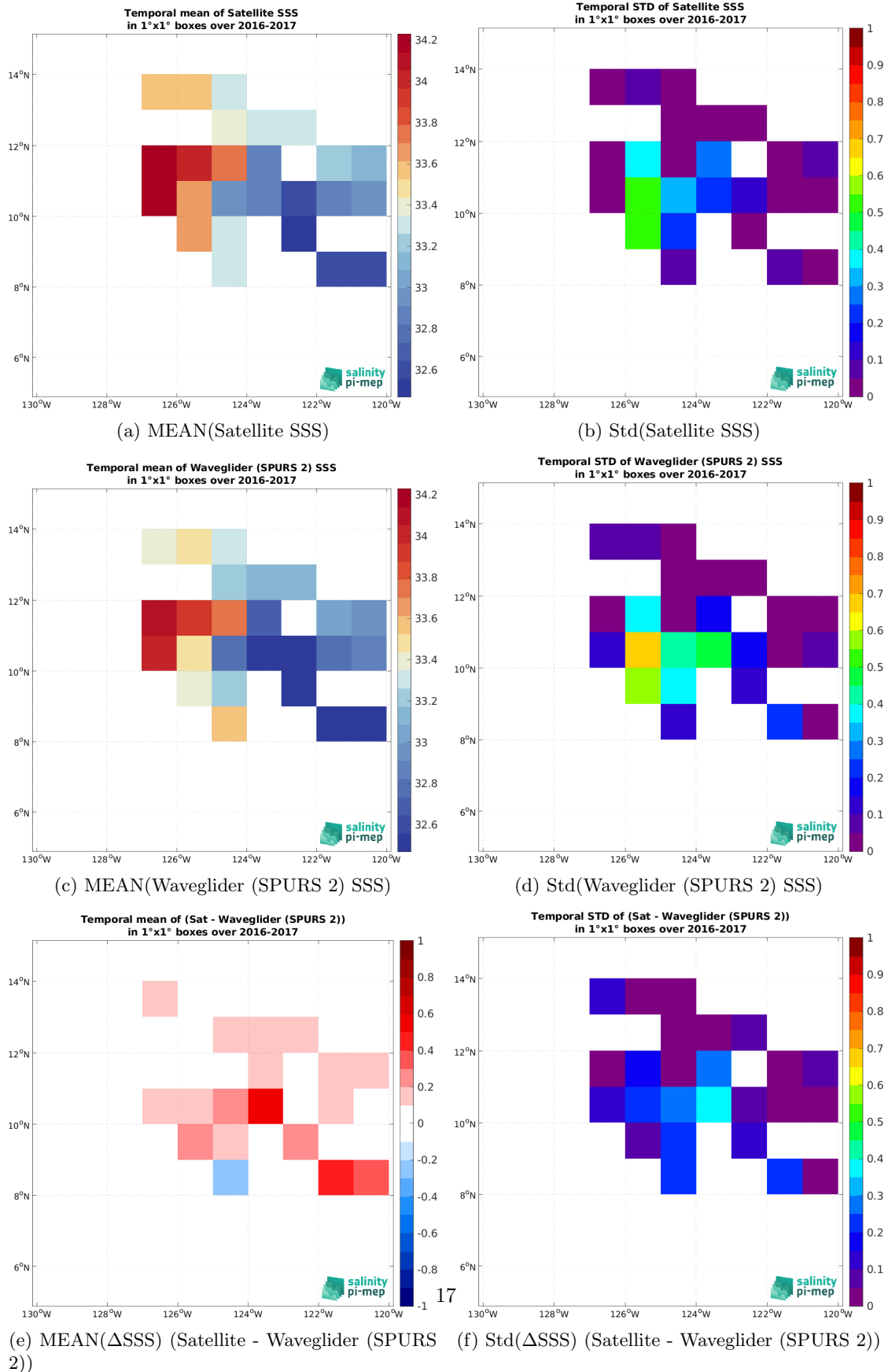
Figure 7: Temporal mean (left) and Std (right) of SSS from SMAP SSS L4 OI v3 - Daily (ESR) (top), Waveglider (SPURS 2) (middle), and of \Delta SSS (Satellite - Waveglider (SPURS 2)). Only match-up pairs are used to generate these maps.
