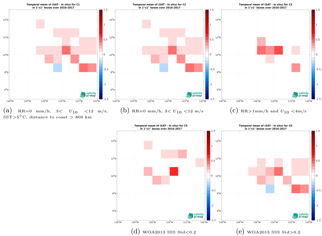
Figure 14: Temporal mean gridded over spatial boxes of size 1^\circ \times 1^\circ of \Delta SSS (SMAP SSS L4 OI v3 - Daily (ESR) - Waveglider (SPURS 2)) for 5 different subdatasets corresponding to:RR=0 mm/h, 3 < U_{10} < 12 m/s, SST >5^\circ C, distance to coast > 800 km (a), RR=0 mm/h, 3 < U_{10} < 12 m/s (b), RR >1 mm/h and U_{10} < 4 m/s (c), WOA2013 SSS Std <0.2 (d), WOA2013 SSS Std >0.2 (e).
