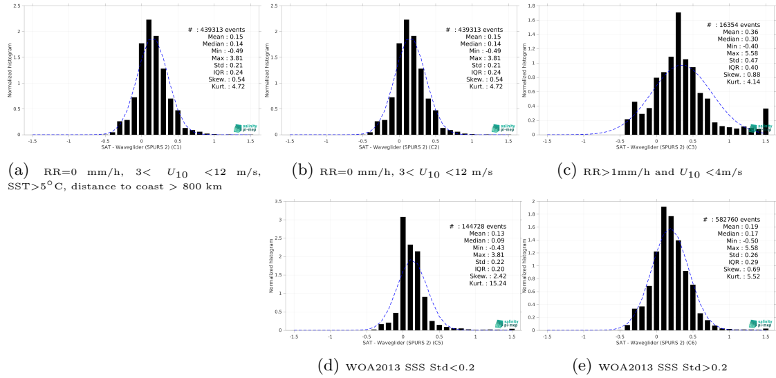
Figure 15: Normalized histogram of \Delta\text{SSS} (SMAP SSS L4 OI v3 - Daily (ESR) - Waveglider (SPURS 2)) for 5 different subdatasets corresponding to: RR=0 mm/h, 3 < U_{10} < 12 m/s, SST>5°C, distance to coast > 800 km (a), RR=0 mm/h, 3 < U_{10} < 12 m/s (b), RR>1mm/h and U_{10} < 4 m/s (c), WOA2013 SSS Std<0.2 (d), WOA2013 SSS Std>0.2 (e).
