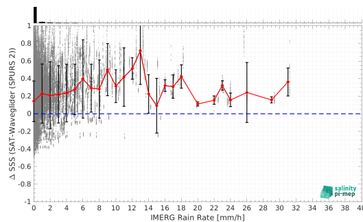
(f) IMERG Rain rate
