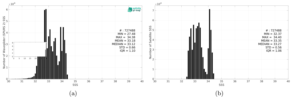
Figure 3: Histograms of SSS from Waveglider (SPURS 2) (a) and SMAP SSS L4 OI v3 - Daily (ESR) (b) considering all match-up pairs per bins of 0.1 over the SPURS 2 Pi-MEP region and for the full satellite product period.
