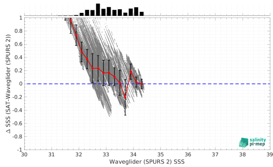
(a) Waveglider (SPURS 2) SSS
