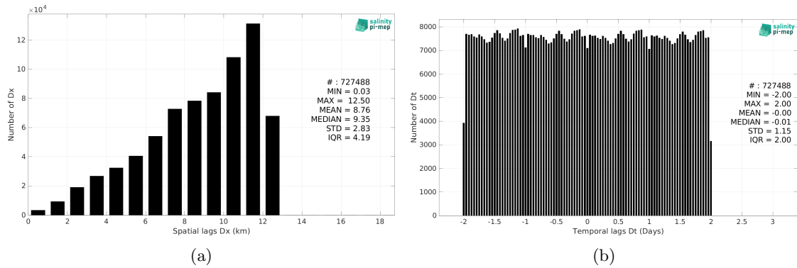
Figure 6: Histograms of the spatial (a) and temporal (b) lags between the location/time of the Waveglider (SPURS 2) measurement and the date of the corresponding SMAP SSS L4 OI v3 - Daily (ESR) SSS pixel.
