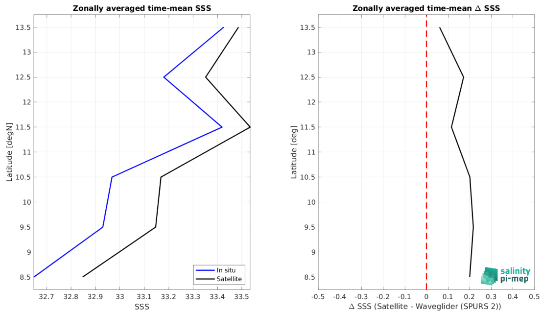
Figure 9: Left panel: Zonal mean SSS from SMAP SSS L4 OI v3 - Daily (ESR) satellite product (black) and from Waveglider (SPURS 2) (blue). Right panel: Zonal mean of \Delta SSS (Satellite - Waveglider (SPURS 2)) for all the collected Pi-MEP match-up pairs estimated over the full satellite product period.
