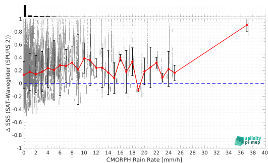
(e) CMORPH Rain rate
