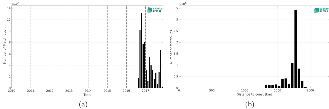
Figure 2: Number of match-ups between Waveglider (SPURS 2) and SMAP SSS L4 OI v3 - Daily (ESR) SSS as a function of time (a) and as function of the distance to coast (b) over the SPURS 2 Pi-MEP region and for the full satellite product period.
