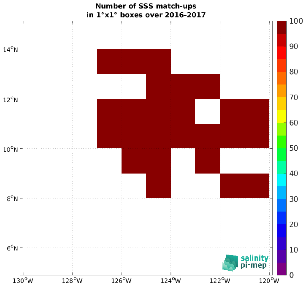
Figure 5: Number of SSS match-ups between Waveglider (SPURS 2) SSS and the SMAP SSS L4 OI v3 - Daily (ESR) SSS product for the SPURS 2 Pi-MEP region over 1^\circ \times 1^\circ boxes and for the full satellite product period.
