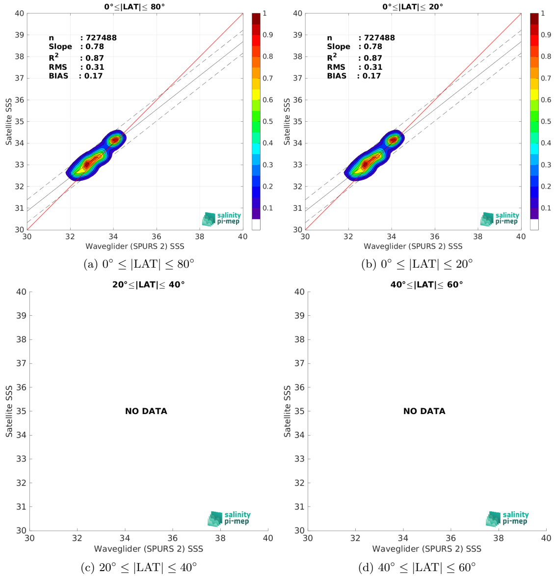
Figure 10: Contour maps of the concentration of SMAP SSS L4 OI v3 - Daily (ESR) SSS (y-axis) versus Waveglider (SPURS 2) SSS (x-axis) at match-up pairs for different latitude bands. For each plot, the red line shows x=y . The black thin and dashed lines indicate a linear fit through the data cloud and the \pm 95\% confidence levels, respectively. The number match-up pairs n , the slope and R^2 coefficient of the linear fit, the root mean square (RMS) and the mean bias between satellite and in situ data are indicated for each latitude band in each plots.
