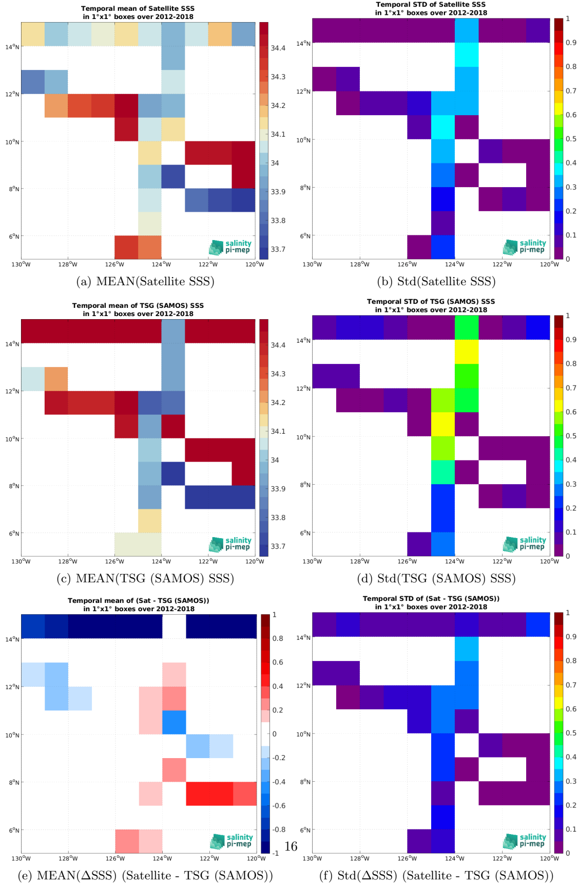
Figure 7: Temporal mean (left) and Std (right) of SSS from SMAP SSS L4 OI v3 - Daily (ESR) (top), TSG (SAMOS) (middle), and of \Delta SSS (Satellite - TSG (SAMOS)). Only match-up pairs are used to generate these maps.
