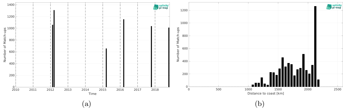
Figure 2: Number of match-ups between TSG (SAMOS) and SMAP SSS L4 OI v3 - Daily (ESR) SSS as a function of time (a) and as function of the distance to coast (b) over the SPURS 2 Pi-MEP region and for the full satellite product period.
