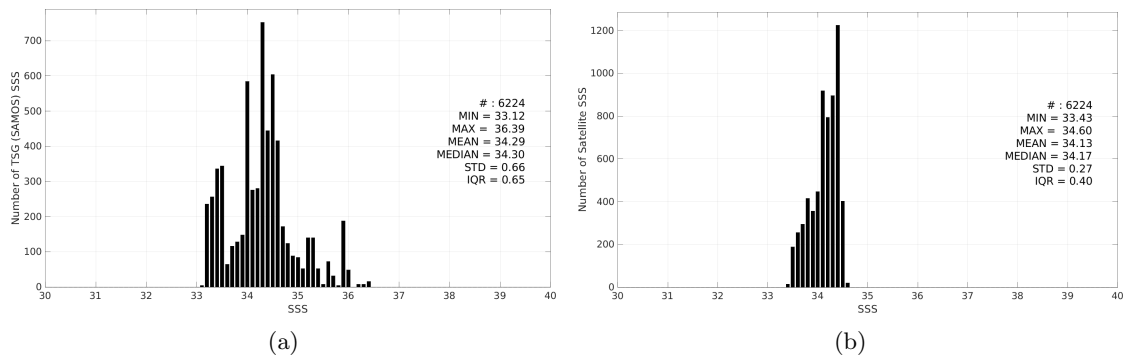
Figure 3: Histograms of SSS from TSG (SAMOS) (a) and SMAP SSS L4 OI v3 - Daily (ESR) (b) considering all match-up pairs per bins of 0.1 over the SPURS 2 Pi-MEP region and for the full satellite product period.
