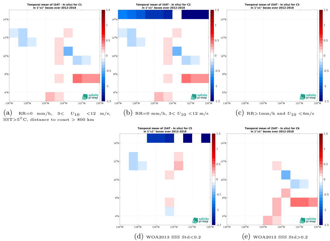
Figure 14: Temporal mean gridded over spatial boxes of size 1^\circ \times 1^\circ of \Delta\text{SSS} (SMAP SSS L4 OI v3 - Daily (ESR) - TSG (SAMOS)) for 5 different subdatasets corresponding to: RR=0 mm/h, 3 < U_{10} < 12 m/s, SST > 5°C, distance to coast > 800 km (a), RR=0 mm/h, 3 < U_{10} < 12 m/s (b), RR > 1mm/h and U_{10} < 4 m/s (c), WOA2013 SSS Std < 0.2 (d), WOA2013 SSS Std > 0.2 (e).
