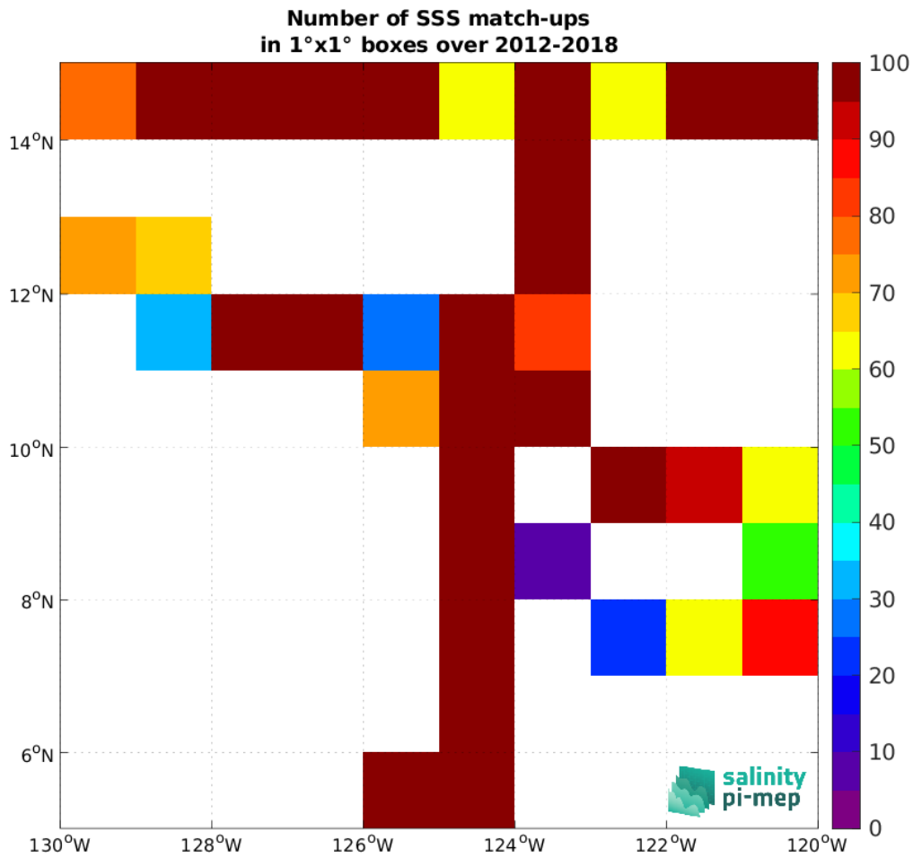
Figure 5: Number of SSS match-ups between TSG (SAMOS) SSS and the SMAP SSS L4 OI v3 - Daily (ESR) SSS product for the SPURS 2 Pi-MEP region over 1^\circ \times 1^\circ boxes and for the full satellite product period.
