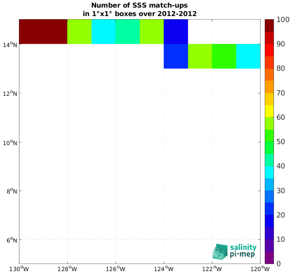
Figure 5: Number of SSS match-ups between TSG (GOSUD-Research-vessel) SSS and the SMAP SSS L4 OI v3 - Daily (ESR) SSS product for the SPURS 2 Pi-MEP region over 1^\circ \times 1^\circ boxes and for the full satellite product period.
