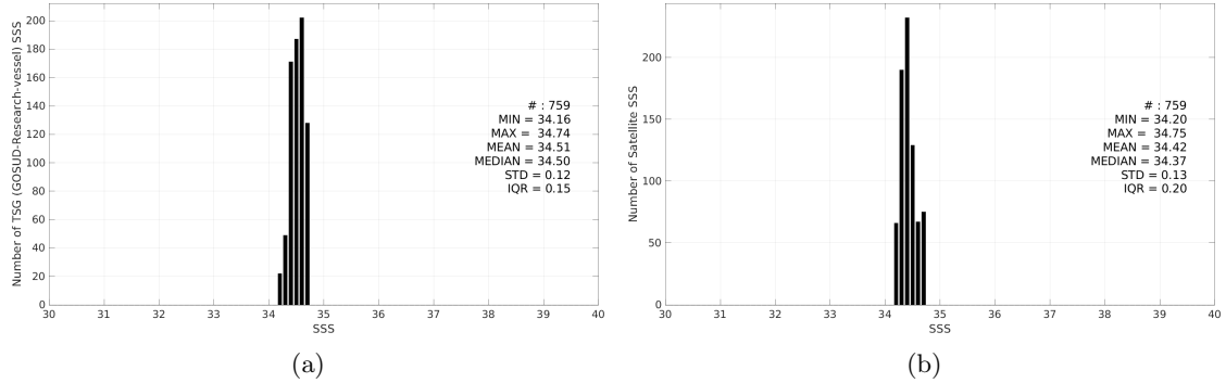
Figure 3: Histograms of SSS from TSG (GOSUD-Research-vessel) (a) and SMAP SSS L4 OI v3 - Daily (ESR) (b) considering all match-up pairs per bins of 0.1 over the SPURS 2 Pi-MEP region and for the full satellite product period.
