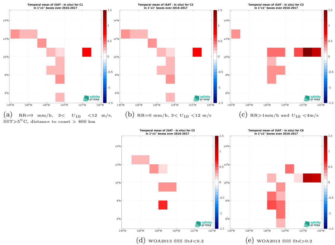
Figure 14: Temporal mean gridded over spatial boxes of size 1^\circ \times 1^\circ of \Delta SSS (SMAP SSS L4 OI v3 - Daily (ESR) - Salinity Snake (SPURS 2)) for 5 different subdatasets corresponding to:RR=0 mm/h, 3 < U_{10} < 12 m/s, SST >5^\circ C, distance to coast > 800 km (a), RR=0 mm/h, 3 < U_{10} < 12 m/s (b), RR >1 mm/h and U_{10} < 4 m/s (c), WOA2013 SSS Std <0.2 (d), WOA2013 SSS Std >0.2 (e).
