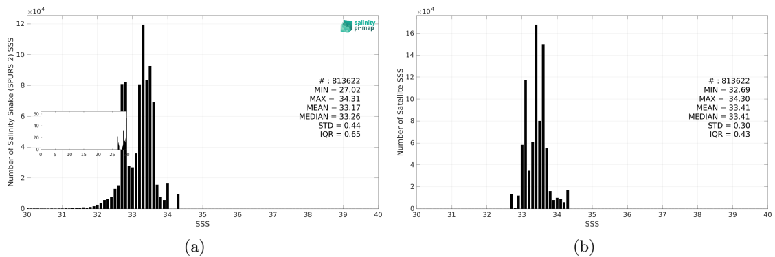
Figure 3: Histograms of SSS from Salinity Snake (SPURS 2) (a) and SMAP SSS L4 OI v3 - Daily (ESR) (b) considering all match-up pairs per bins of 0.1 over the SPURS 2 Pi-MEP region and for the full satellite product period.
