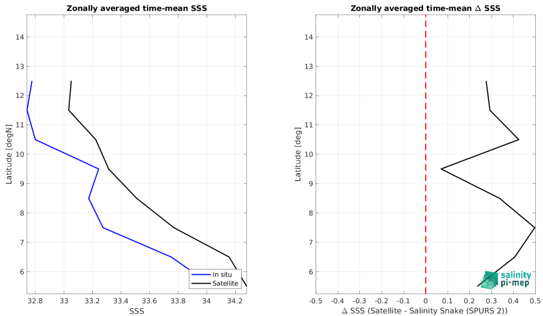
Figure 9: Left panel: Zonal mean SSS from SMAP SSS L4 OI v3 - Daily (ESR) satellite product (black) and from Salinity Snake (SPURS 2) (blue). Right panel: Zonal mean of \Delta SSS (Satellite - Salinity Snake (SPURS 2)) for all the collected Pi-MEP match-up pairs estimated over the full satellite product period.
