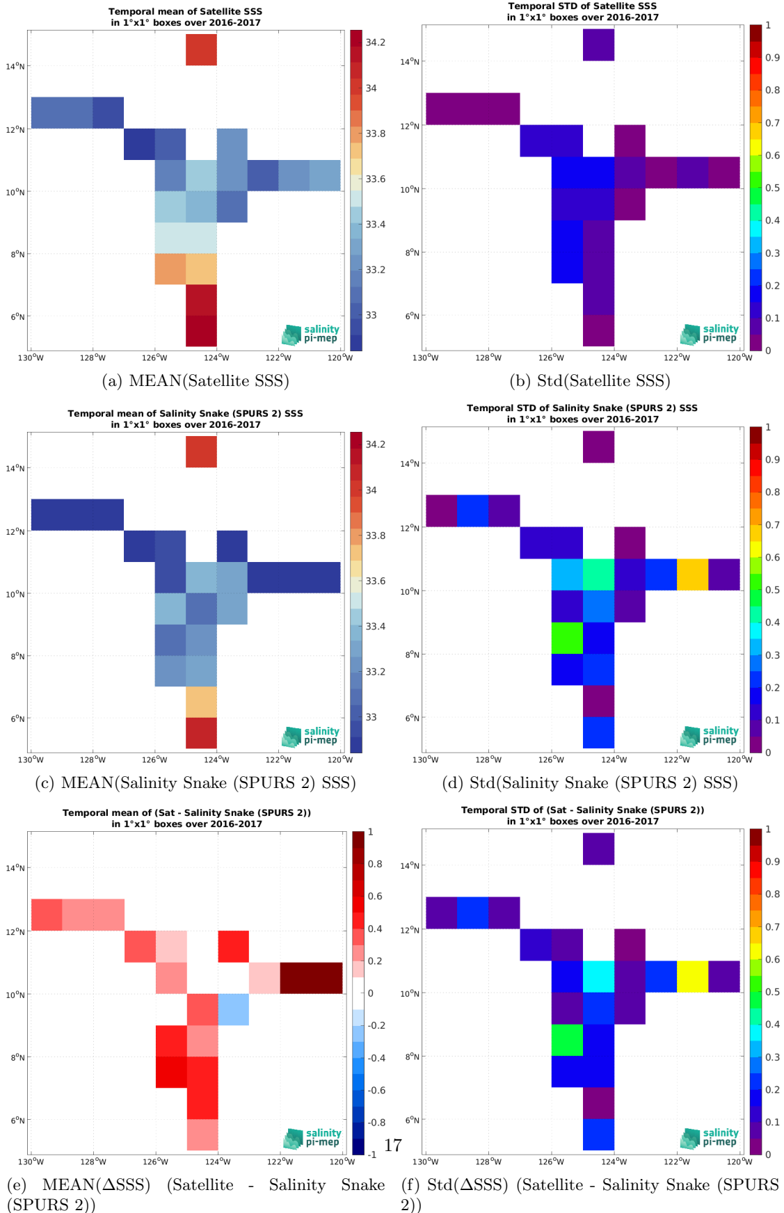
Figure 7: Temporal mean (left) and Std (right) of SSS from SMAP SSS L4 OI v3 - Daily (ESR) (top), Salinity Snake (SPURS 2) (middle), and of \Delta SSS (Satellite - Salinity Snake (SPURS 2)). Only match-up pairs are used to generate these maps.
