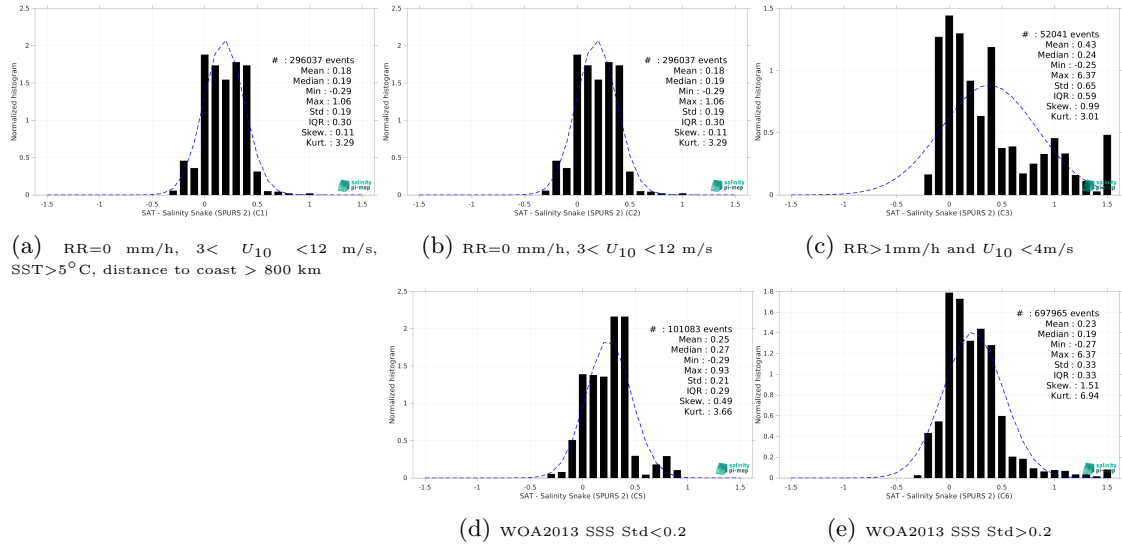
Figure 15: Normalized histogram of \Delta SSS (SMAP SSS L4 OI v3 - Daily (ESR) - Salinity Snake (SPURS 2)) for 5 different subdatasets corresponding to: RR=0 mm/h, 3 < U_{10} < 12 m/s, SST>5°C, distance to coast > 800 km (a), RR=0 mm/h, 3 < U_{10} < 12 m/s (b), RR>1mm/h and U_{10} < 4 m/s (c), WOA2013 SSS Std<0.2 (d), WOA2013 SSS Std>0.2 (e).
