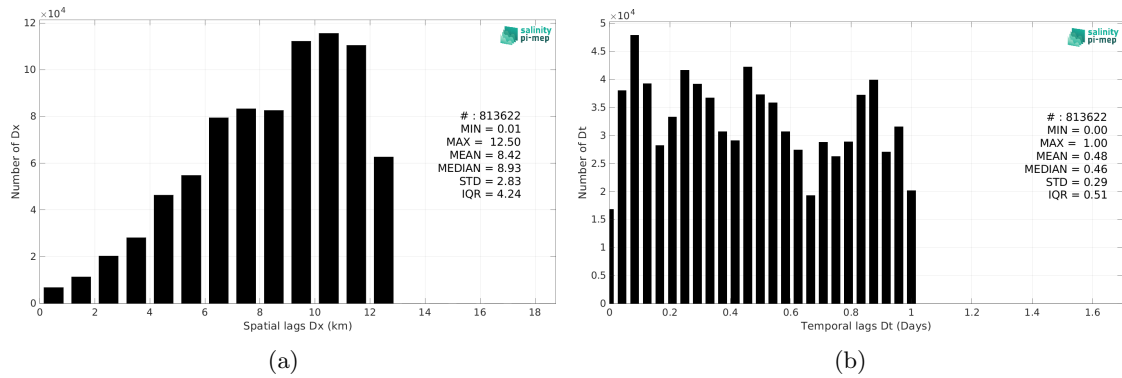
Figure 6: Histograms of the spatial (a) and temporal (b) lags between the location/time of the Salinity Snake (SPURS 2) measurement and the date of the corresponding SMAP SSS L4 OI v3 - Daily (ESR) SSS pixel.
