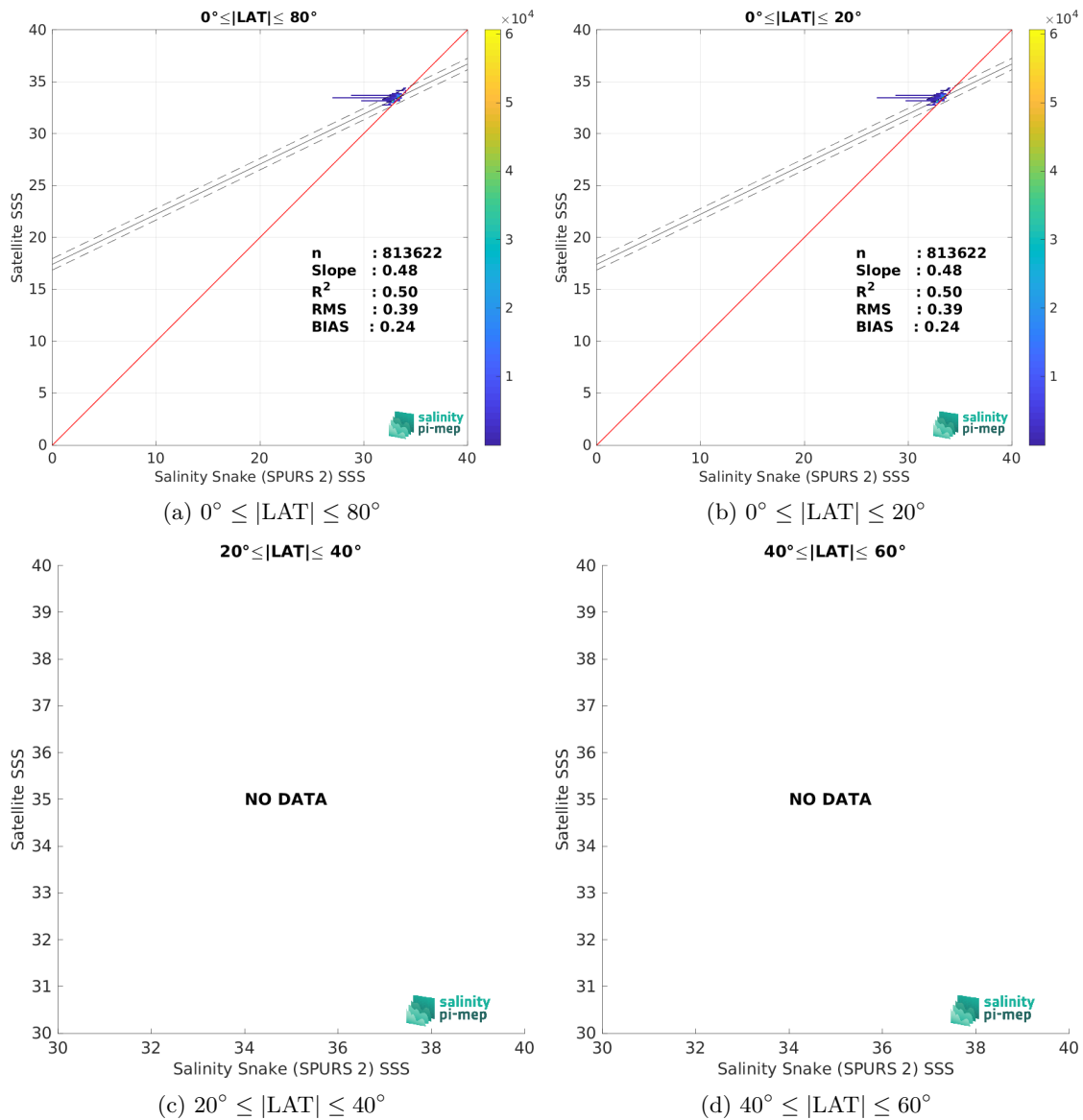
Figure 10: Contour maps of the concentration of SMAP SSS L4 OI v3 - Daily (ESR) SSS (y-axis) versus Salinity Snake (SPURS 2) SSS (x-axis) at match-up pairs for different latitude bands. For each plot, the red line shows x=y . The black thin and dashed lines indicate a linear fit through the data cloud and the \pm 95\% confidence levels, respectively. The number match-up pairs n , the slope and R^2 coefficient of the linear fit, the root mean square (RMS) and the mean bias between satellite and in situ data are indicated for each latitude band in each plots.
