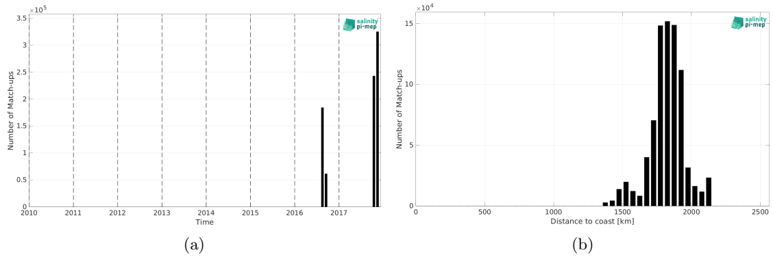
Figure 2: Number of match-ups between Salinity Snake (SPURS 2) and SMAP SSS L4 OI v3 - Daily (ESR) SSS as a function of time (a) and as function of the distance to coast (b) over the SPURS 2 Pi-MEP region and for the full satellite product period.
