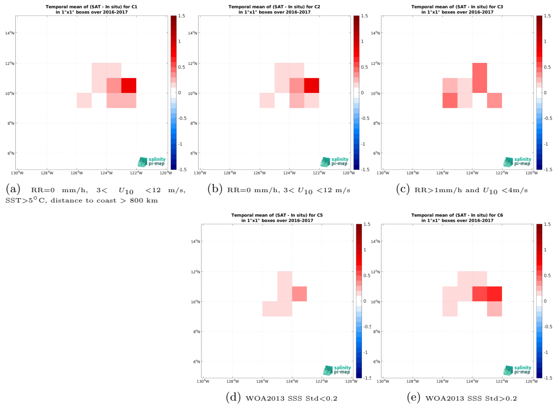
Figure 14: Temporal mean gridded over spatial boxes of size 1^\circ \times 1^\circ of \Delta SSS (SMAP SSS L4 OI v3 - Daily (ESR) - Seaglider (SPURS 2)) for 5 different subdatasets corresponding to:RR=0 mm/h, 3 < U_{10} < 12 m/s, SST > 5°C, distance to coast > 800 km (a), RR=0 mm/h, 3 < U_{10} < 12 m/s (b), RR > 1mm/h and U_{10} < 4 m/s (c), WOA2013 SSS Std < 0.2 (d), WOA2013 SSS Std > 0.2 (e).
