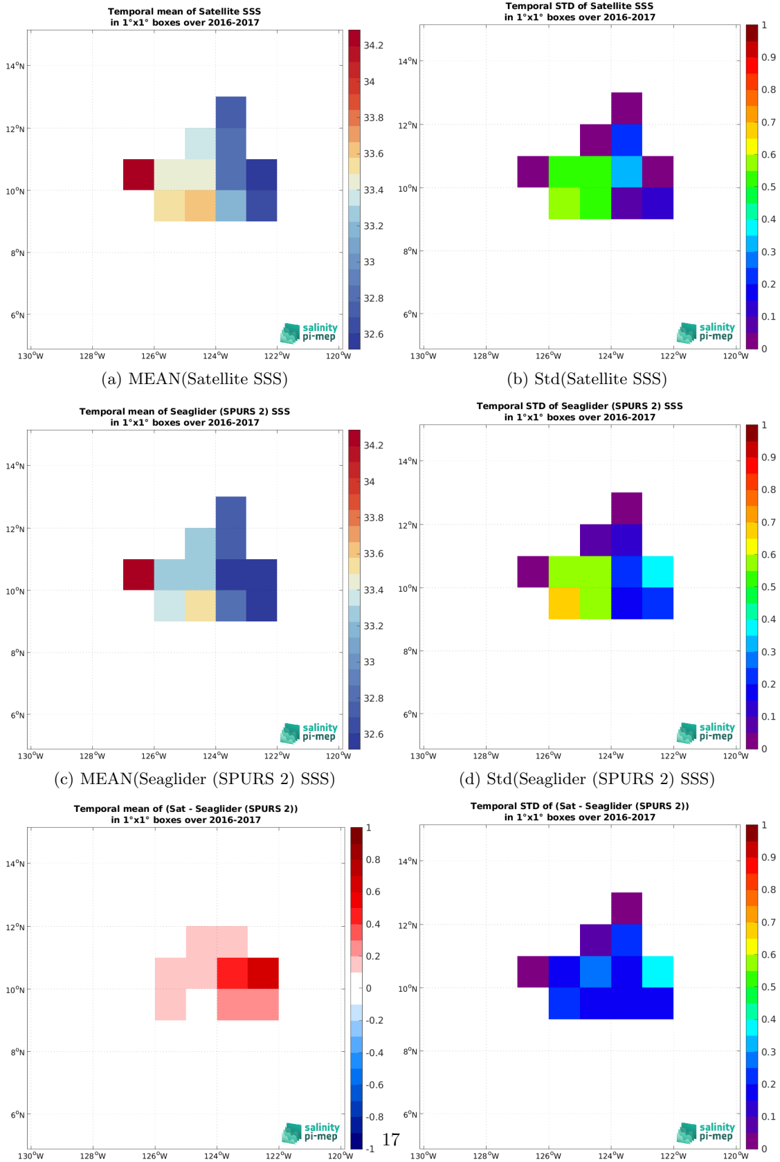
Figure 7: Temporal mean (left) and Std (right) of SSS from SMAP SSS L4 OI v3 - Daily (ESR) (top), Seaglider (SPURS 2) (middle), and of \Delta SSS (Satellite - Seaglider (SPURS 2)). Only match-up pairs are used to generate these maps.
