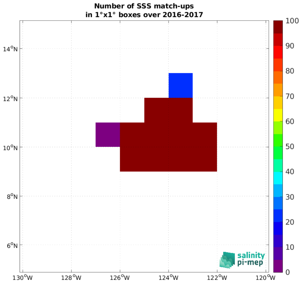
Figure 5: Number of SSS match-ups between Seagliders (SPURS 2) SSS and the SMAP SSS L4 OI v3 - Daily (ESR) SSS product for the SPURS 2 Pi-MEP region over 1^\circ \times 1^\circ boxes and for the full satellite product period.
