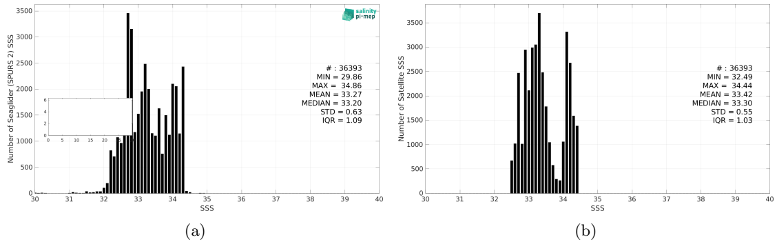
Figure 3: Histograms of SSS from Seaglider (SPURS 2) (a) and SMAP SSS L4 OI v3 - Daily (ESR) (b) considering all match-up pairs per bins of 0.1 over the SPURS 2 Pi-MEP region and for the full satellite product period.
