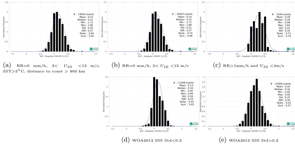
Figure 15: Normalized histogram of \Delta SSS (SMAP SSS L4 OI v3 - Daily (ESR) - Seaglider (SPURS 2)) for 5 different subdatasets corresponding to: RR=0 mm/h, 3 < U_{10} < 12 m/s, SST>5°C, distance to coast > 800 km (a), RR=0 mm/h, 3 < U_{10} < 12 m/s (b), RR>1mm/h and U_{10} < 4 m/s (c), WOA2013 SSS Std<0.2 (d), WOA2013 SSS Std>0.2 (e).
