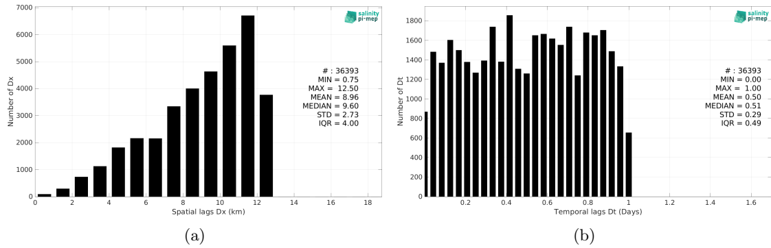
Figure 6: Histograms of the spatial (a) and temporal (b) lags between the location/time of the Seaglider (SPURS 2) measurement and the date of the corresponding SMAP SSS L4 OI v3 - Daily (ESR) SSS pixel.
