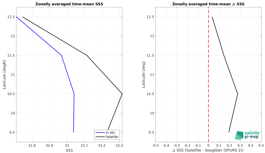
Figure 9: Left panel: Zonal mean SSS from SMAP SSS L4 OI v3 - Daily (ESR) satellite product (black) and from Seaglider (SPURS 2) (blue). Right panel: Zonal mean of \Delta SSS (Satellite - Seaglider (SPURS 2)) for all the collected Pi-MEP match-up pairs estimated over the full satellite product period.
