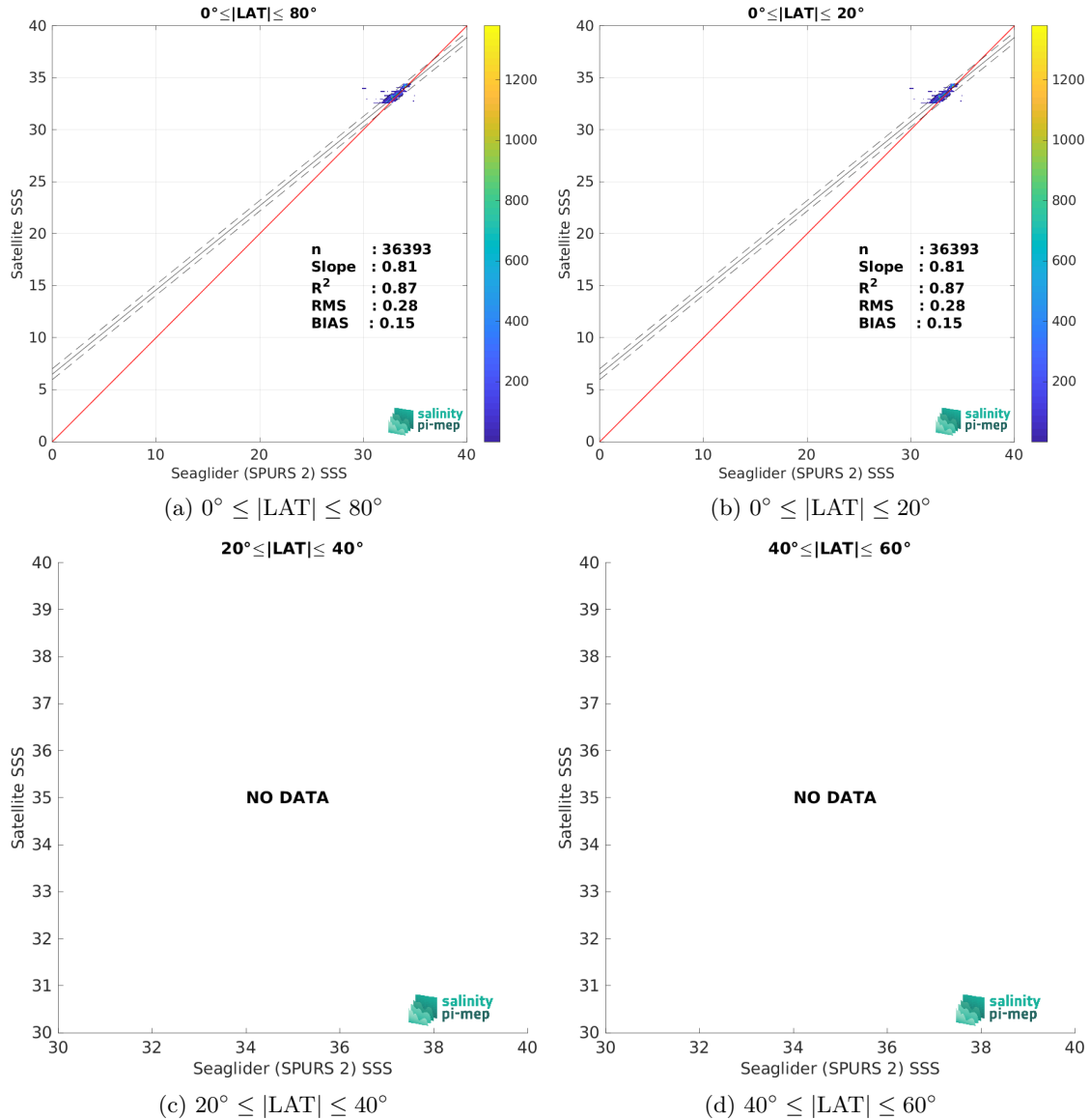
Figure 10: Contour maps of the concentration of SMAP SSS L4 OI v3 - Daily (ESR) SSS (y-axis) versus Seaglider (SPURS 2) SSS (x-axis) at match-up pairs for different latitude bands. For each plot, the red line shows x=y . The black thin and dashed lines indicate a linear fit through the data cloud and the \pm 95\% confidence levels, respectively. The number match-up pairs n , the slope and R^2 coefficient of the linear fit, the root mean square (RMS) and the mean bias between satellite and in situ data are indicated for each latitude band in each plots.
