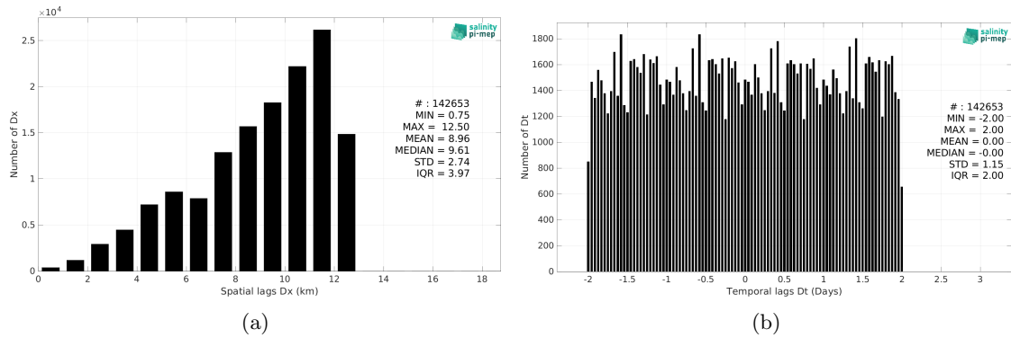
Figure 6: Histograms of the spatial (a) and temporal (b) lags between the location/time of the Seaglider (SPURS 2) measurement and the date of the corresponding SMAP SSS L4 OI v3 - Daily (ESR) SSS pixel.
