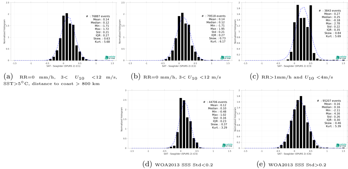
Figure 15: Normalized histogram of \Delta SSS (SMAP SSS L4 OI v3 - Daily (ESR) - Seaglider (SPURS 2)) for 5 different subdatasets corresponding to: RR=0 mm/h, 3 < U_{10} < 12 m/s, SST > 5°C, distance to coast > 800 km (a), RR=0 mm/h, 3 < U_{10} < 12 m/s (b), RR > 1mm/h and U_{10} < 4 m/s (c), WOA2013 SSS Std < 0.2 (d), WOA2013 SSS Std > 0.2 (e).
