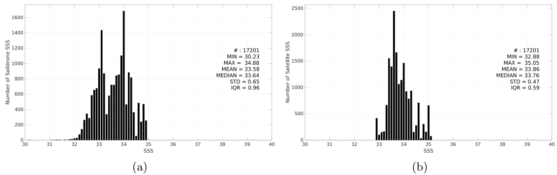
Figure 3: Histograms of SSS from Saildrone (a) and SMAP SSS L4 OI v3 - Daily (ESR) (b) considering all match-up pairs per bins of 0.1 over the SPURS 2 Pi-MEP region and for the full satellite product period.
