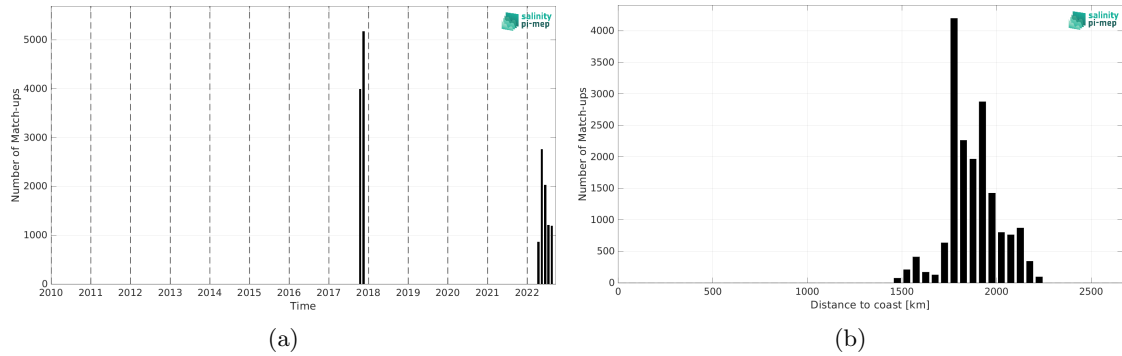
Figure 2: Number of match-ups between Saildrone and SMAP SSS L4 OI v3 - Daily (ESR) SSS as a function of time (a) and as function of the distance to coast (b) over the SPURS 2 Pi-MEP region and for the full satellite product period.
