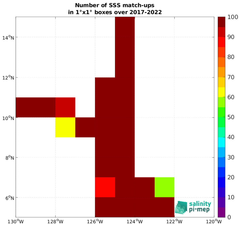
Figure 5: Number of SSS match-ups between Saildrone SSS and the SMAP SSS L4 OI v3 - Daily (ESR) SSS product for the SPURS 2 Pi-MEP region over 1^\circ \times 1^\circ boxes and for the full satellite product period.
