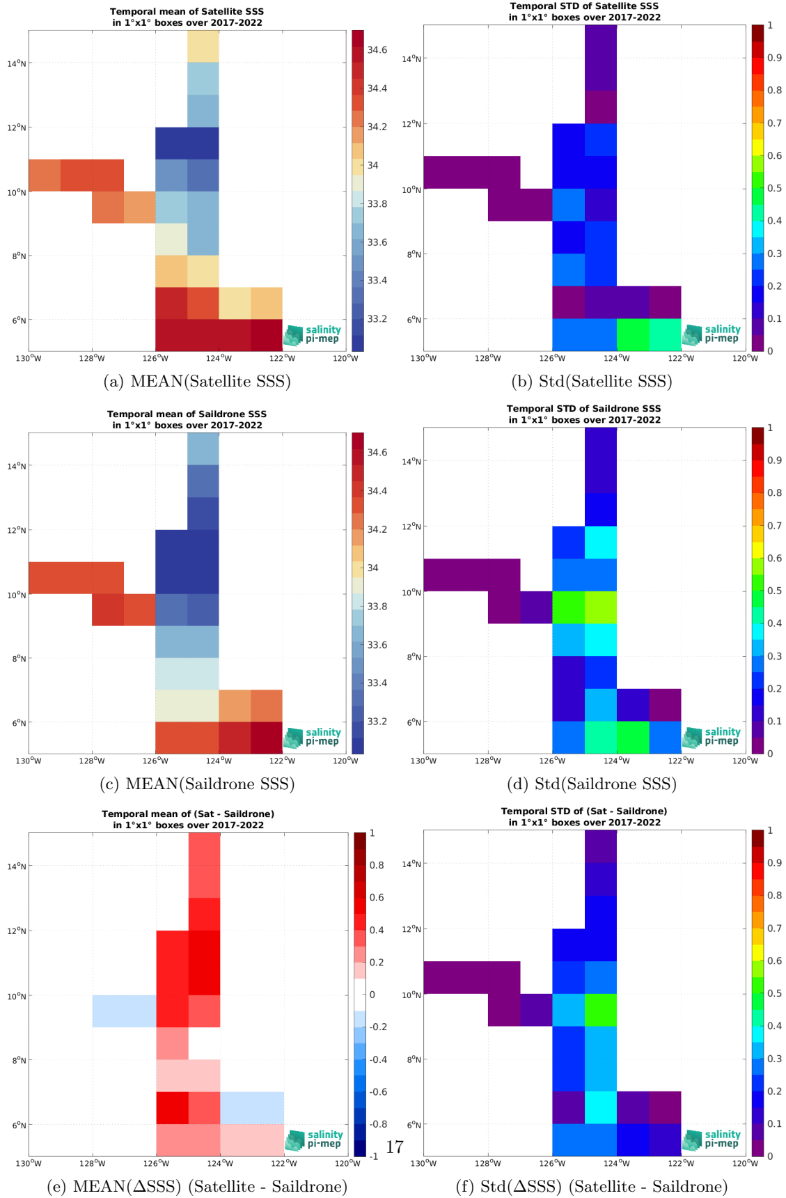
Figure 7: Temporal mean (left) and Std (right) of SSS from SMAP SSS L4 OI v3 - Daily (ESR) (top), Saildrone (middle), and of \Delta SSS (Satellite - Saildrone). Only match-up pairs are used to generate these maps.
