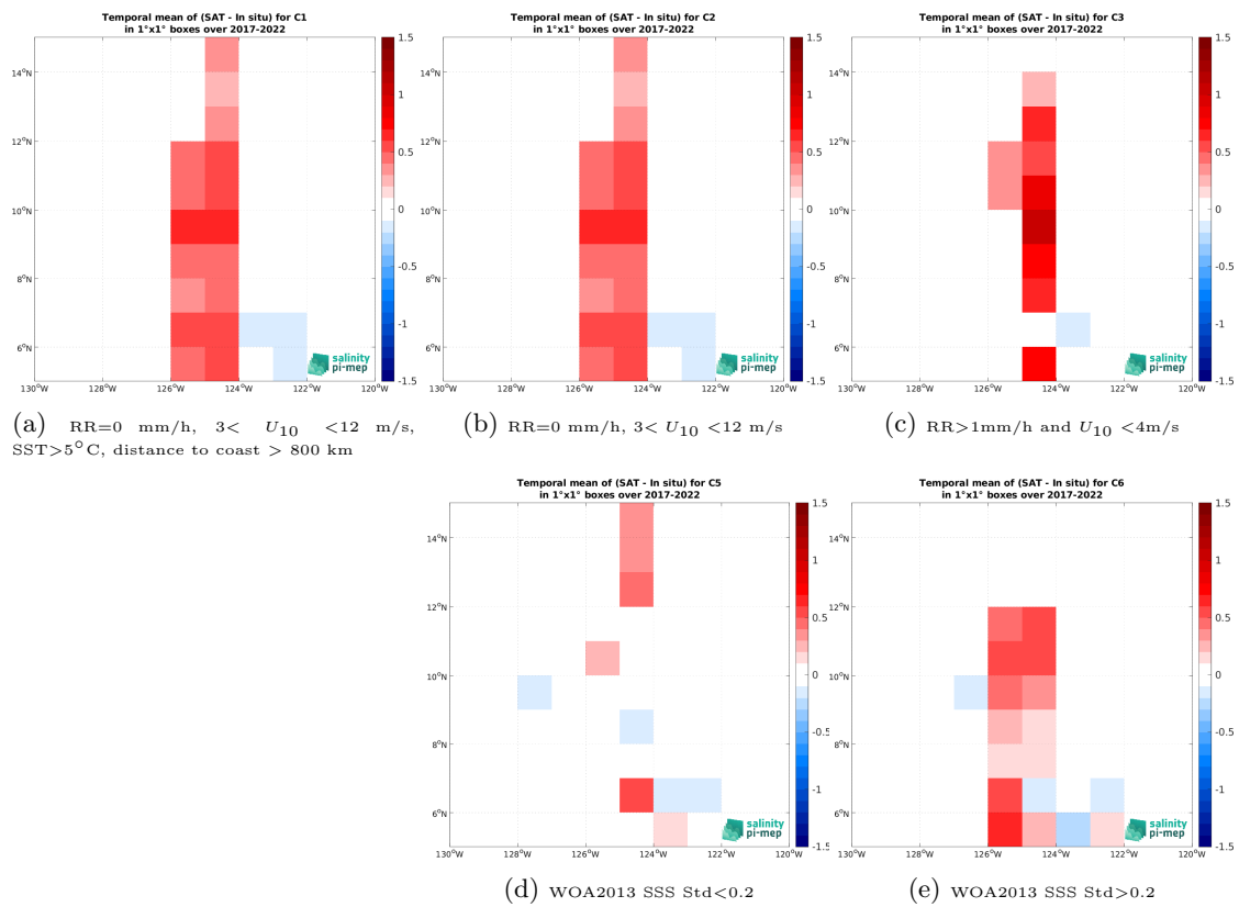
Figure 14: Temporal mean gridded over spatial boxes of size 1^\circ \times 1^\circ of \Delta SSS (SMAP SSS L4 OI v3 - Daily (ESR) - Saildrone) for 5 different subdatasets corresponding to:RR=0 mm/h, 3 < U_{10} < 12 m/s, SST > 5^\circ\text{C} , distance to coast > 800 km (a), RR=0 mm/h, 3 < U_{10} < 12 m/s (b), RR > 1 mm/h and U_{10} < 4 m/s (c), WOA2013 SSS Std < 0.2 (d), WOA2013 SSS Std > 0.2 (e).
