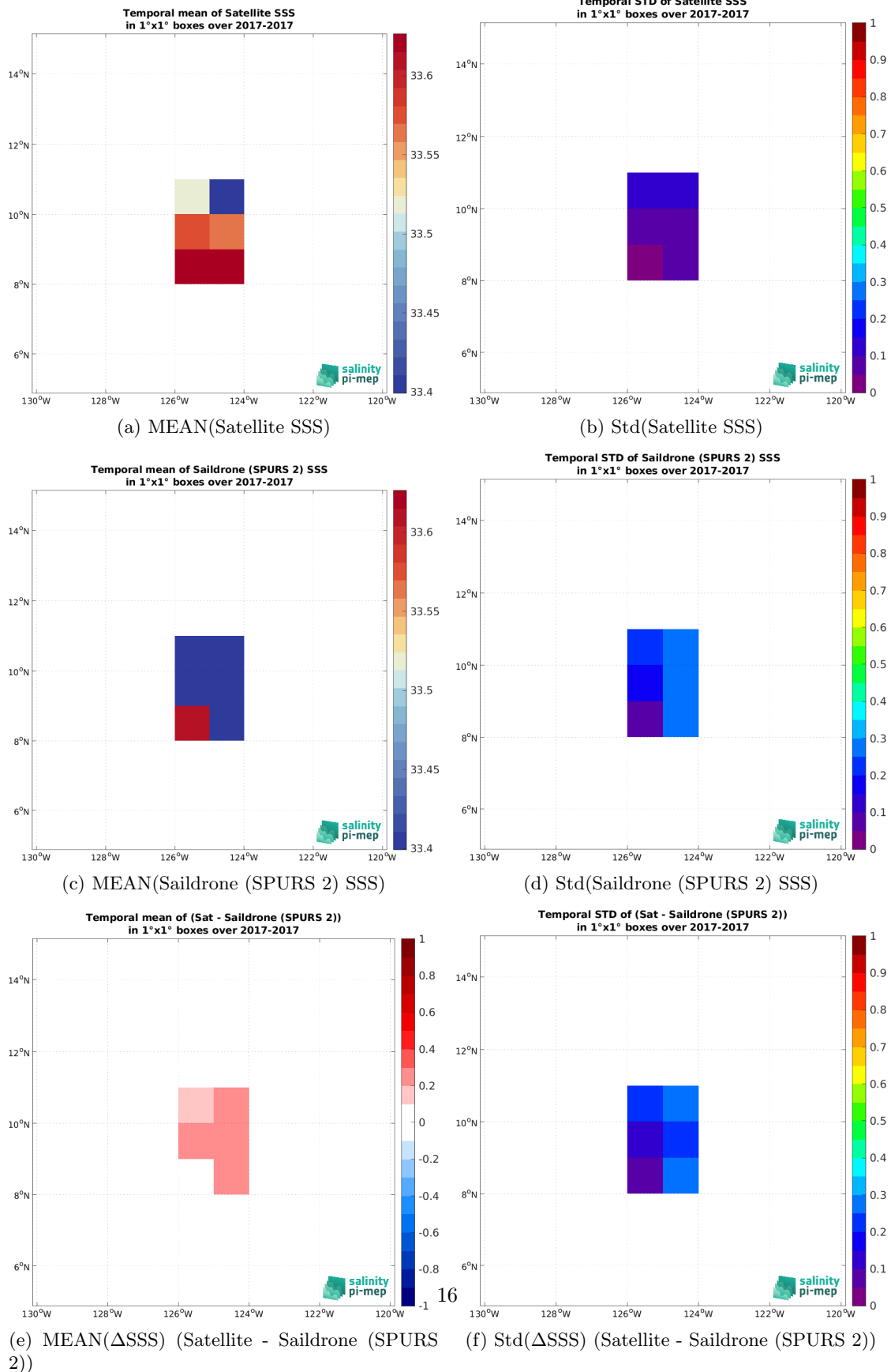
Figure 7: Temporal mean (left) and Std (right) of SSS from SMAP SSS L4 OI v3 - Daily (ESR) (top), Saildrone (SPURS 2) (middle), and of \Delta SSS (Satellite - Saildrone (SPURS 2)). Only match-up pairs are used to generate these maps.
