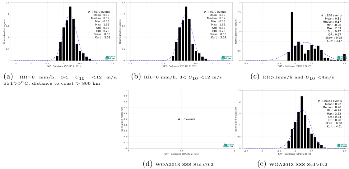
Figure 15: Normalized histogram of \Delta\text{SSS} (SMAP SSS L4 OI v3 - Daily (ESR) - Sailability (SPURS 2)) for 5 different subdatasets corresponding to: RR=0 mm/h, 3 < U_{10} < 12 m/s, SST>5°C, distance to coast > 800 km (a), RR=0 mm/h, 3 < U_{10} < 12 m/s (b), RR>1mm/h and U_{10} < 4 m/s (c), WOA2013 SSS Std<0.2 (d), WOA2013 SSS Std>0.2 (e).
