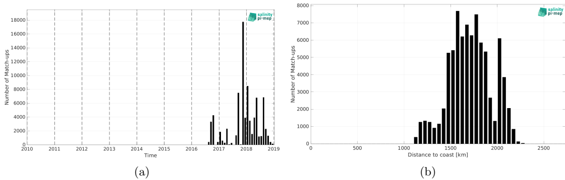
Figure 2: Number of match-ups between Surface drifters and SMAP SSS L4 OI v3 - Daily (ESR) SSS as a function of time (a) and as function of the distance to coast (b) over the SPURS 2 Pi-MEP region and for the full satellite product period.
