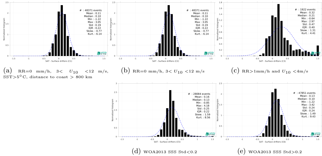
Figure 14: Normalized histogram of \Delta SSS (SMAP SSS L4 OI v3 - Daily (ESR) - Surface drifters) for 5 different subdatasets corresponding to: RR=0 mm/h, 3 < U_{10} < 12 m/s, SST >5^{\circ} C, distance to coast > 800 km (a), RR=0 mm/h, 3 < U_{10} < 12 m/s (b), RR >1 mm/h and U_{10} < 4 m/s (c), WOA2013 SSS Std <0.2 (d), WOA2013 SSS Std >0.2 (e).
