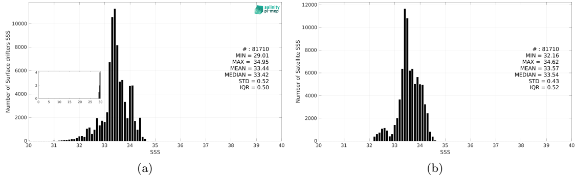
Figure 3: Histograms of SSS from Surface drifters (a) and SMAP SSS L4 OI v3 - Daily (ESR) (b) considering all match-up pairs per bins of 0.1 over the SPURS 2 Pi-MEP region and for the full satellite product period.
