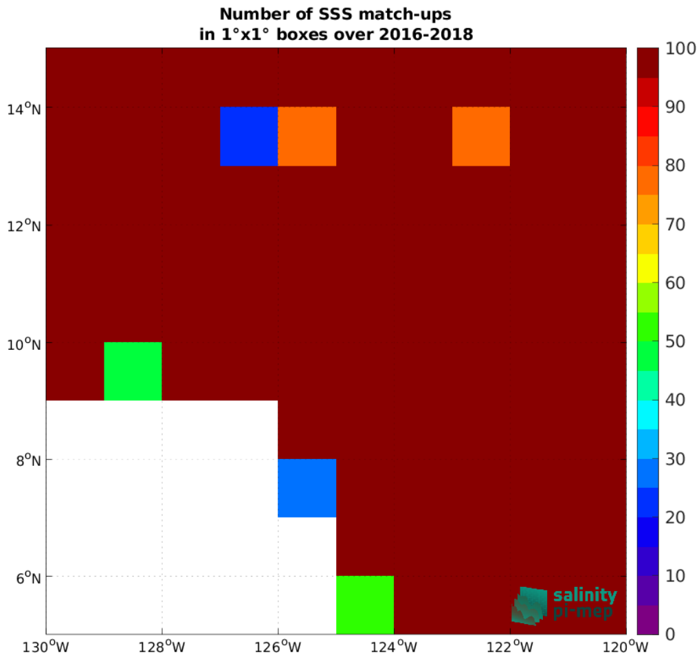
Figure 4: Number of SSS match-ups between Surface drifters SSS and the SMAP SSS L4 OI v3 - Daily (ESR) SSS product for the SPURS 2 Pi-MEP region over 1°x1° boxes and for the full satellite product period.
