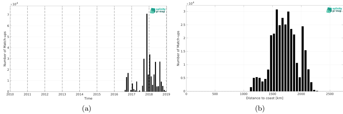
Figure 2: Number of match-ups between Surface drifters and SMAP SSS L4 OI v3 - Daily (ESR) SSS as a function of time (a) and as function of the distance to coast (b) over the SPURS 2 Pi-MEP region and for the full satellite product period.
