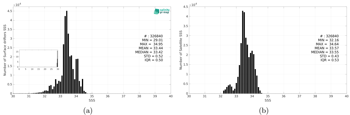
Figure 3: Histograms of SSS from Surface drifters (a) and SMAP SSS L4 OI v3 - Daily (ESR) (b) considering all match-up pairs per bins of 0.1 over the SPURS 2 Pi-MEP region and for the full satellite product period.
