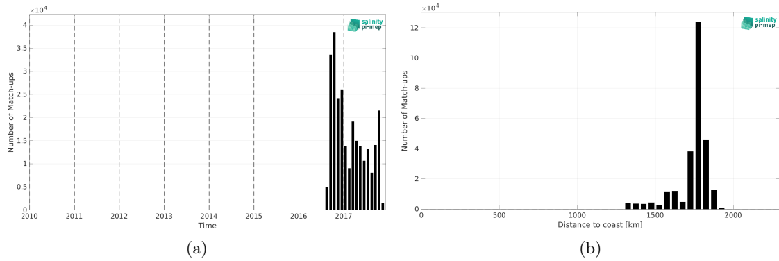
Figure 1: Number of match-ups between Waveglider (SPURS 2) and SMAP SSS L4 OI v2 - 7 Days (ESR) SSS as a function of time (a) and as function of the distance to coast (b) over the SPURS 2 Pi-MEP region and for the full satellite product period.
