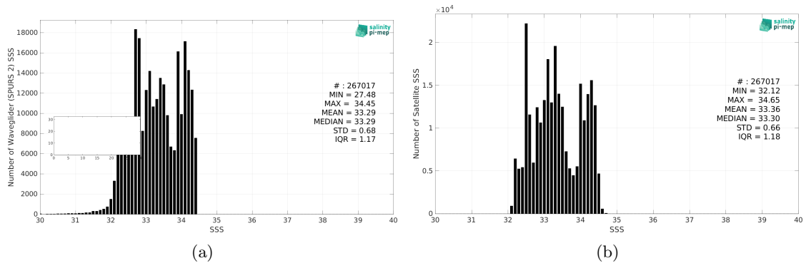
Figure 2: Histograms of SSS from Waveglider (SPURS 2) (a) and SMAP SSS L4 OI v2 - 7 Days (ESR) (b) considering all match-up pairs per bins of 0.1 over the SPURS 2 Pi-MEP region and for the full satellite product period.
