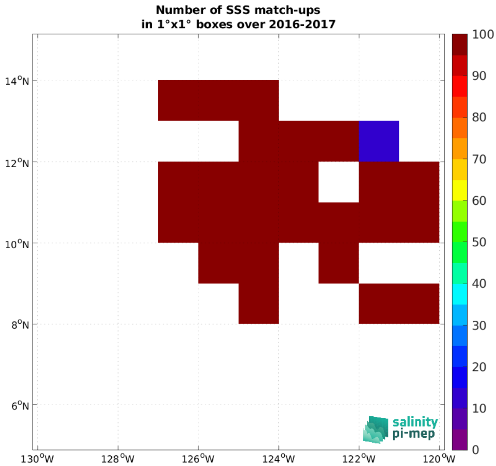
Figure 4: Number of SSS match-ups between Waveglider (SPURS 2) SSS and the SMAP SSS L4 OI v2 - 7 Days (ESR) SSS product for the SPURS 2 Pi-MEP region over 1^{\circ} \times 1^{\circ} boxes and for the full satellite product period.
