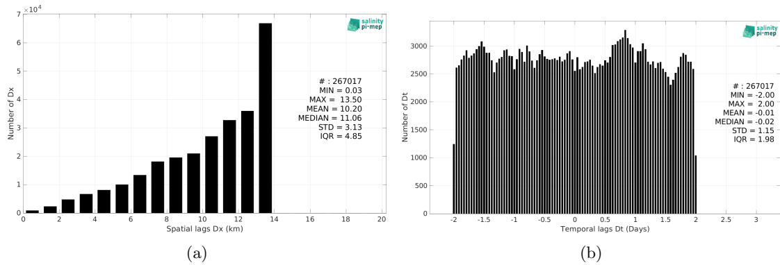
Figure 5: Histograms of the spatial (a) and temporal (b) lags between the location/time of the Waveglider (SPURS 2) measurement and the date of the corresponding SMAP SSS L4 OI v2 - 7 Days (ESR) SSS pixel.
