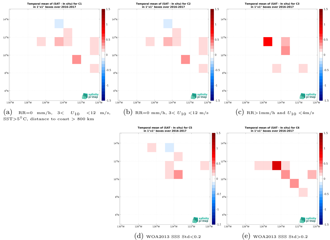
Figure 12: Temporal mean gridded over spatial boxes of size 1^\circ \times 1^\circ of \Delta SSS (SMAP SSS L4 OI v2 - 7 Days (ESR) - Waveglider (SPURS 2)) for 5 different subdatasets corresponding to:RR=0 mm/h, 3 < U_{10} < 12 m/s, SST >5^\circ\text{C} , distance to coast > 800 km (a), RR=0 mm/h, 3 < U_{10} < 12 m/s (b), RR >1 mm/h and U_{10} < 4 m/s (c), WOA2013 SSS Std <0.2 (d), WOA2013 SSS Std >0.2 (e).
