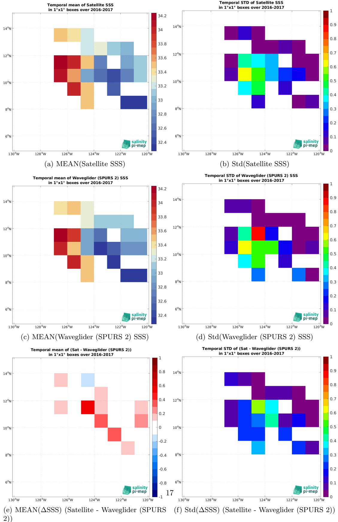
Figure 6: Temporal mean (left) and Std (right) of SSS from SMAP SSS L4 OI v2 - 7 Days (ESR) (top), Waveglider (SPURS 2) (middle), and of \Delta SSS (Satellite - Waveglider (SPURS 2)). Only match-up pairs are used to generate these maps.
