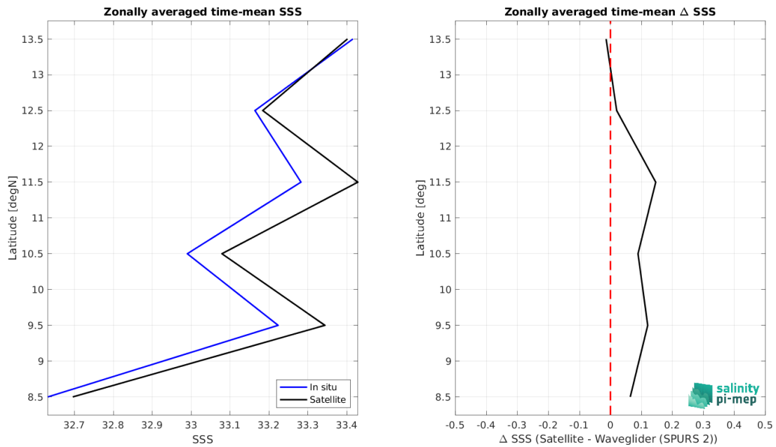
Figure 8: Left panel: Zonal mean SSS from SMAP SSS L4 OI v2 - 7 Days (ESR) satellite product (black) and from Waveglider (SPURS 2) (blue). Right panel: Zonal mean of \Delta SSS (Satellite - Waveglider (SPURS 2)) for all the collected Pi-MEP match-up pairs estimated over the full satellite product period.
