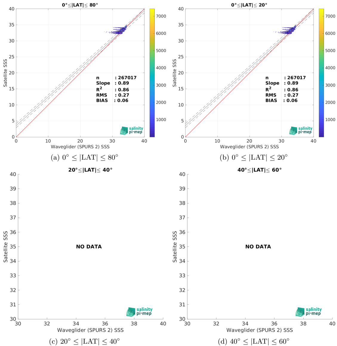
Figure 9: Contour maps of the concentration of SMAP SSS L4 OI v2 - 7 Days (ESR) SSS (y-axis) versus Waveglider (SPURS 2) SSS (x-axis) at match-up pairs for different latitude bands. For each plot, the red line shows x=y . The black thin and dashed lines indicate a linear fit through the data cloud and the \pm 95\% confidence levels, respectively. The number match-up pairs n , the slope and R^2 coefficient of the linear fit, the root mean square (RMS) and the mean bias between satellite and in situ data are indicated for each latitude band in each plots.
