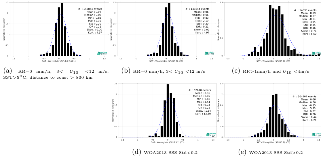
Figure 13: Normalized histogram of \Delta SSS (SMAP SSS L4 OI v2 - 7 Days (ESR) - Waveglider (SPURS 2)) for 5 different subdatasets corresponding to: RR=0 mm/h, 3 < U_{10} < 12 m/s, SST>5°C, distance to coast > 800 km (a), RR=0 mm/h, 3 < U_{10} < 12 m/s (b), RR>1mm/h and U_{10} < 4 m/s (c), WOA2013 SSS Std<0.2 (d), WOA2013 SSS Std>0.2 (e).
