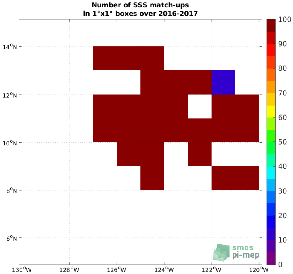
Figure 4: Number of SSS match-ups between Waveglider (SPURS 2) SSS and the SMAP SSS L4 OI v2 - 7 Days (ESR) SSS product for the SPURS 2 Pi-MEP region over 1°x1° boxes and for the full satellite product period.
