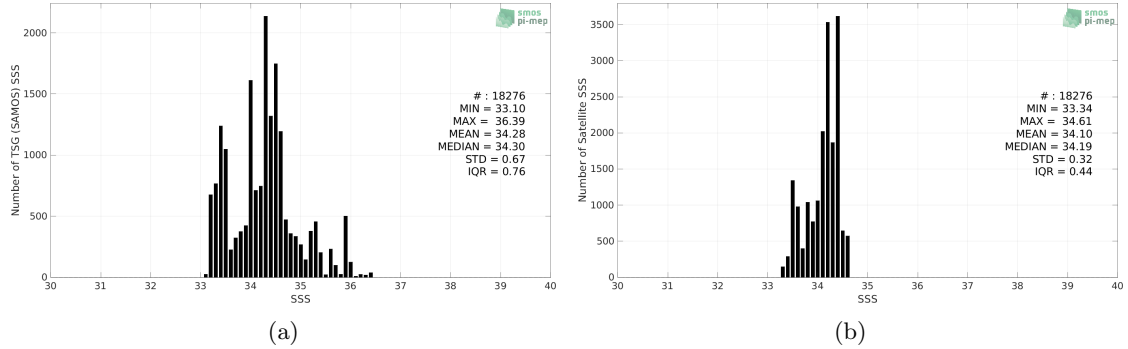
Figure 2: Histograms of SSS from TSG (SAMOS) (a) and SMAP SSS L4 OI v2 - 7 Days (ESR) (b) considering all match-up pairs per bins of 0.1 over the SPURS 2 Pi-MEP region and for the full satellite product period.
