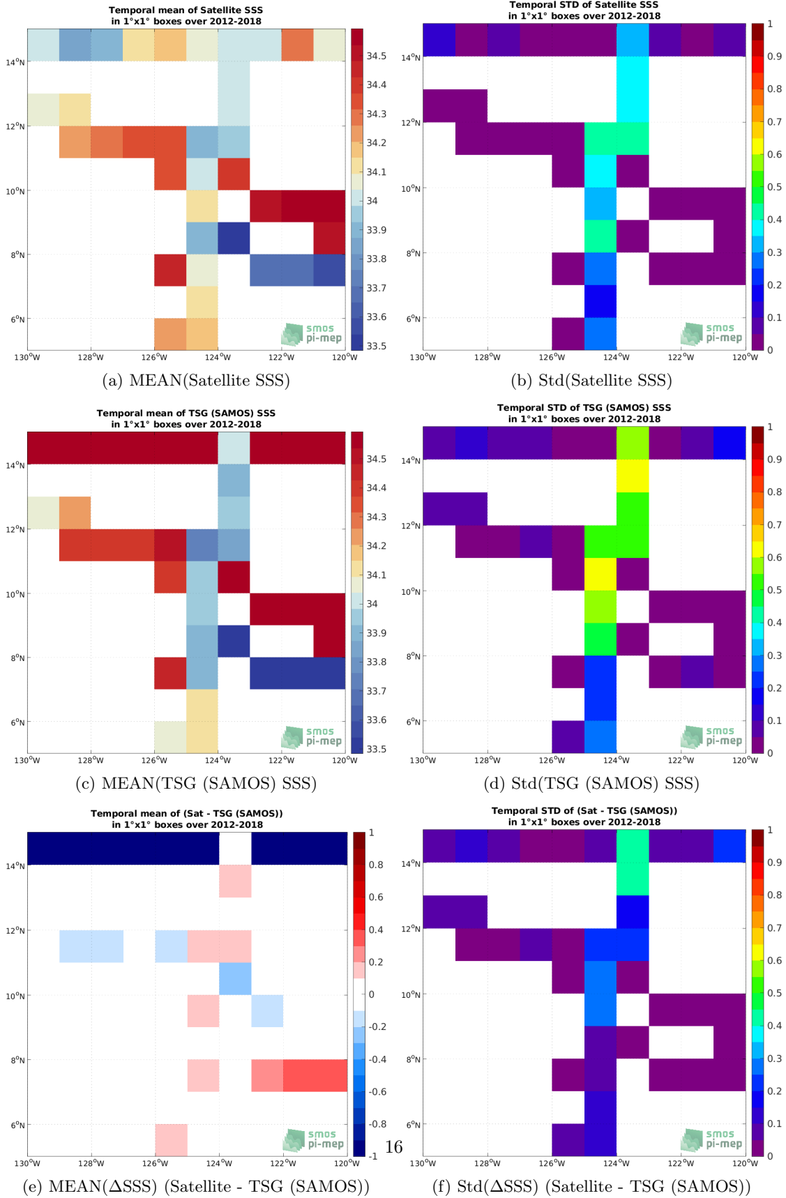
Figure 6: Temporal mean (left) and Std (right) of SSS from SMAP SSS L4 OI v2 - 7 Days (ESR) (top), TSG (SAMOS) (middle), and of \Delta SSS (Satellite - TSG (SAMOS)). Only match-up pairs are used to generate these maps.
