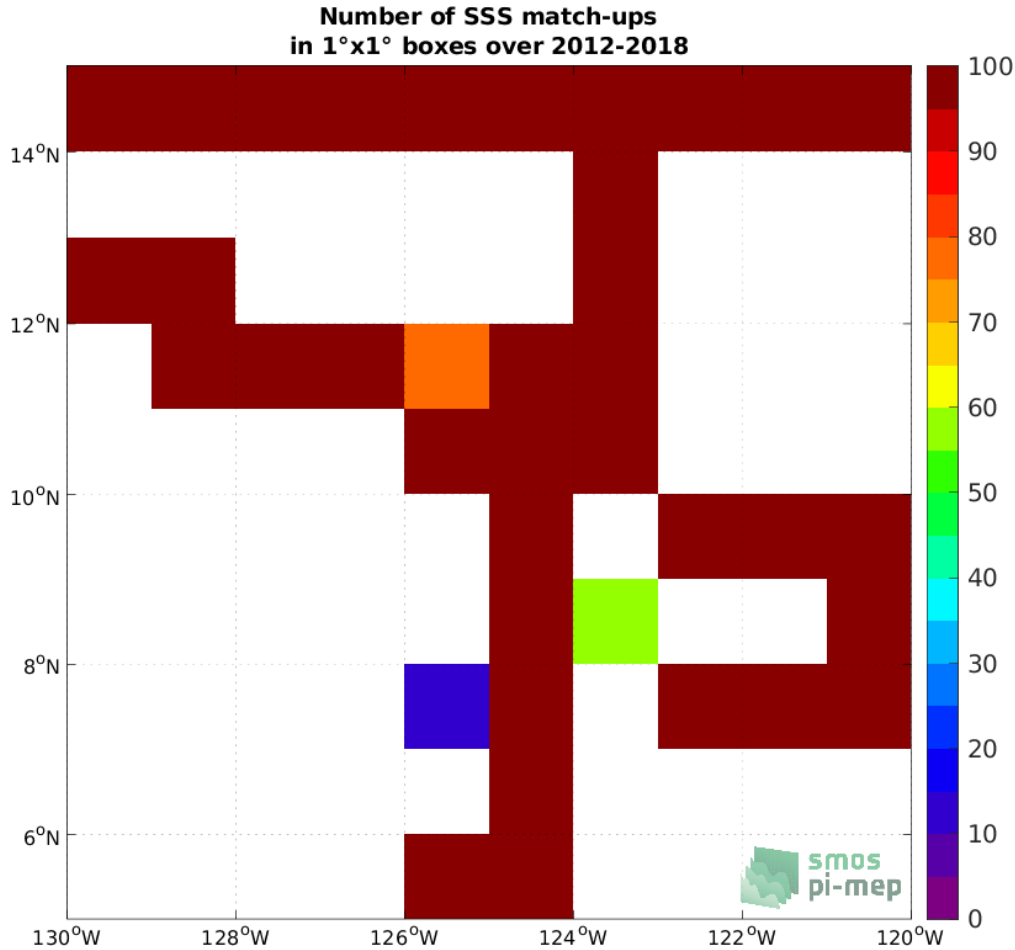
Figure 4: Number of SSS match-ups between TSG (SAMOS) SSS and the SMAP SSS L4 OI v2 - 7 Days (ESR) SSS product for the SPURS 2 Pi-MEP region over 1^\circ \times 1^\circ boxes and for the full satellite product period.
